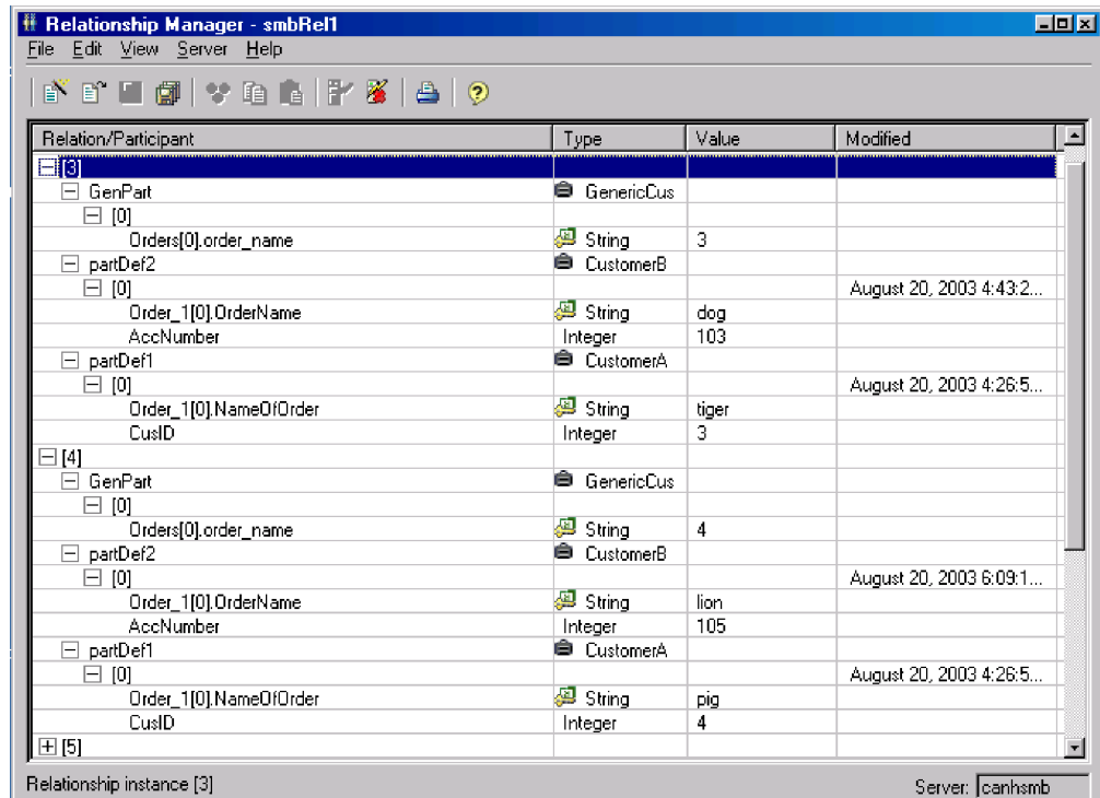
Figure 37. Relationship Manager, arborescence de relation
