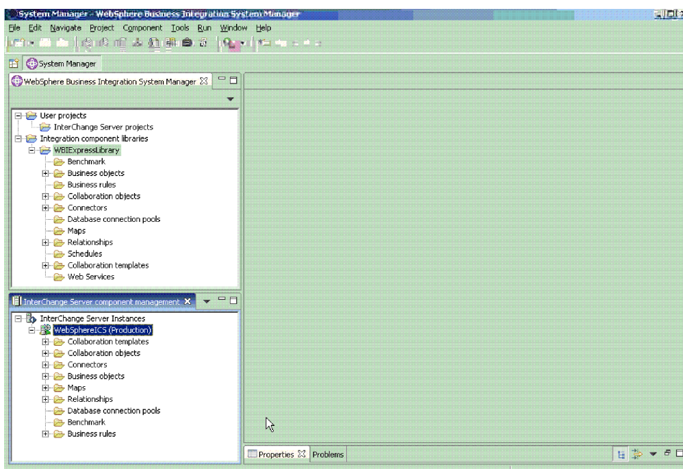
Figure 25. System Manager
