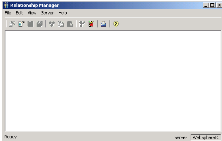
Figure 38. Relationship Manager
