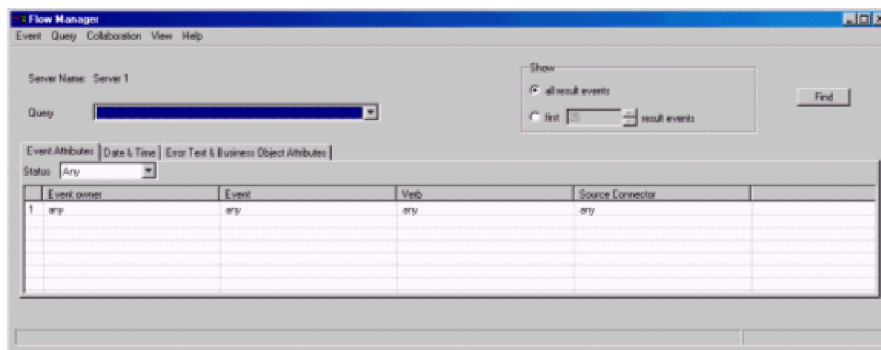
Figure 69. Flow Manager
