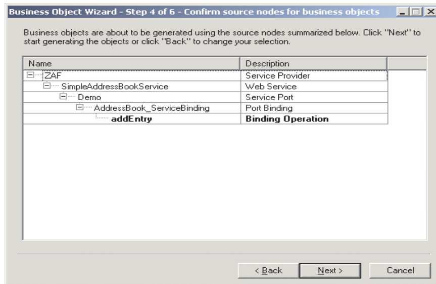
Figure 65. Confirm window
