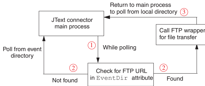
Figure 6. Local and remote event notification operation
