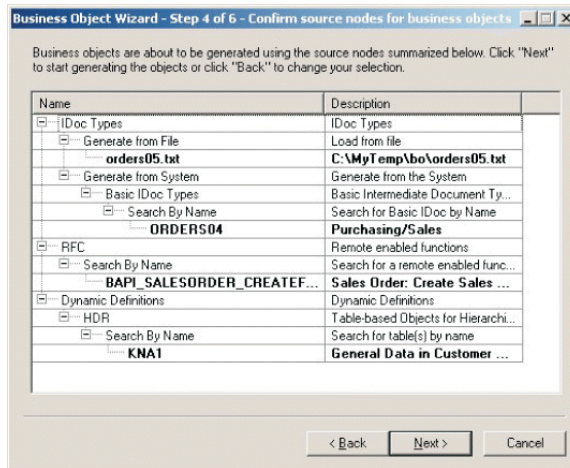
Figure 42. Confirming selection of nodes and leaves
