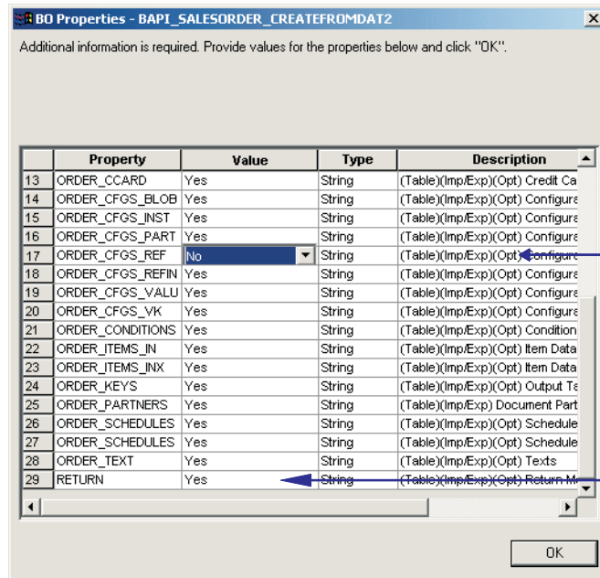
Figure 48. Specifying attributes for removal from the definition
