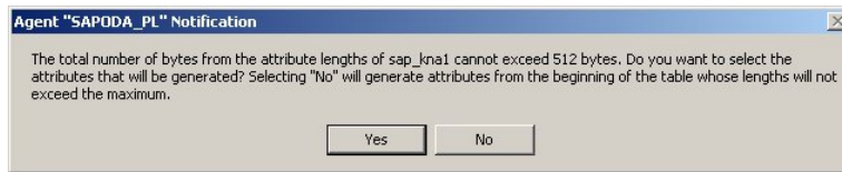
Figure 50. 512 byte warning
