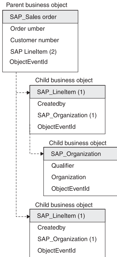
Figure 14. Hierarchical business object SAP sales order (IDoc)
