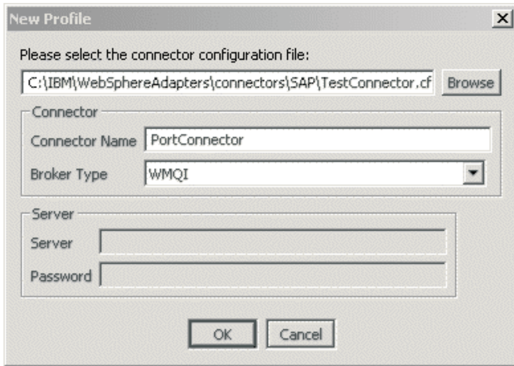
Figure 37. Test Connector—New Profile
