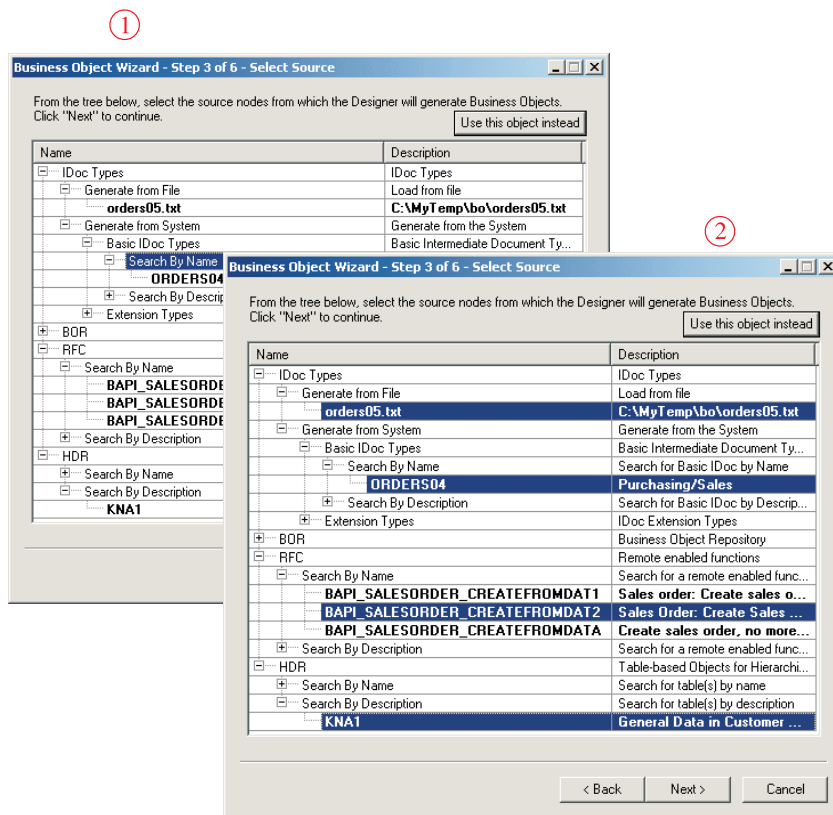
Figure 40. Tree with expanded nodes
