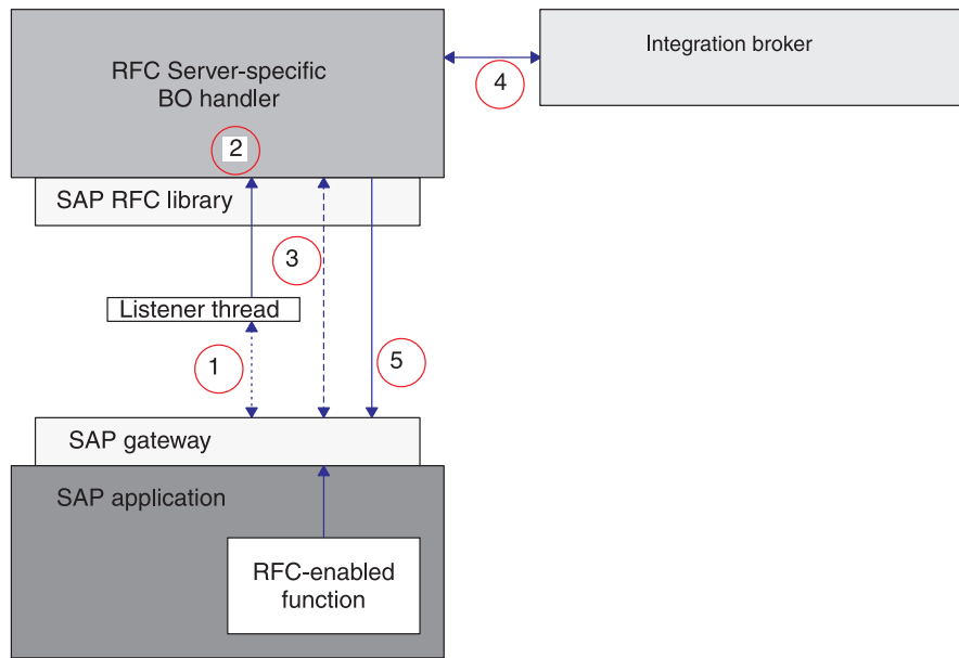
Figure 26. Business object processing
