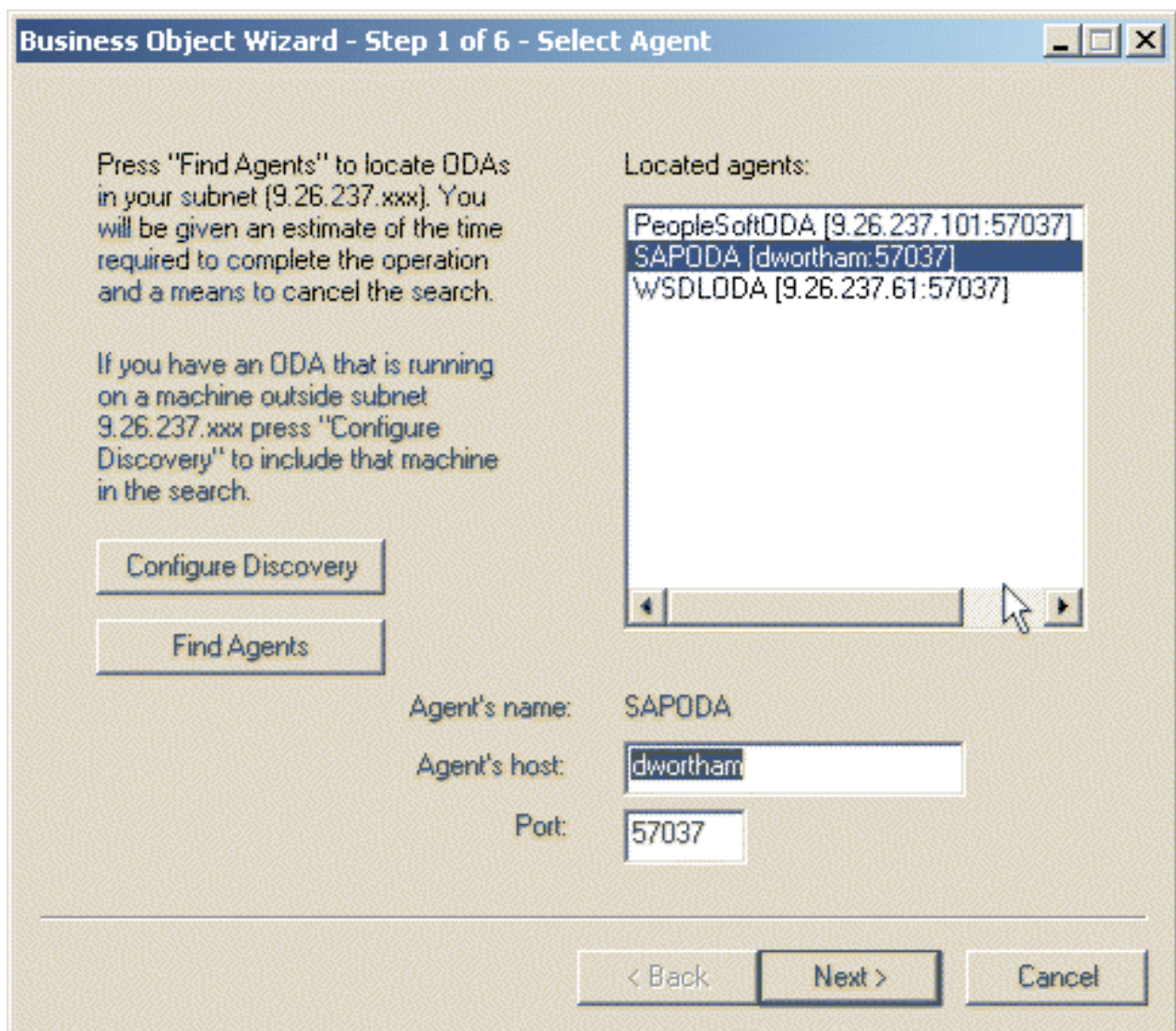
Figure 34. Business Object Wizard—Select Agent
