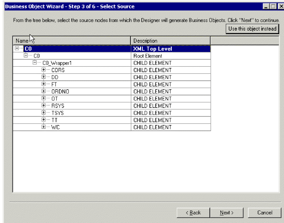
Figure 40. Tree of XML elements with expanded nodes
