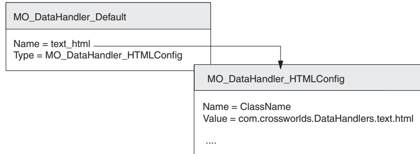
Figure 37. Example top-level connector meta-object for a custom data handler
