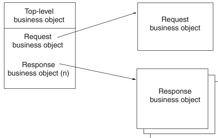
Figure 31. Business object structure for a request-response business object
