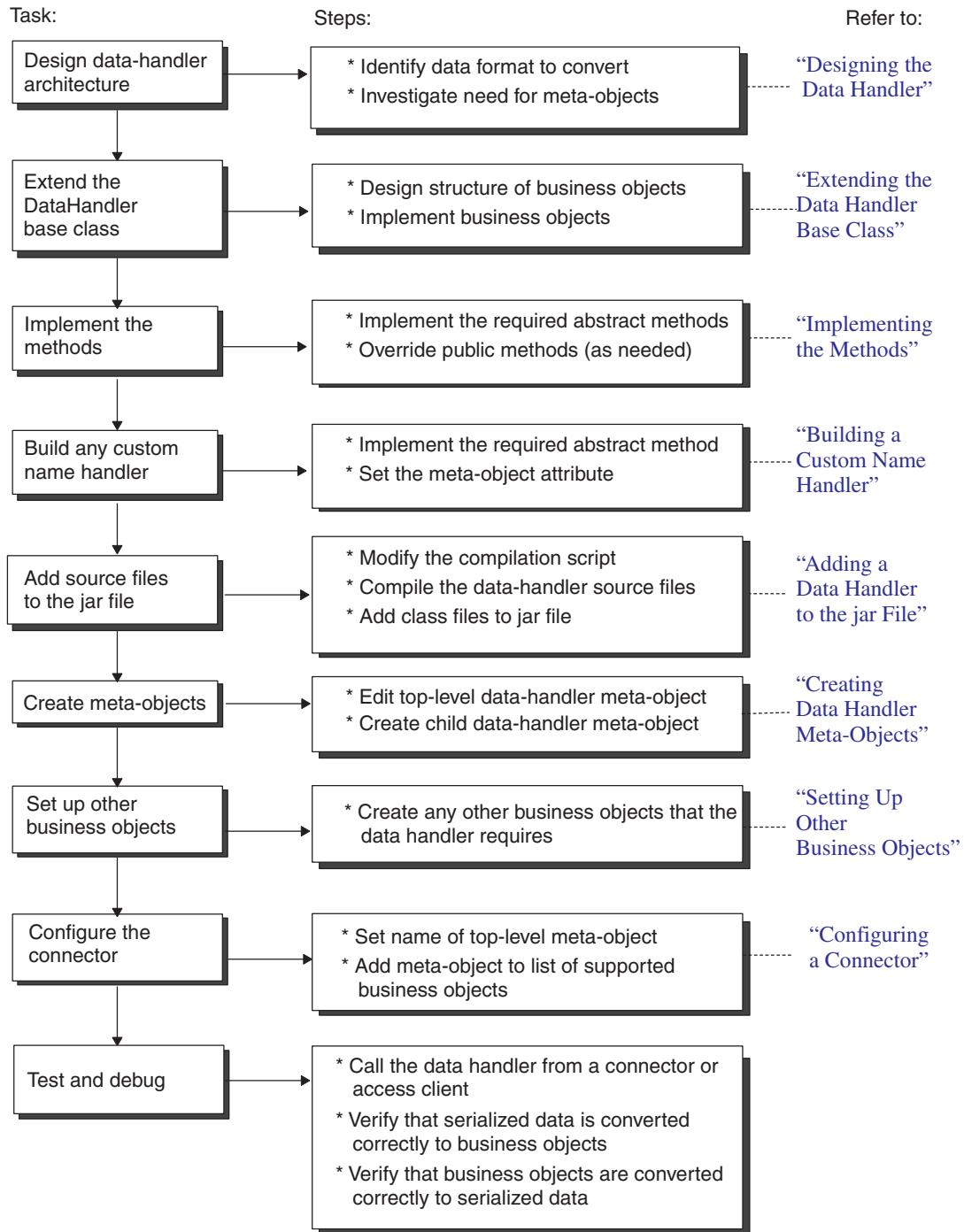
Figure 33. Overview of the data-handler development process
