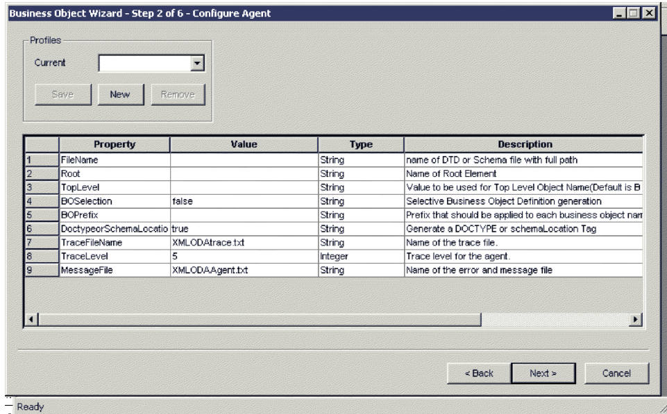
Figure 39. Specifying ODA configuration properties
