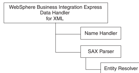
Figure 11. XML data handler components
