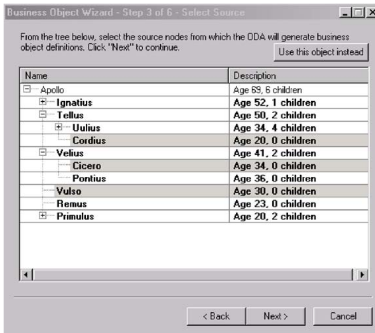
Figure 39. Select Source dialog box with source nodes expanded and selected
