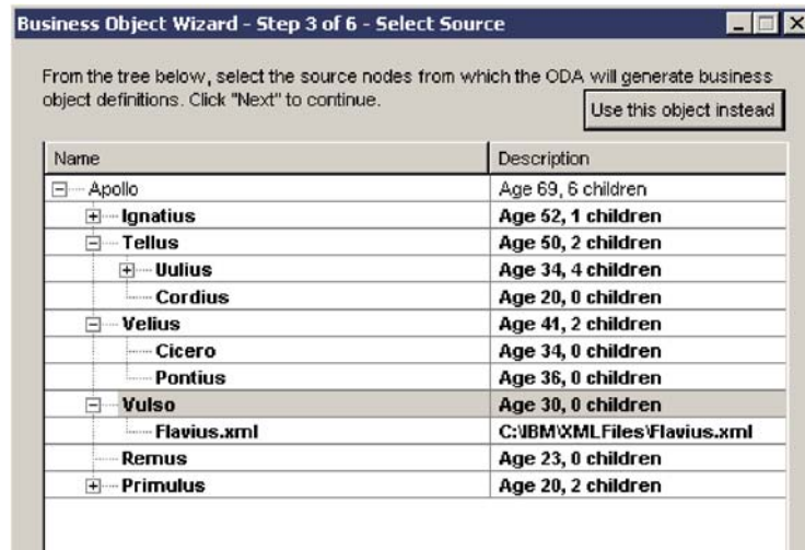
Figure 50. File associated with a source node
