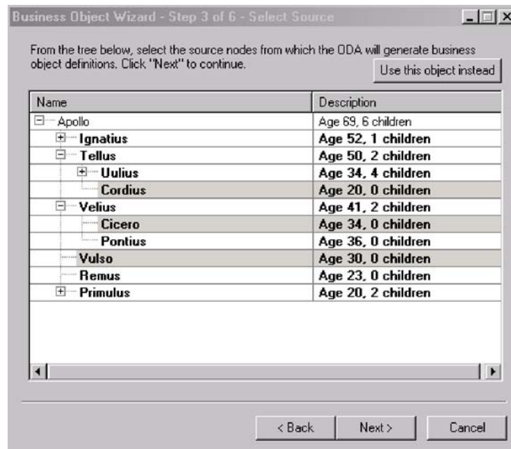
Figure 38. Initial Select Source dialog box
