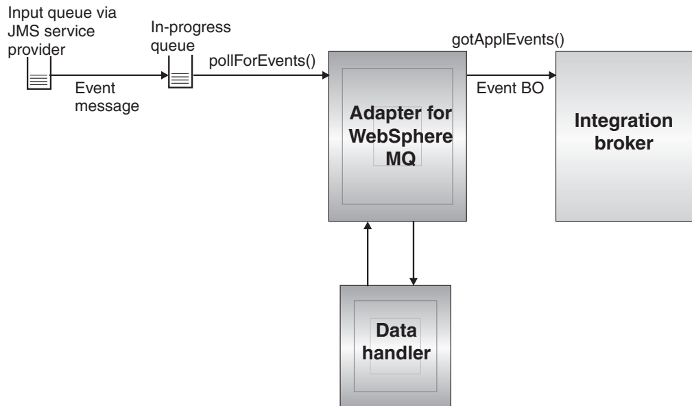
Figure 2. Application-connector communication method: Event delivery
