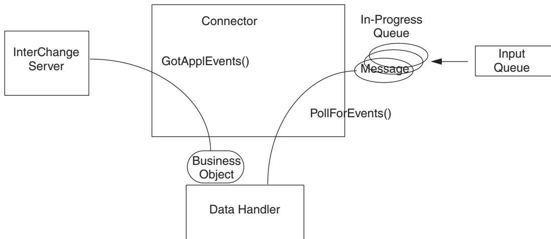
Figure 3. Application-adapter communication method: Message return
