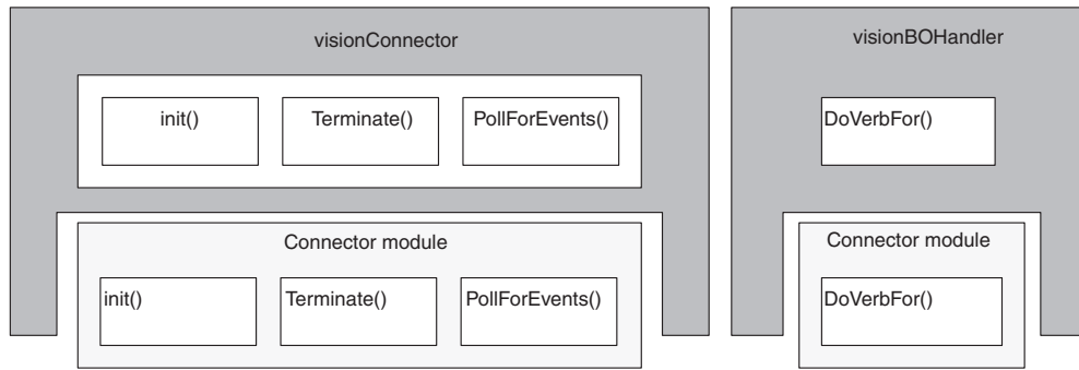
Figure 3. Vision connector framework and connector modules
