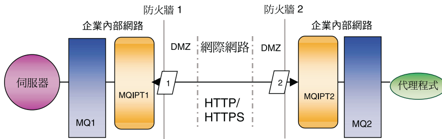
圖 3. HTTP/HTTPS 配置
