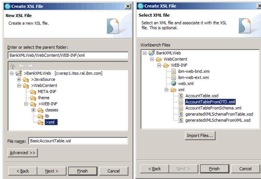
Figure 10-35 The create new XSL wizard
