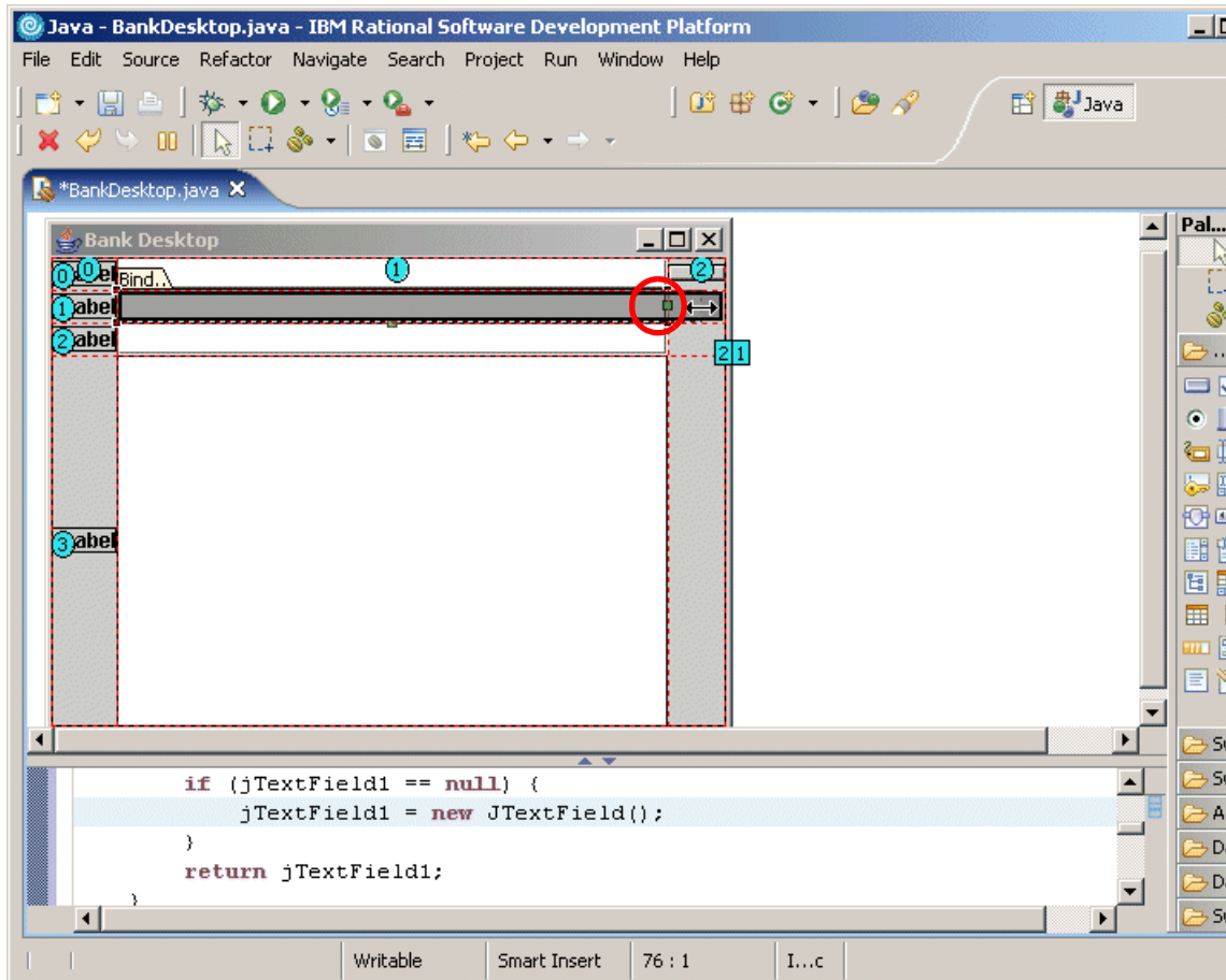
Figure 9-10 Resizing components within the layout
