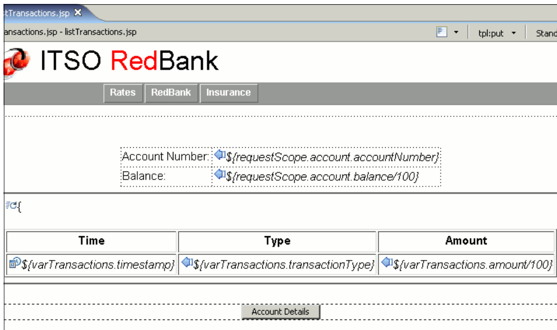
Figure 11-44 Completed listTransactions.jsp in the Design view
