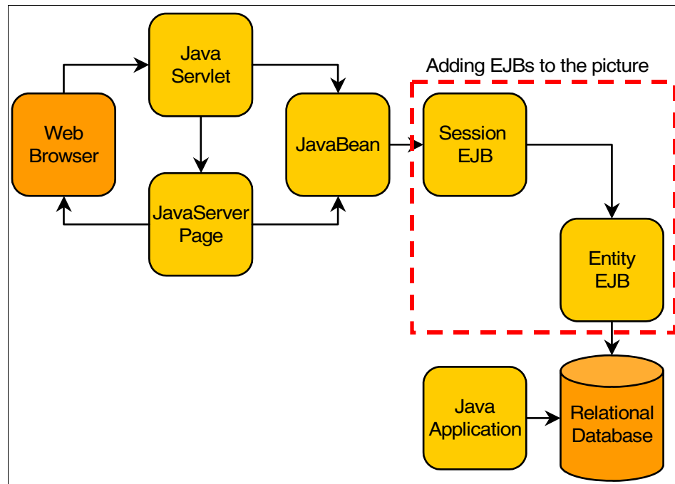
Figure 2-4 EJBs as part of an enterprise application
