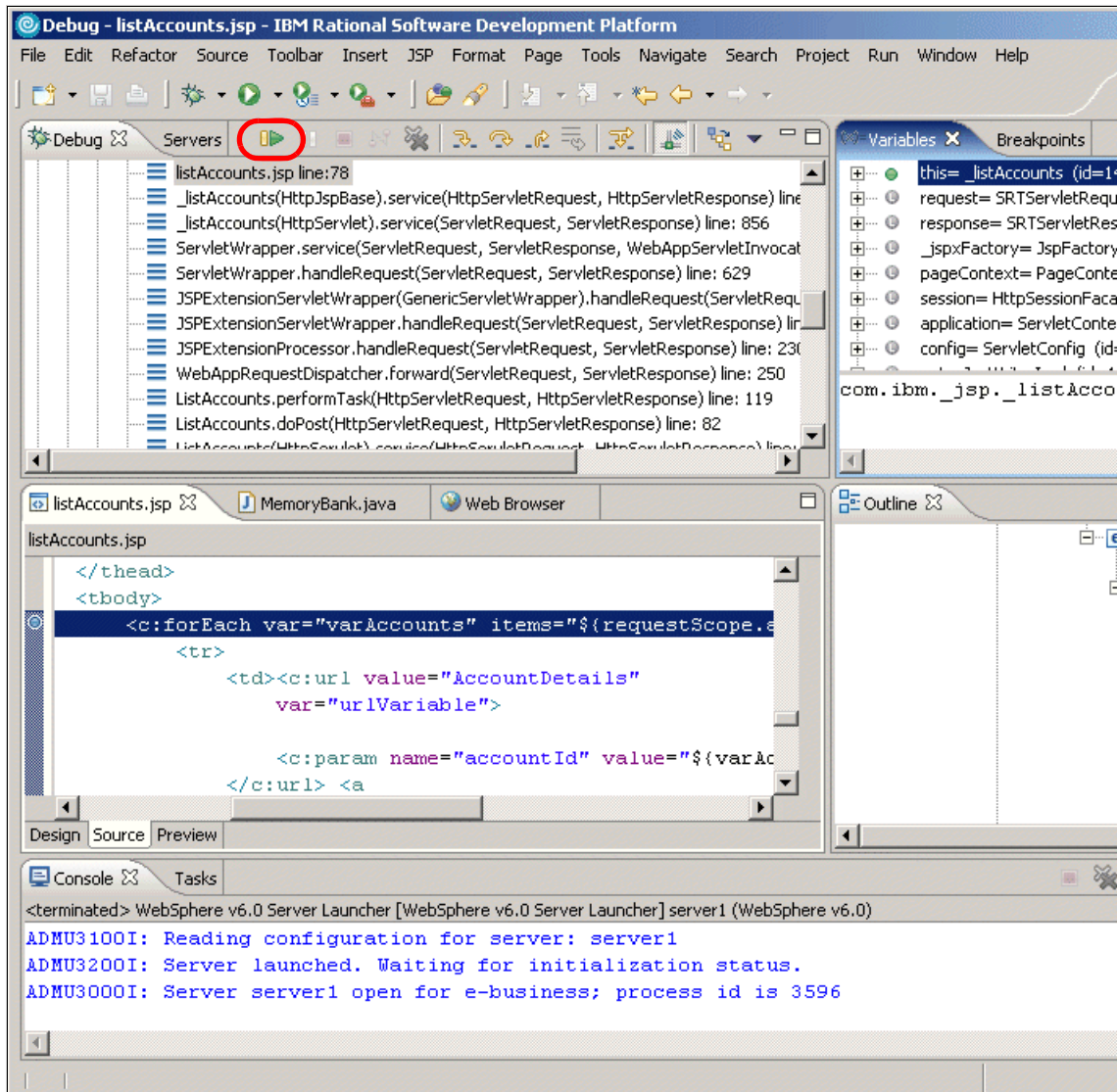
Figure 21-12 Breakpoint in listAccounts.jsp in the Debug perspective
