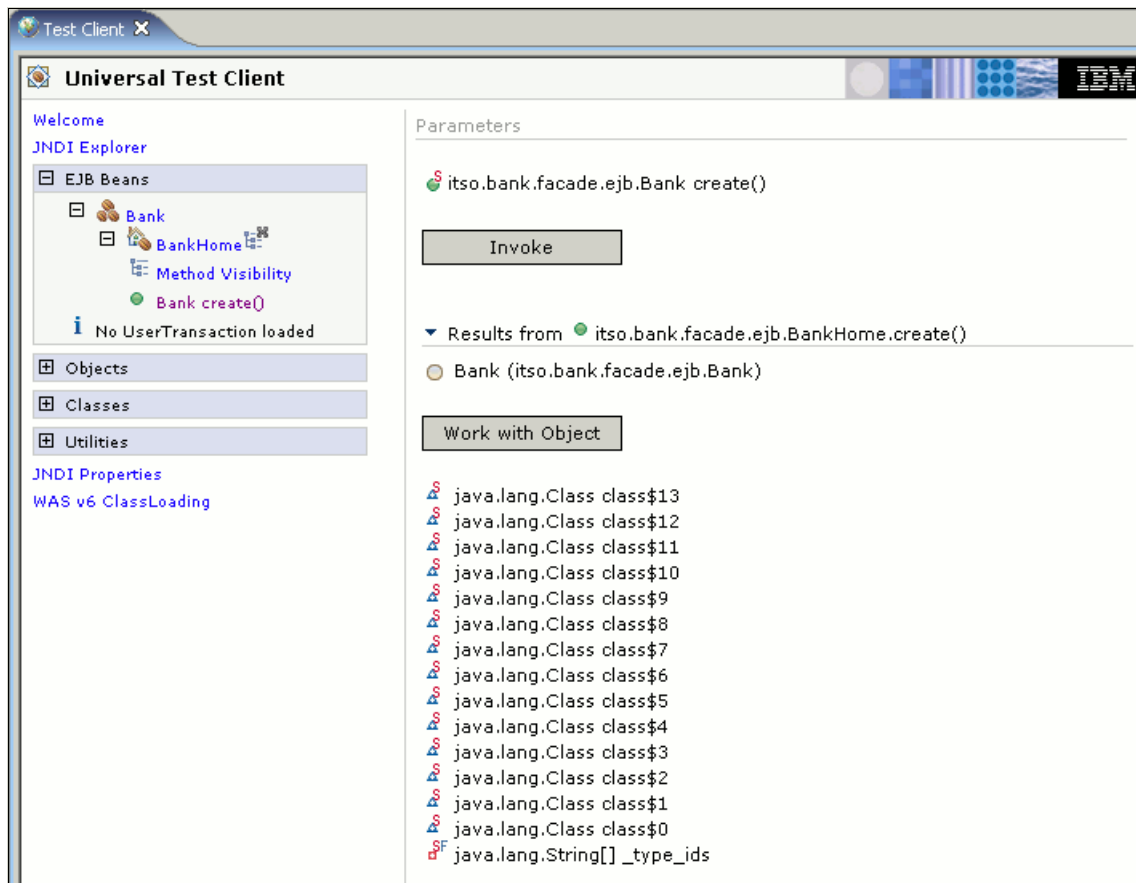
Figure 15-50 After invoking the create method for the Bank EJB
