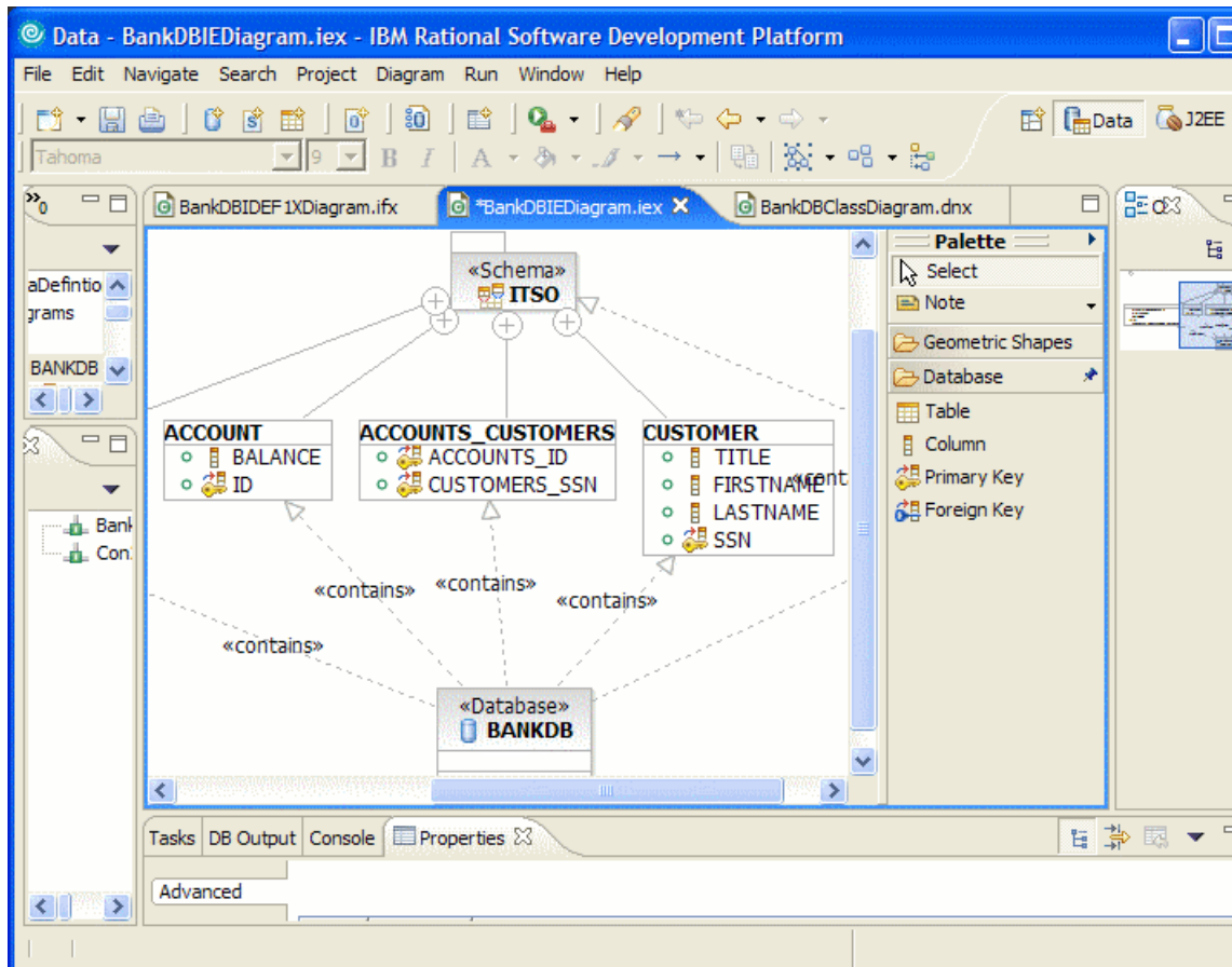
Figure 8-30 UML visualization - IE diagram
