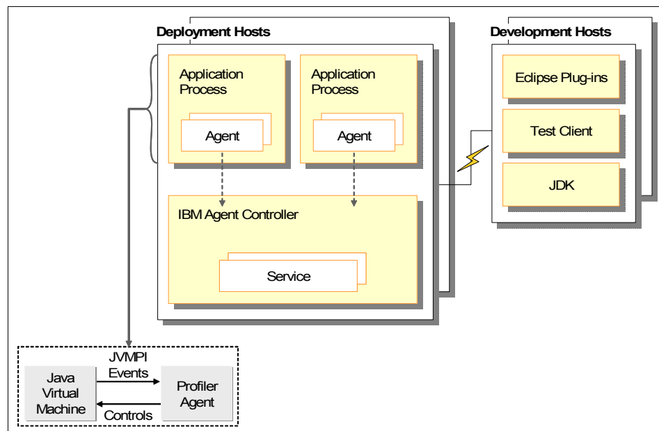
Figure 24-1 Profiling architecture of IBM Rational Application Developer V6.0
