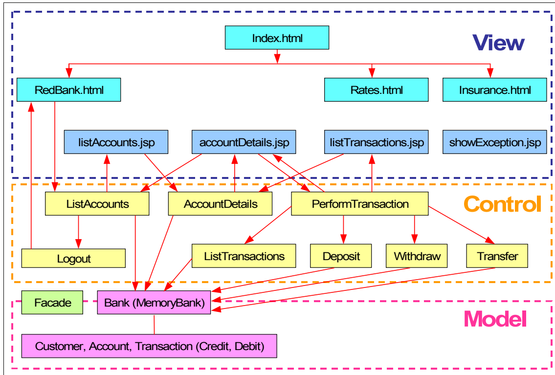
Figure 11-9 ITSO RedBank application flow
