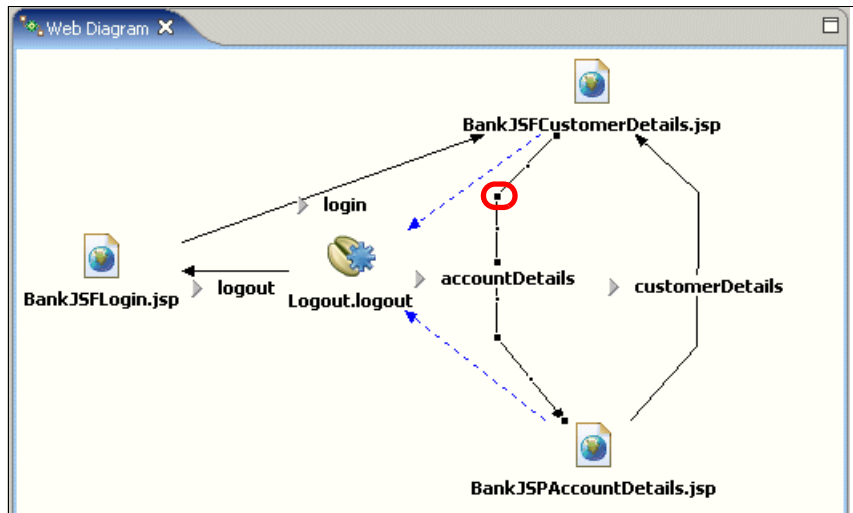
Figure 13-38 Completed Web diagram
