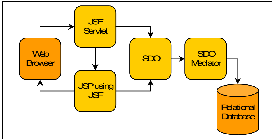
Figure 2-2 JSF and SDO
