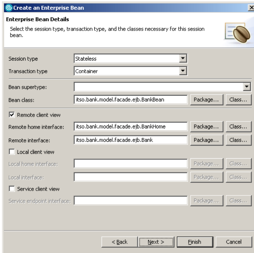
Figure 15-44 Creating a new session bean (page 2)
