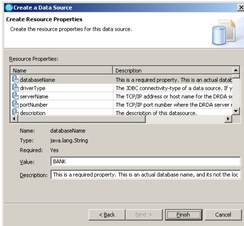
Figure 19-19 Create a Data Source (page 3)
