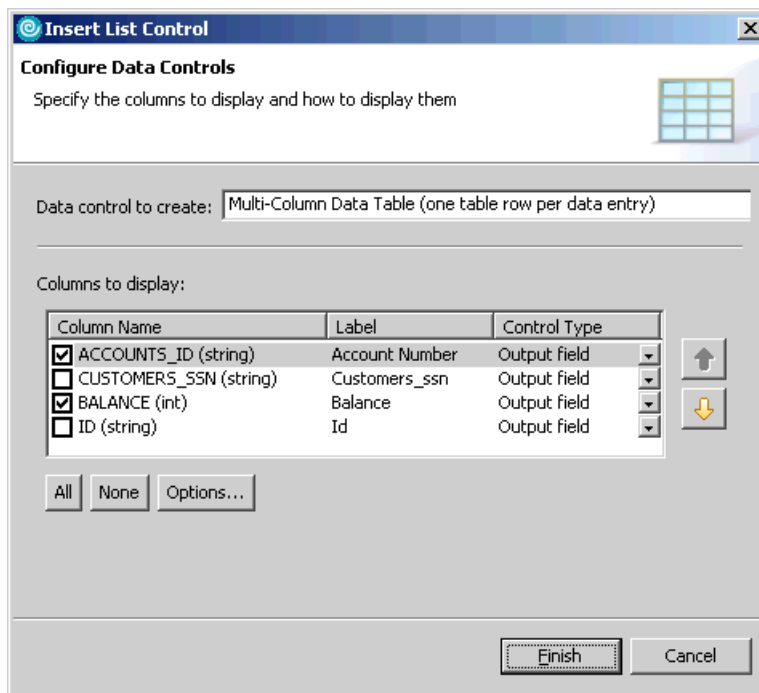
Figure 14-28 Configure Data Controls
