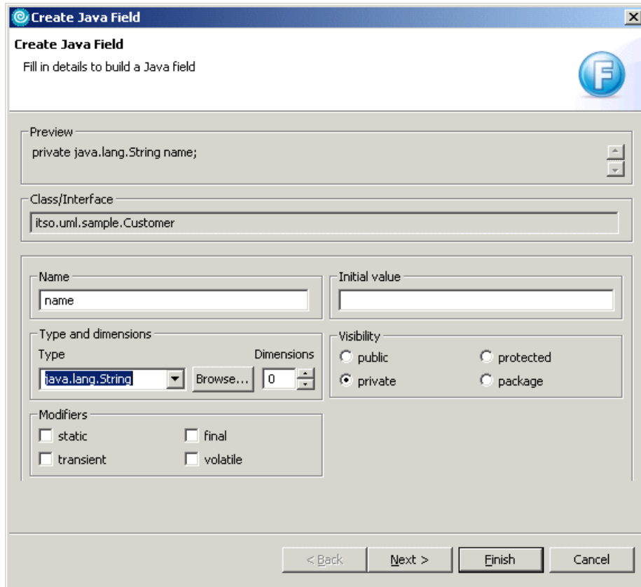
Figure 6-15 Adding a new field to Customer class
