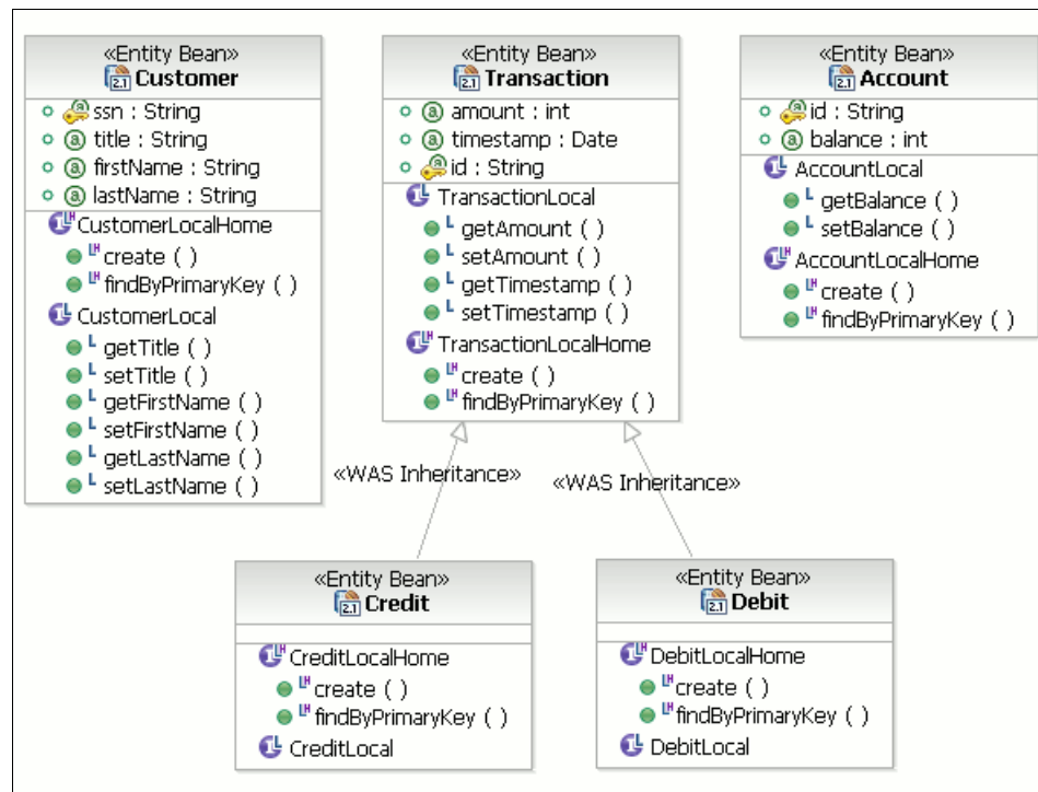
Figure 15-23 Class diagram at entity bean creation phase
