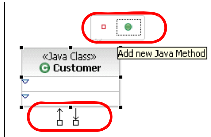
Figure 6-14 Shape action bar
