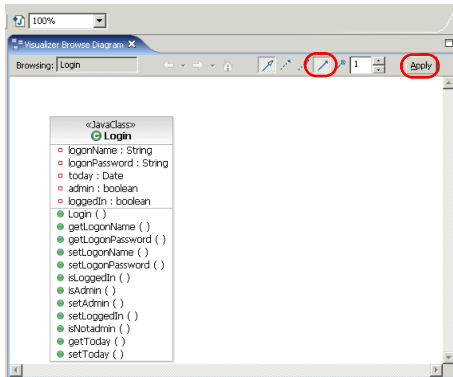
Figure 6-5 Visualizer Browse Diagram - Login.java
