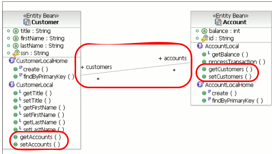
Figure 15-27 Finished customer account relationship
