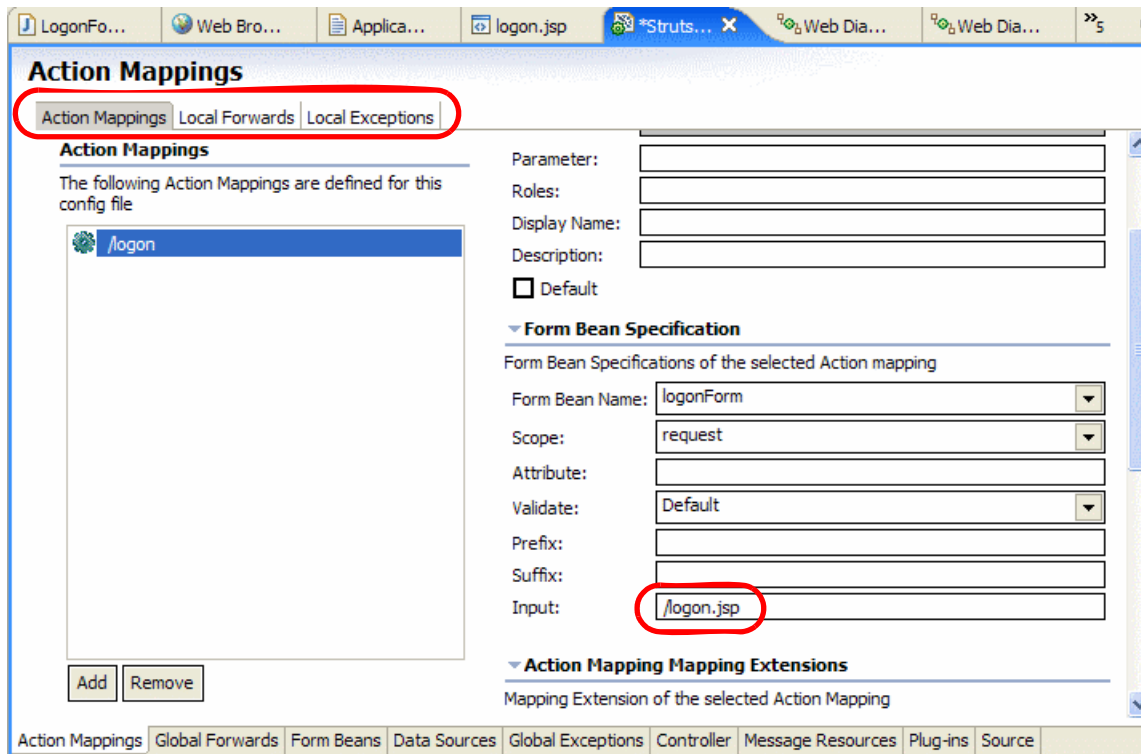
Figure 12-31 Struts Configuration Editor - Action input attribute
