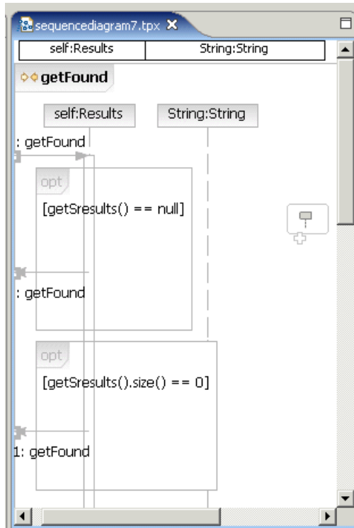
Figure 6-11 Static method sequence diagram with option fragments
