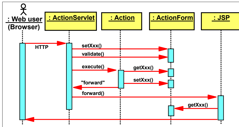
Figure 12-2 Struts request sequence
