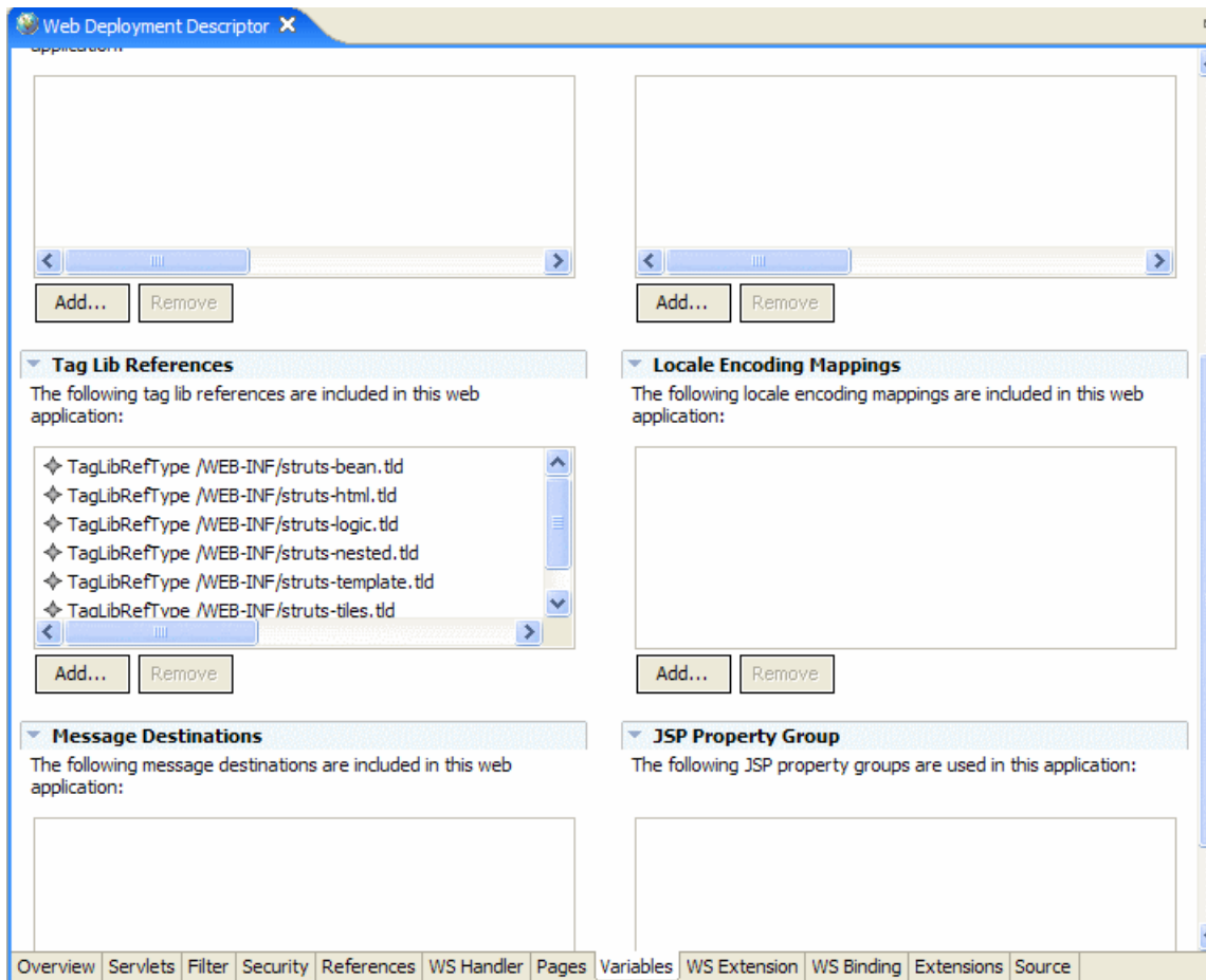
Figure 12-8 Generated Web Deployment Descriptor config for Struts tag library references
