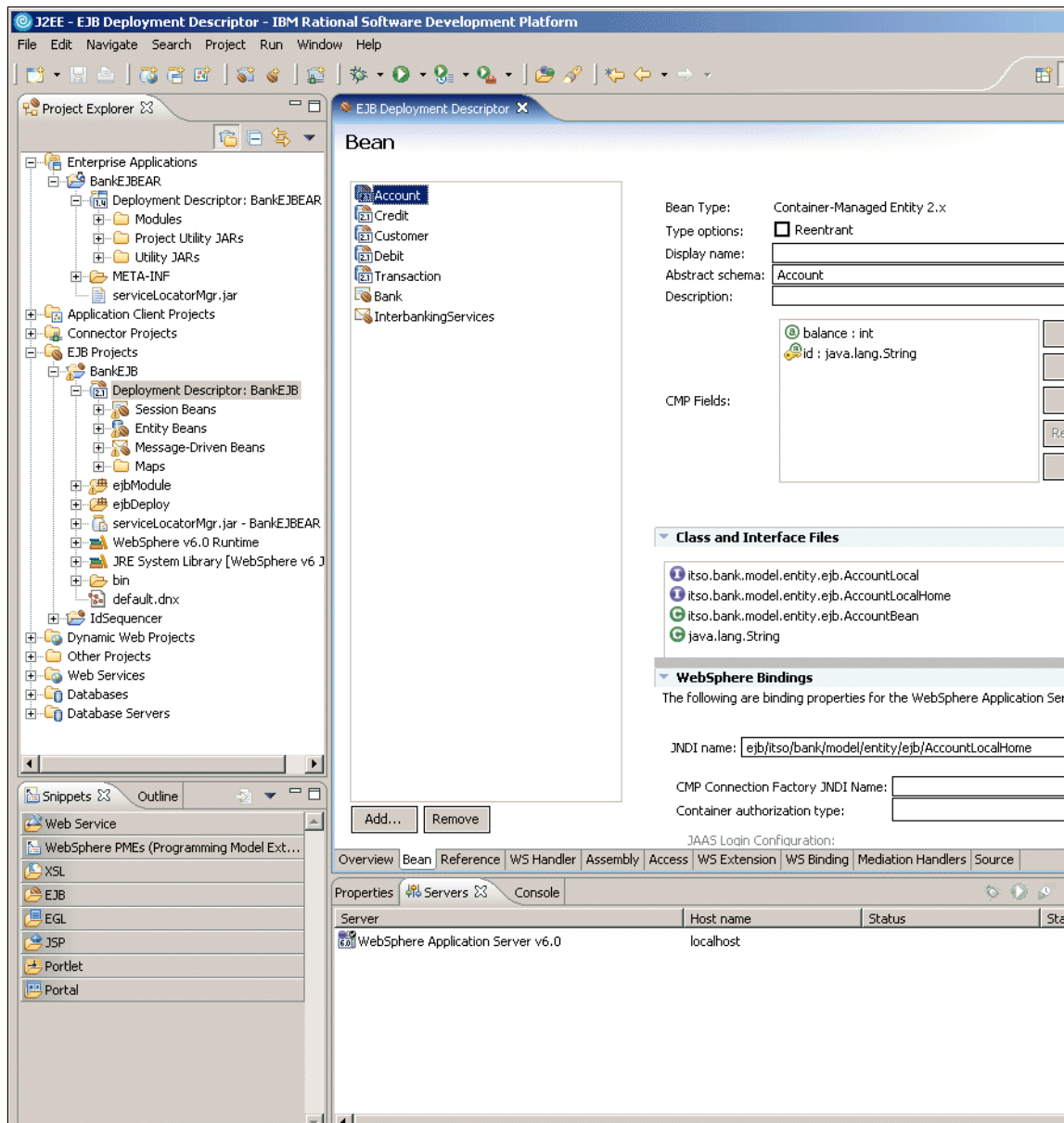
Figure 23-4 Deployment Descriptor Editor in Rational Application Developer
