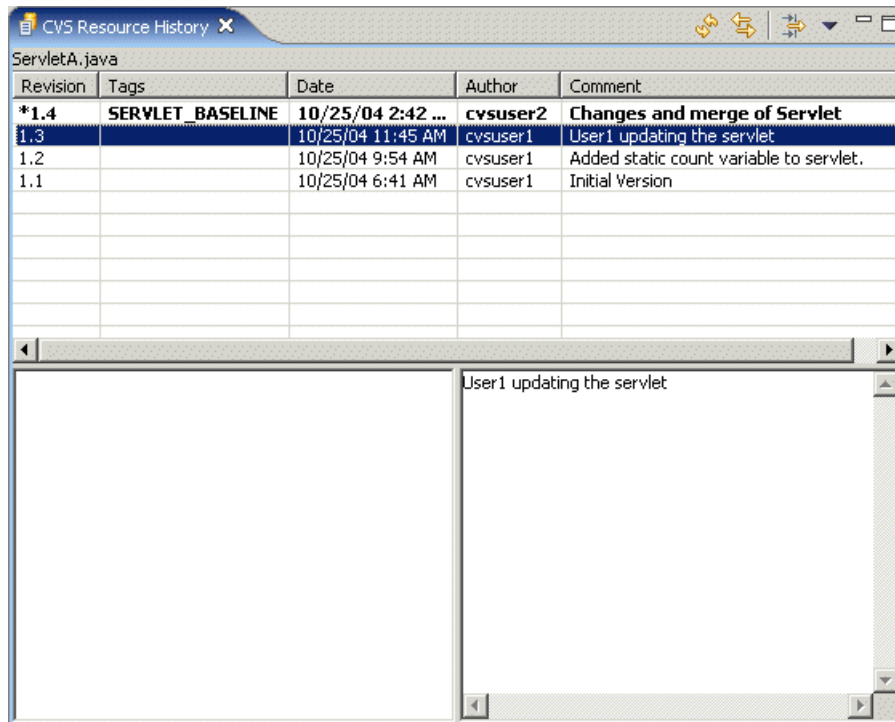
Figure 26-37 CVS Resource view for ServletA.java
