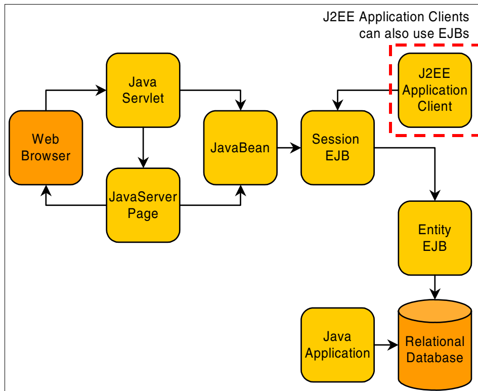
Figure 2-5 J2EE Application Clients
