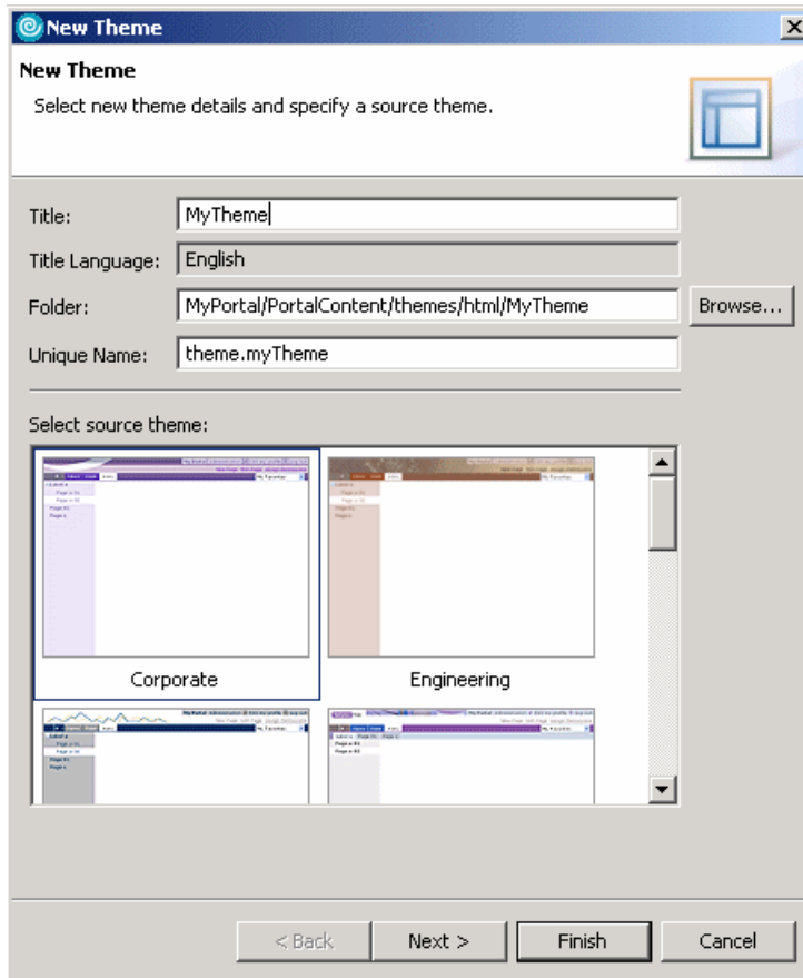
Figure 18-8 New Theme wizard
