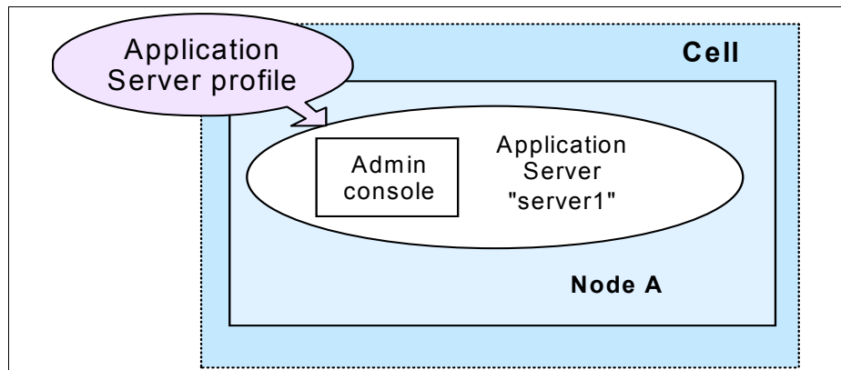
Figure 19-1 System management topology - Standalone server (Base and Express)
