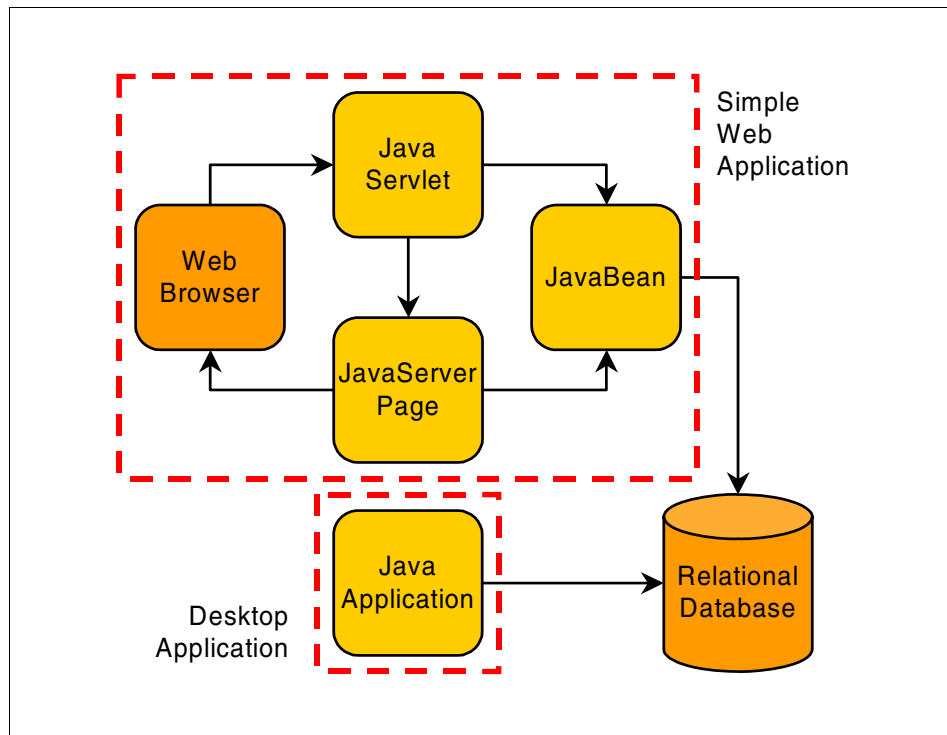
Figure 2-1 Simple Web application
