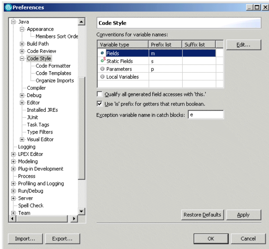
Figure 3-22 Completed code style definition preferences
