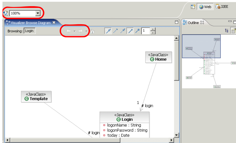
Figure 6-6 Visualizer Browse diagram and the Outline view
