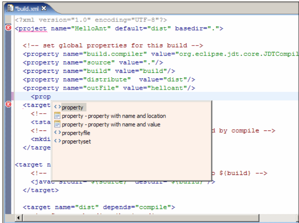
Figure 22-1 Code Assist in Ant editor
