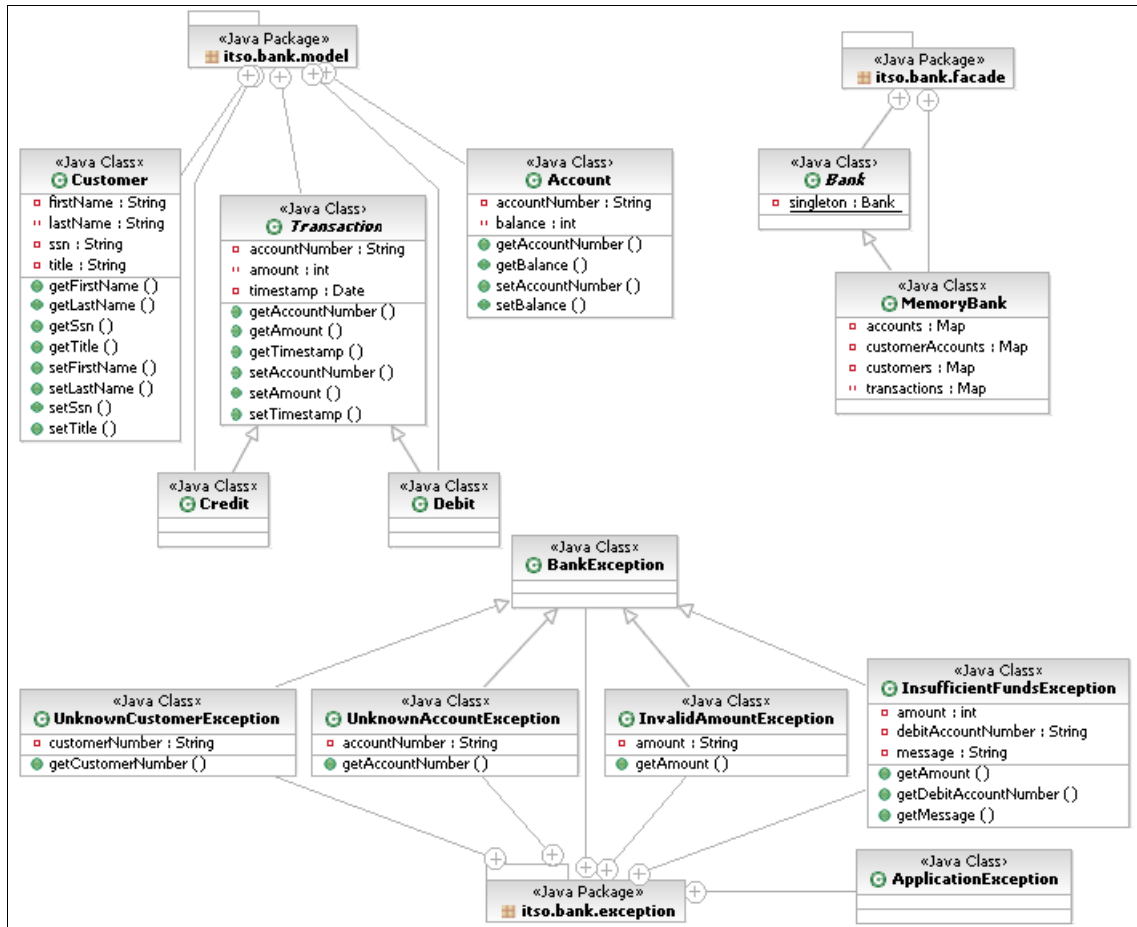
Figure 11-34 Class diagram with fields and accessors
