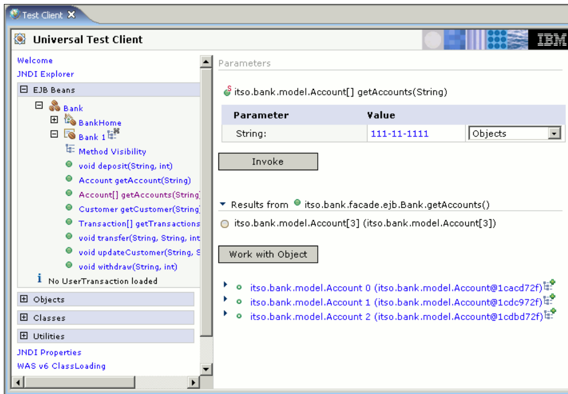
Figure 15-51 After invoking getAccounts for customer 111-11-1111
