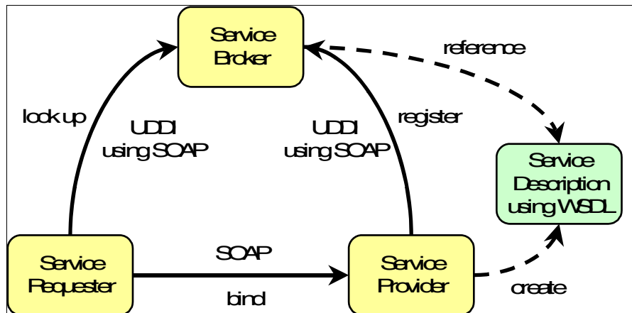
Figure 17-2 Web Services implementation of an SOA
