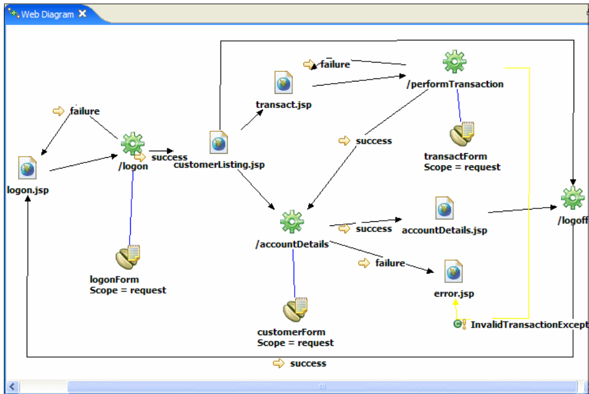
Figure 12-3 Struts Web diagram - Bank sample
