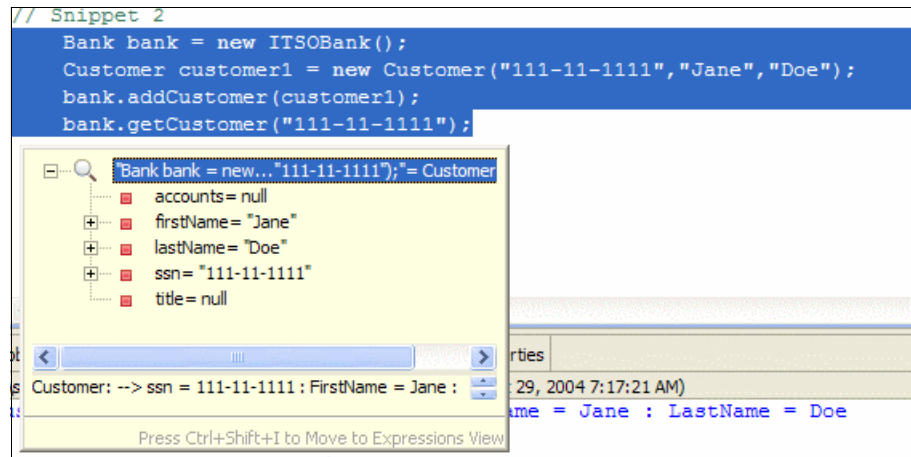
Figure 7-41 Java Scrapbook - Display results
