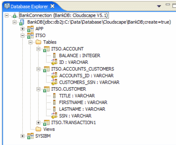
Figure 8-5 Data perspective - Database Explorer view
