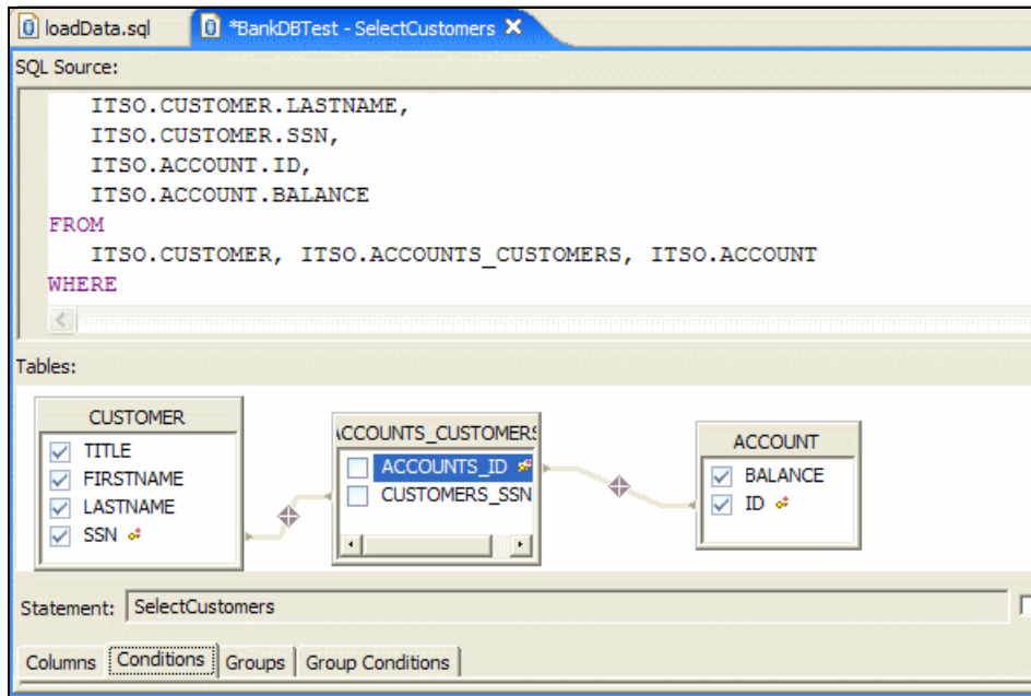
Figure 8-41 SQL Query Builder - Creating joins
