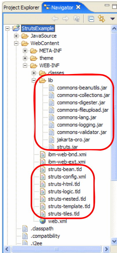
Figure 12-6 Generated struts-config.xml, Struts jars, and tag library definitions
