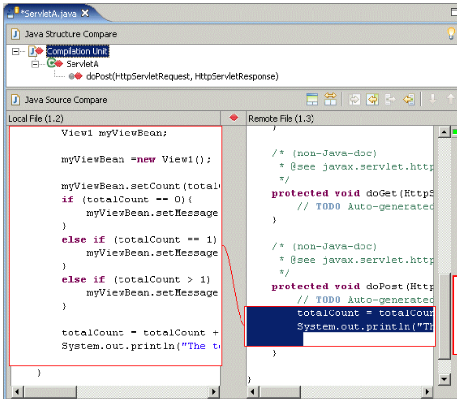
Figure 26-32 Merging changes from right to left
