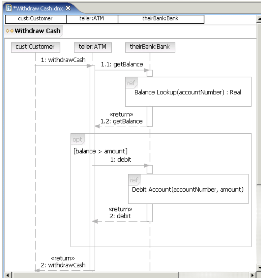
Figure 6-21 Completed sequence diagram: Withdraw Cash
