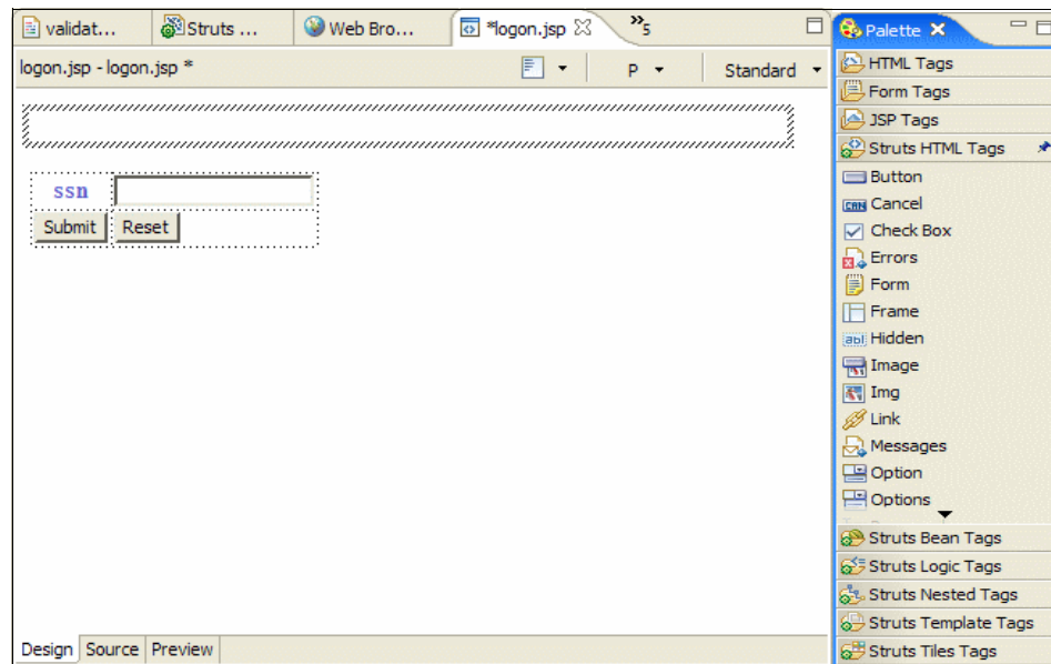
Figure 12-28 Struts tags - Adding a Struts tag
