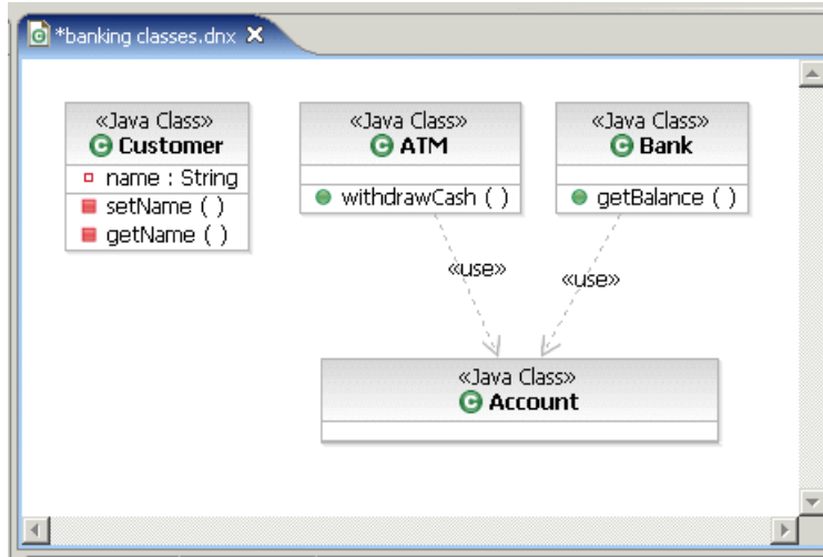
Figure 6-16 Completed class diagram
