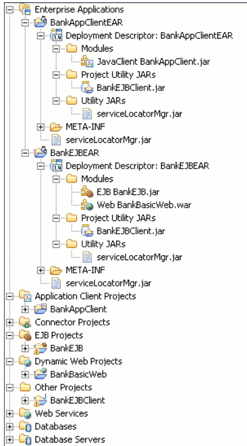
Figure 16-4 Project Explorer for the finished application client
