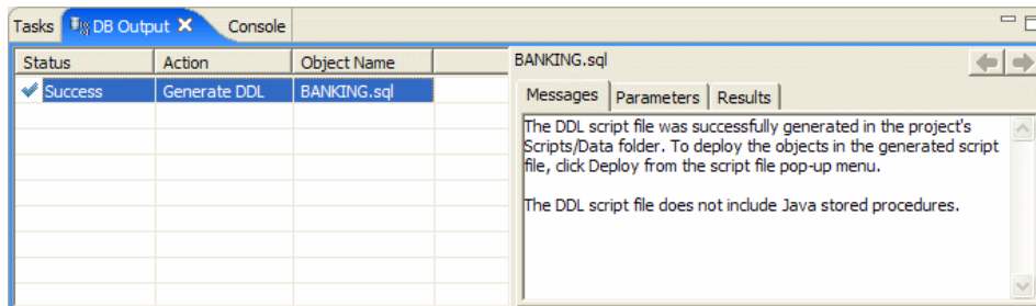
Figure 8-6 Data perspective - Database Output view
