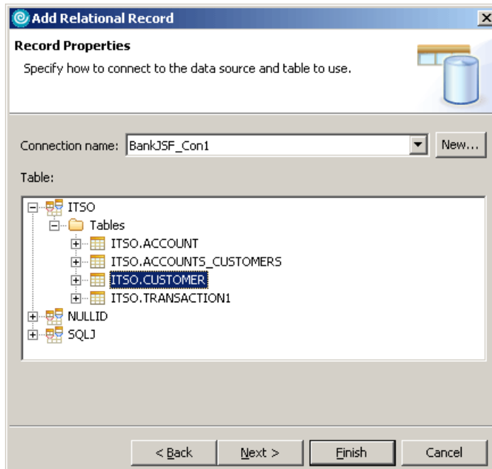
Figure 13-56 Selecting the table for the Relational Record
