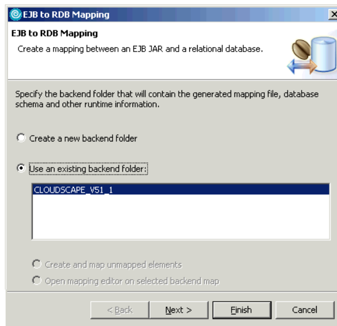
Figure 15-36 Using an existing backend folder
