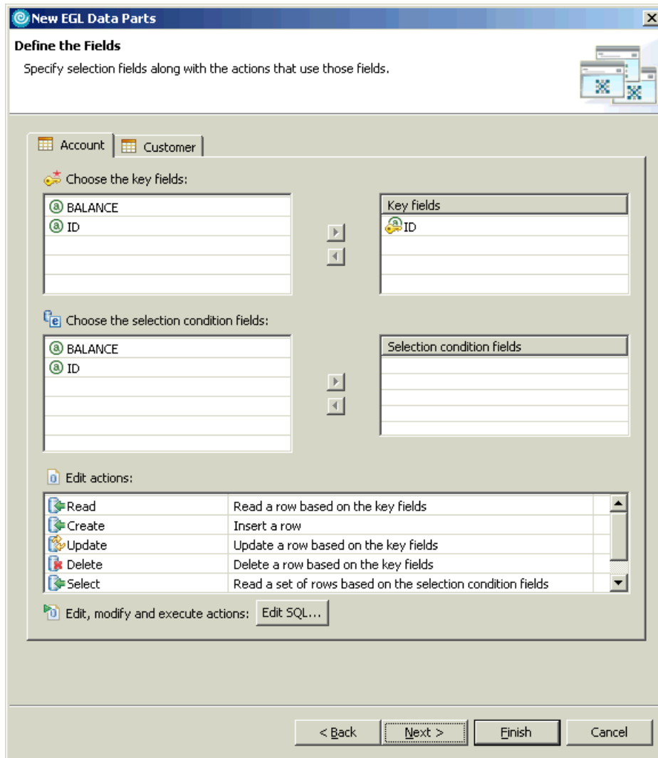
Figure 14-15 New EGL Data Parts - Define the Fields
