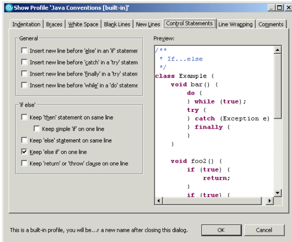
Figure 3-29 Code formatting - Control Statements
