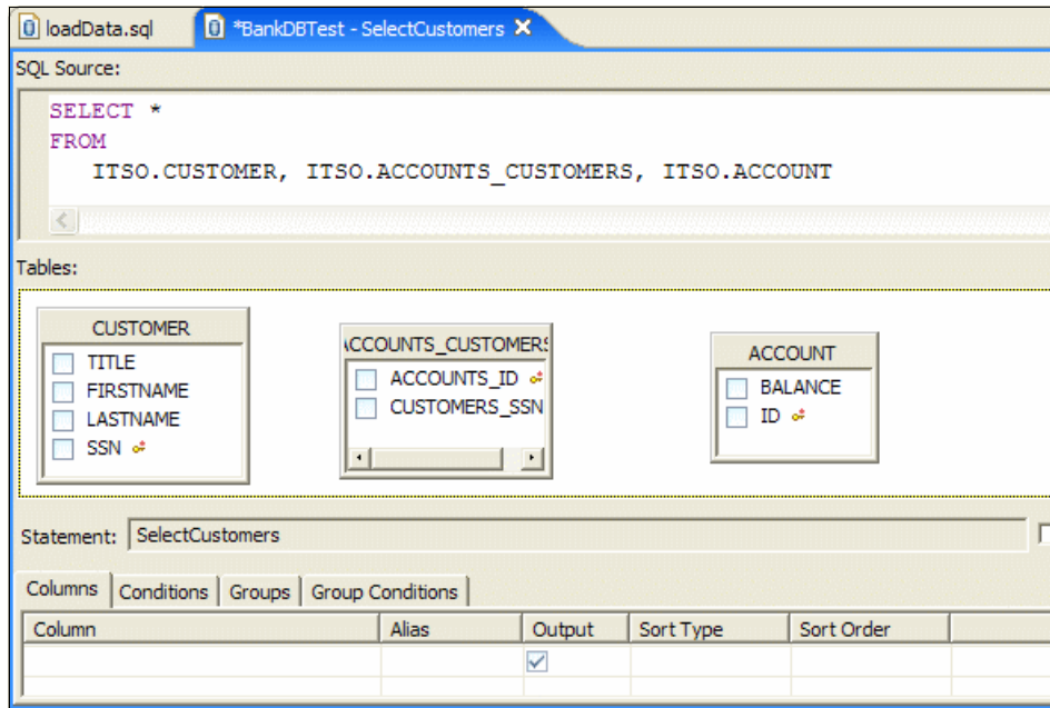
Figure 8-40 SQL Query Builder - Select tables
