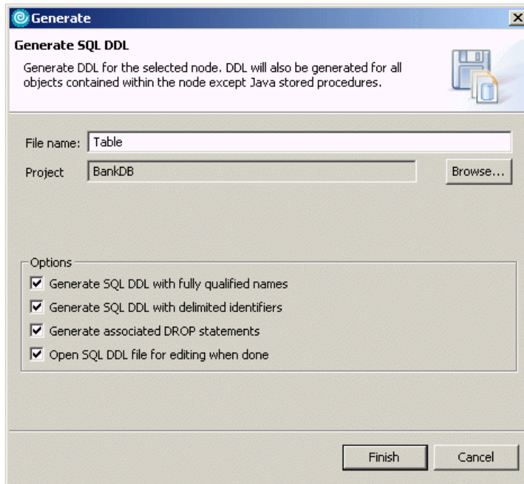
Figure 8-23 Generate DDL wizard - Generate SQL DDL for the BankDB database
