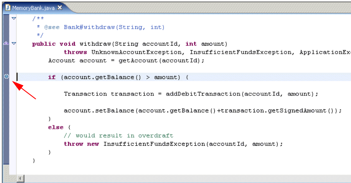
Figure 21-7 Add a breakpoint
