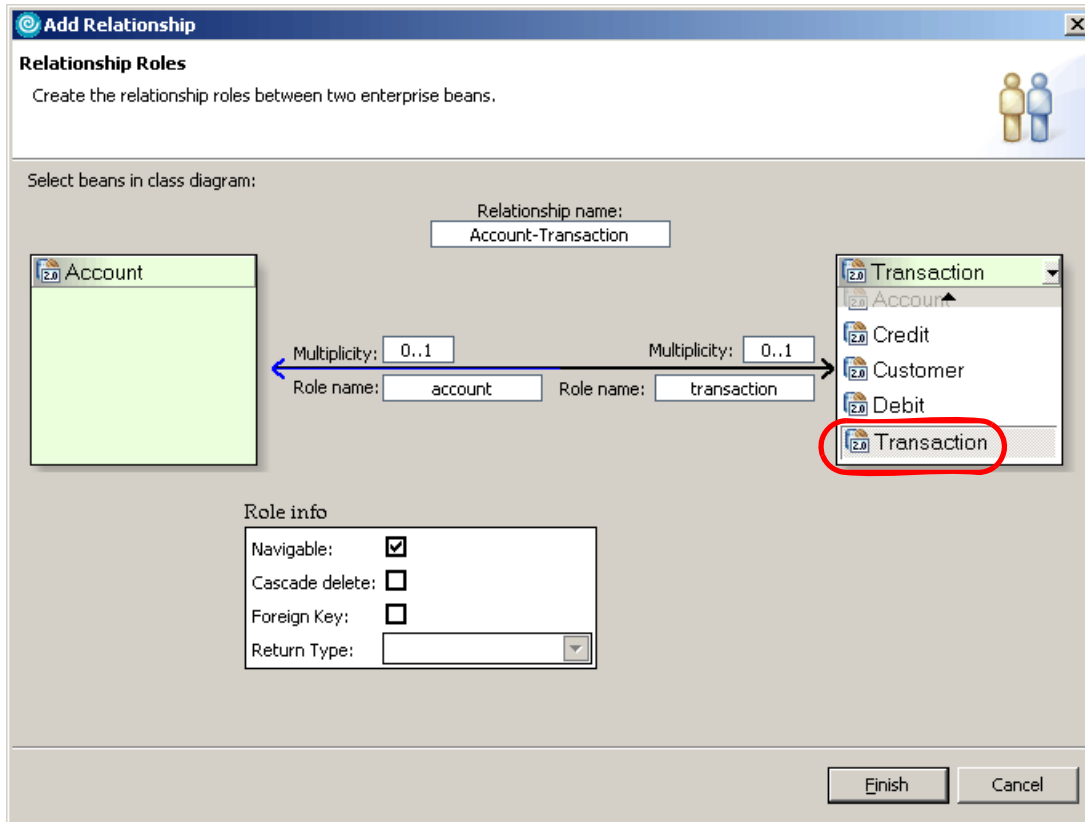
Figure 15-29 Add relationship wizard (part 1)
