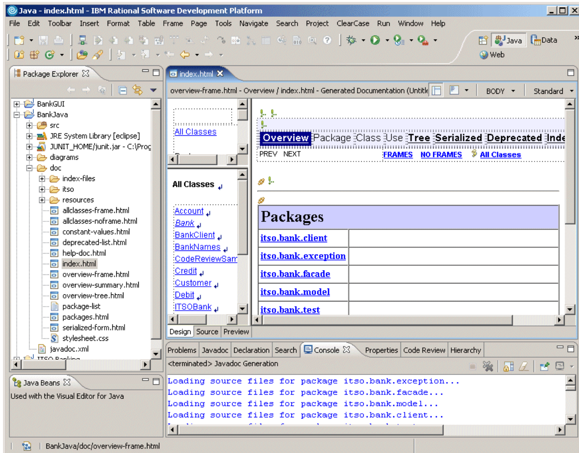
Figure 7-50 Javadoc output generated from the Javadoc Wizard for the BankJava project
