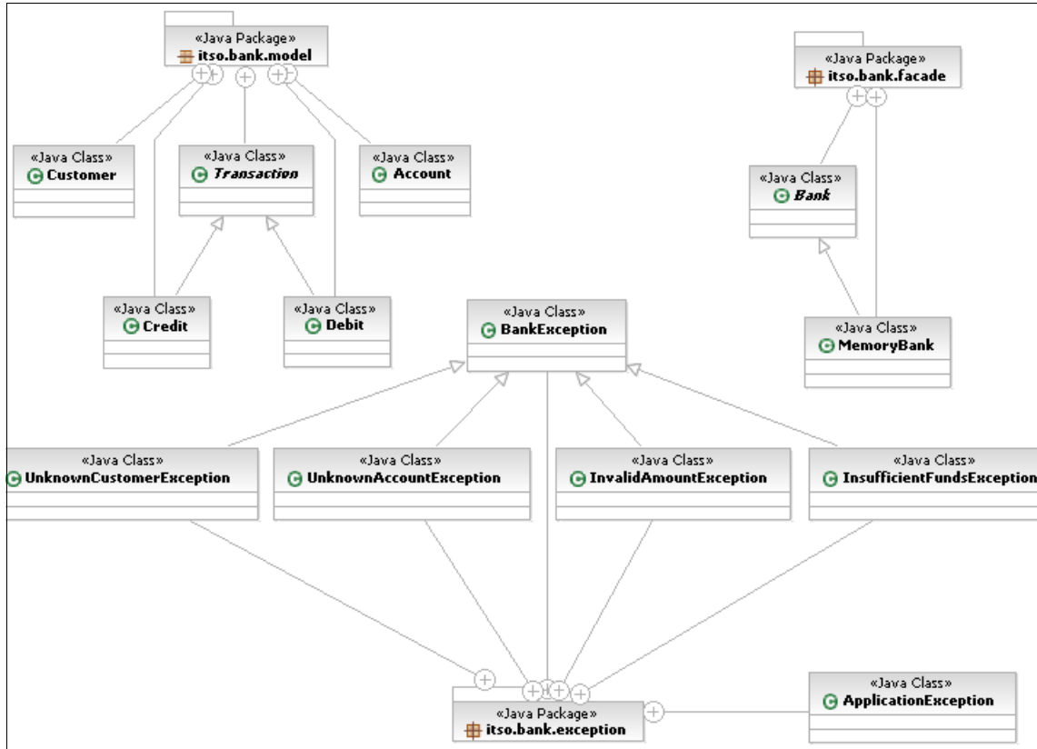
Figure 11-30 Class diagram with packages before adding attributes and methods
