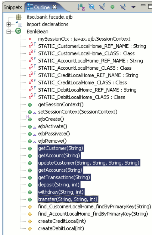
Figure 15-47 Promote Bank methods to the remote interface
