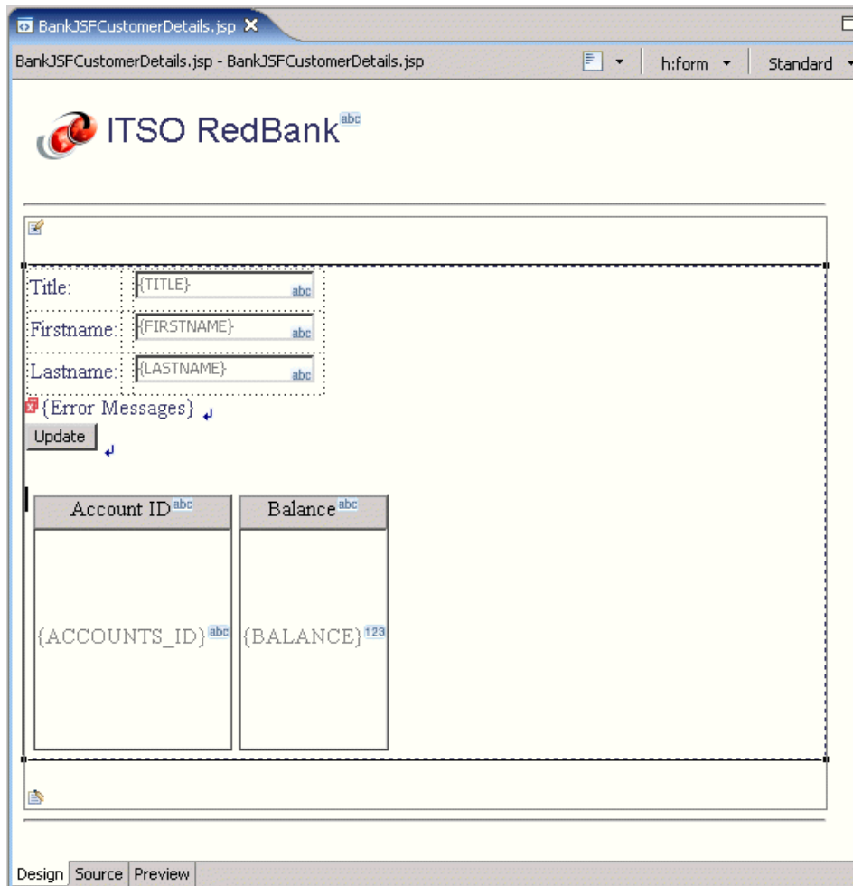
Figure 13-64 Design view of showing the table for customer accounts
