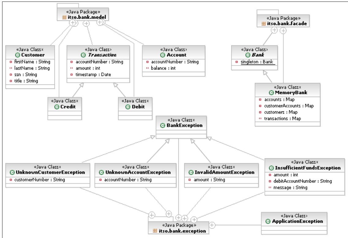
Figure 11-33 Class diagram with fields
