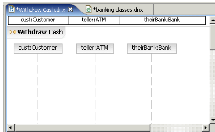
Figure 6-18 Sequence diagram with three lifelines
