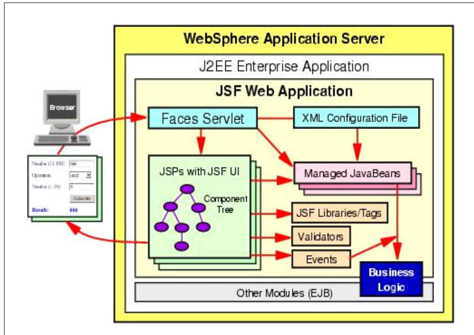
Figure 13-1 JSF application architecture
