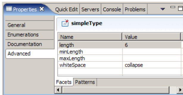
Figure 10-21 Advance tab for user-defined simple type, with a base type of string
