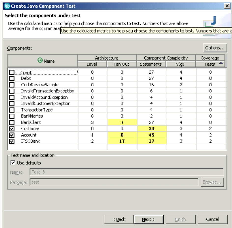
Figure 20-7 Select the components under test
