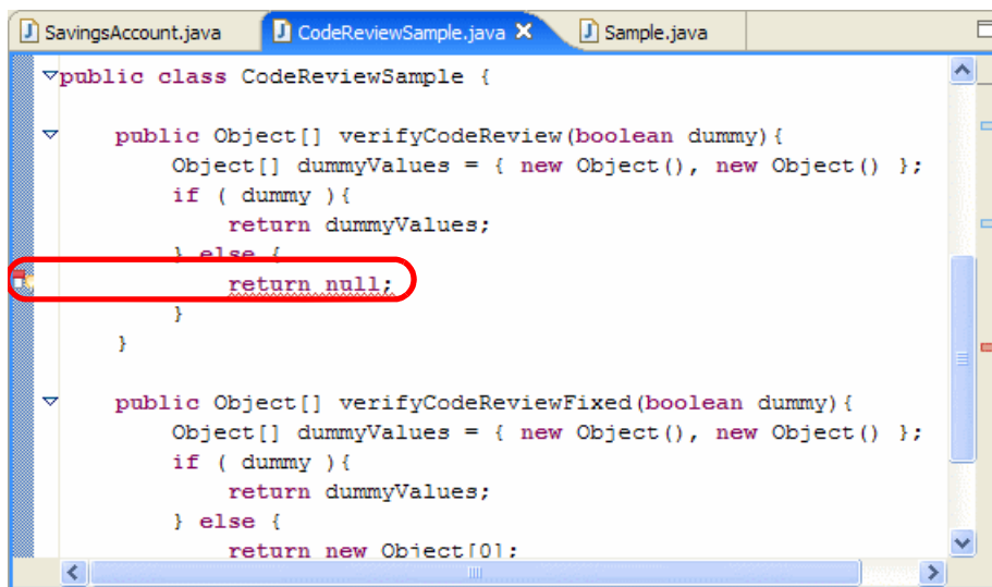
Figure 7-8 Editor displays the problem icon beside the offending line
