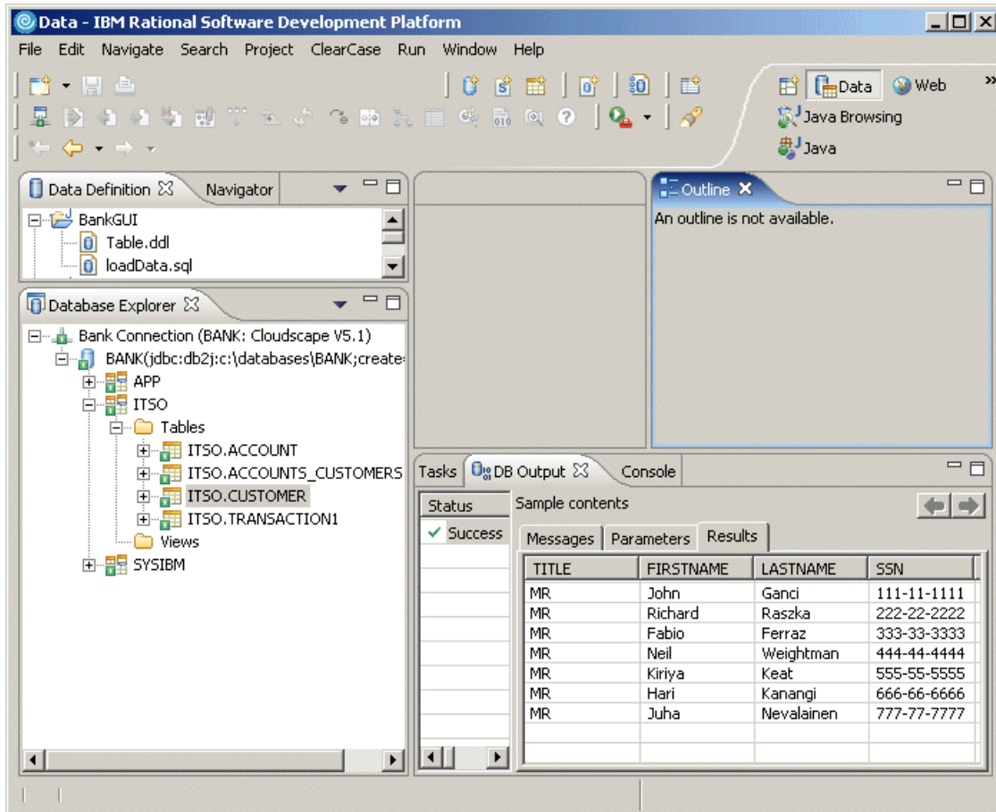
Figure 8-13 Bank connection working correctly
