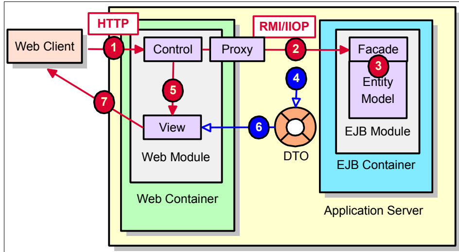
Figure 15-4 Application component model and workflow
