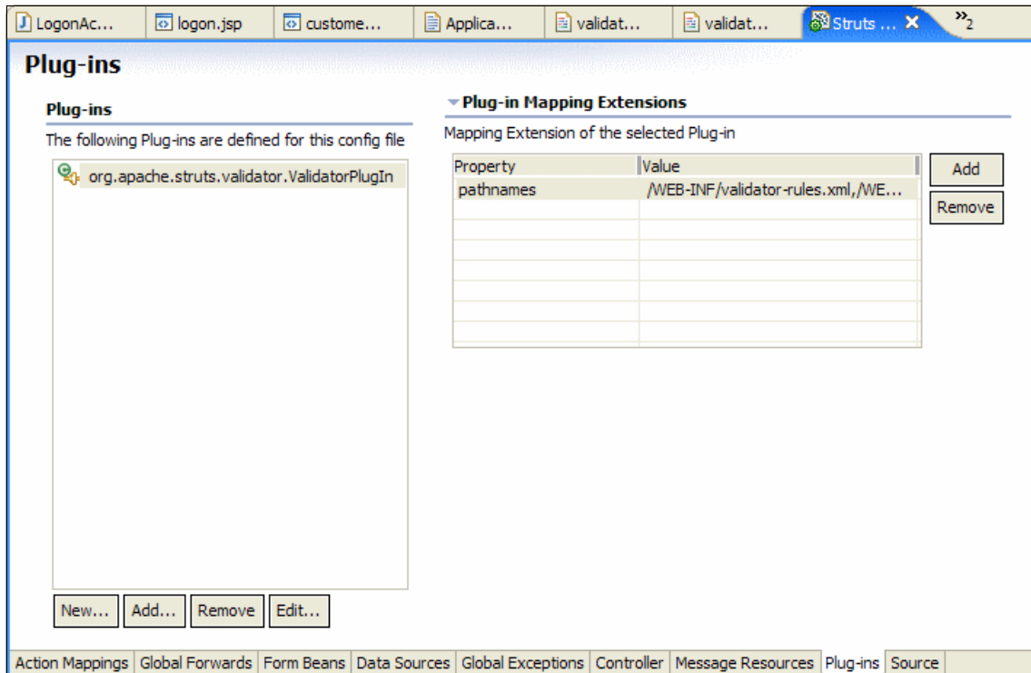
Figure 12-26 Struts Configuration Editor - Adding the validator plug-in
