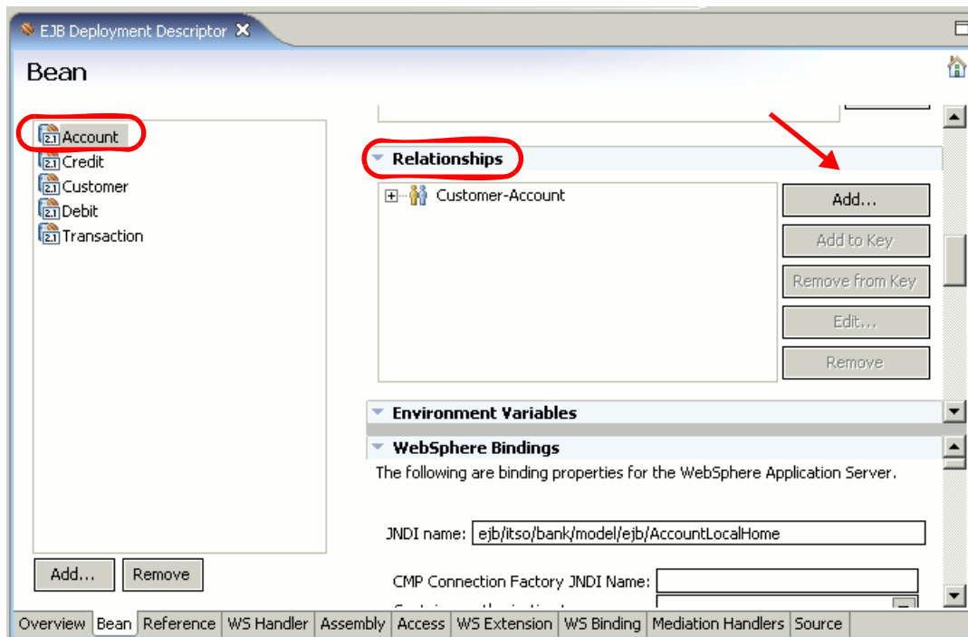
Figure 15-28 Defining relationships with the EJB Deployment Descriptor Editor
