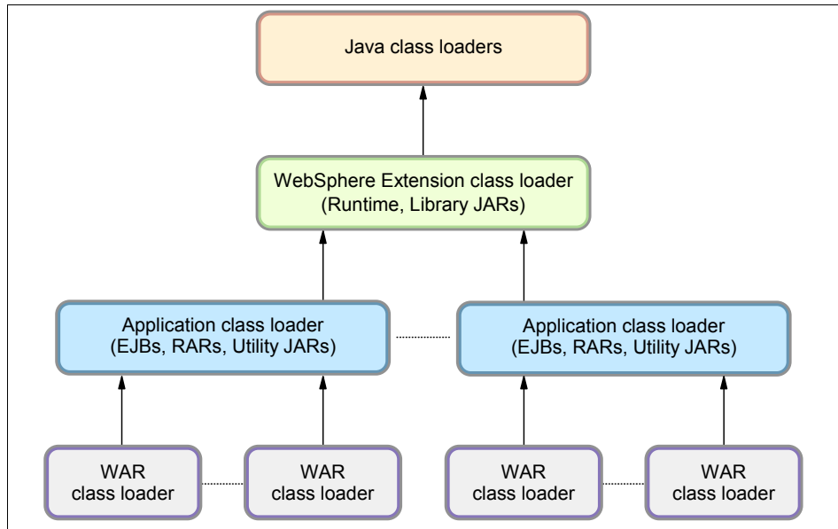
Figure 23-2 WebSphere class loaders hierarchy
