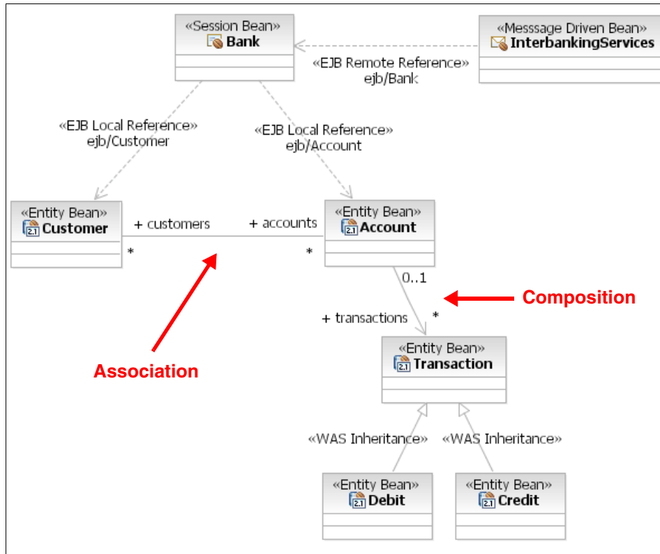
Figure 15-24 Association relationships in the model
