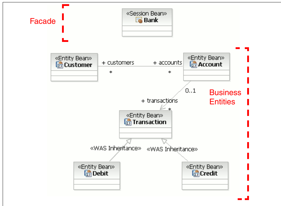
Figure 15-3 EJB module’s class diagram for RedBank application
