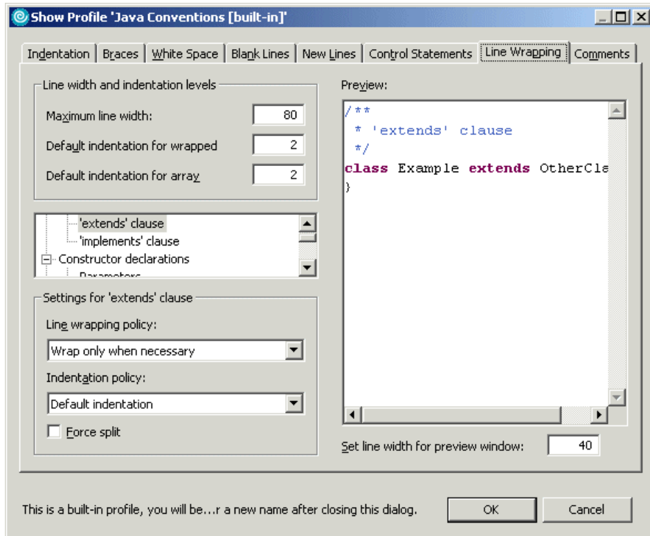
Figure 3-30 Code formatting - Line Wrapping
