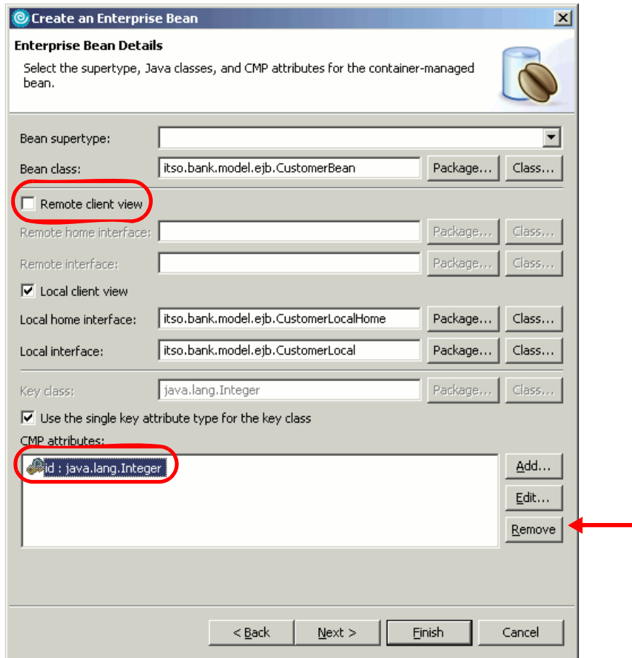
Figure 15-15 Create an entity bean (page 2)
