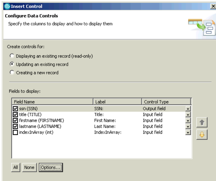
Figure 14-27 Insert customer record
