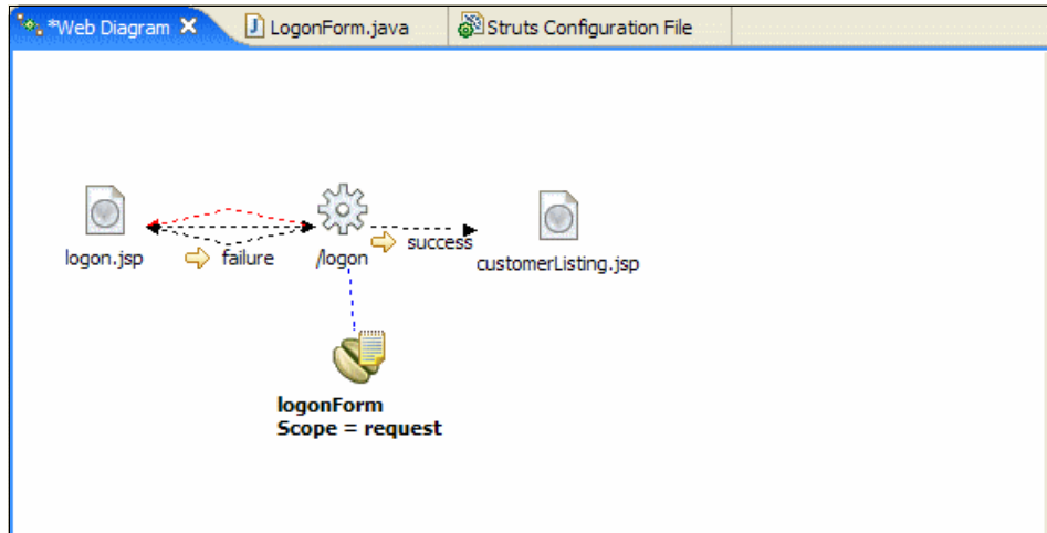
Figure 12-19 Realize Struts components - Logon form bean realized
