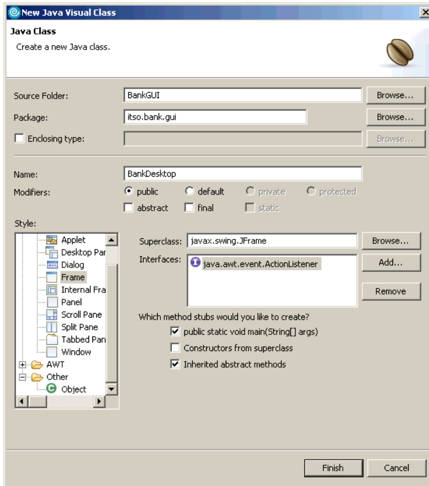
Figure 9-2 New Java Visual Class
