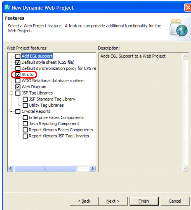
Figure 12-4 Create a Struts-based Dynamic Web Project - Select Features
