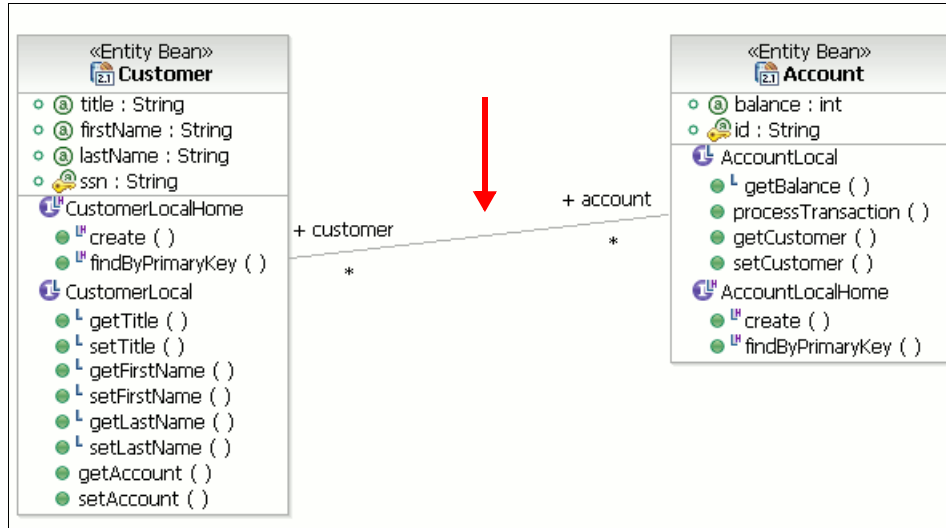
Figure 15-26 Association relationship between Customer and Account (part 1)
