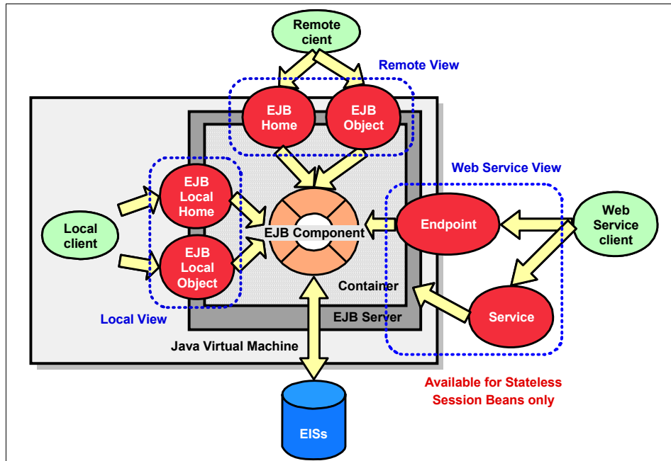
Figure 15-1 EJB architecture overview
