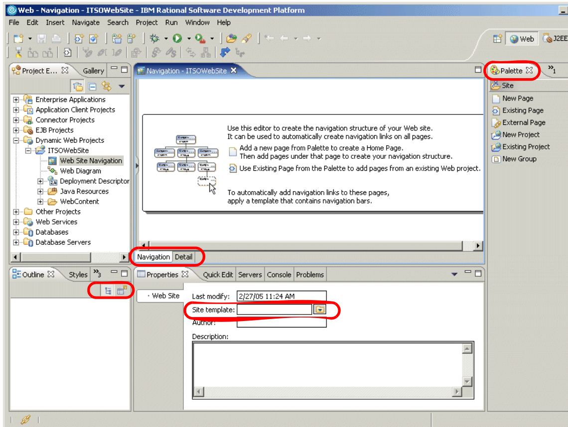
Figure 11-16 Web Site Designer - Navigation view
