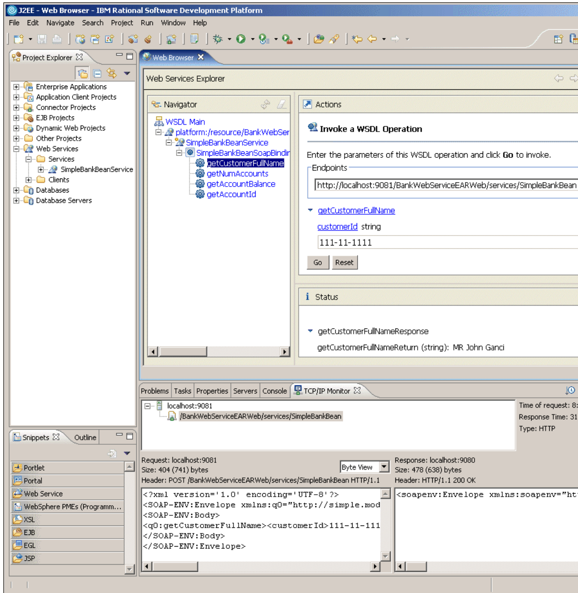
Figure 17-13 TCP/IP Monitor view
