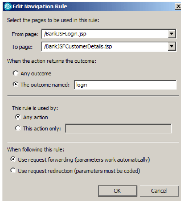
Figure 13-30 Edit Navigation Rule dialog
