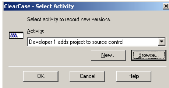
Figure 25-17 Specifying activity
