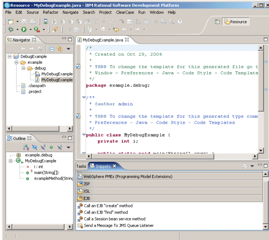
Figure 4-20 Resource perspective
