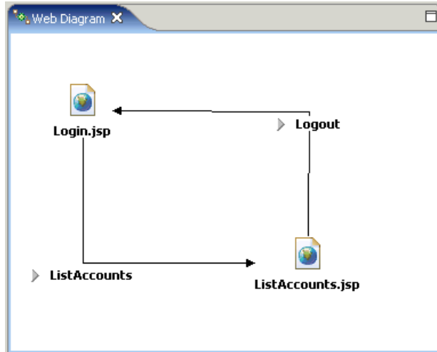
Figure 14-21 Web diagram
