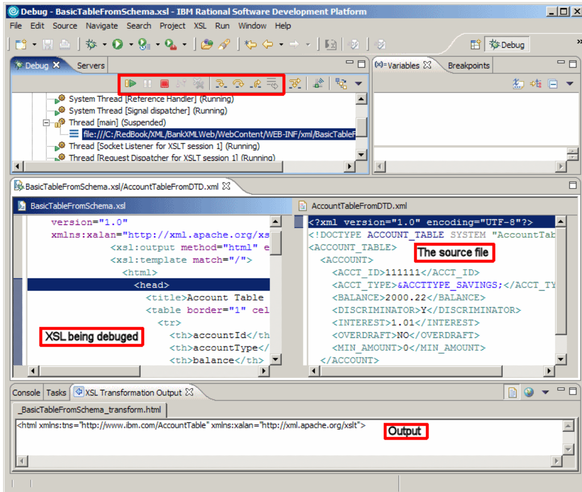
Figure 10-47 Debug perspective
