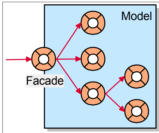
Figure 11-2 Model layer
