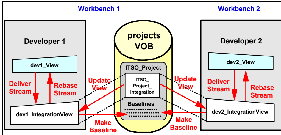
Figure 25-3 Scenario setup
