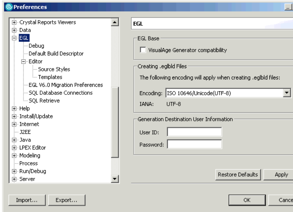
Figure 14-3 EGL preferences
