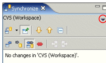
Figure 26-61 Synchronize view
