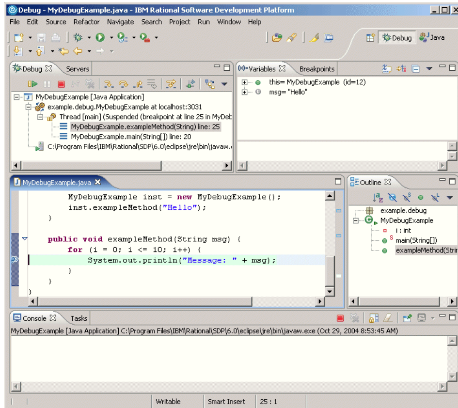
Figure 4-11 Debug perspective
