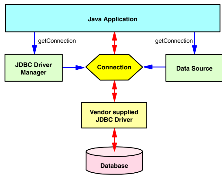
Figure 8-1 JDBC overview
