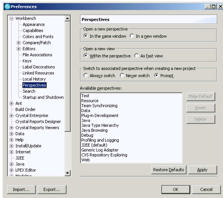
Figure 3-13 Perspectives preferences
