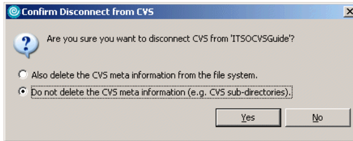
Figure 26-55 Disconnect confirmation
