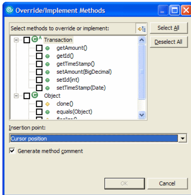
Figure 7-62 Java editor - Override/Implement Methods
