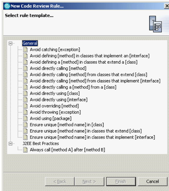
Figure 3-39 Adding a new rule to the J2EE Best Practices code review
