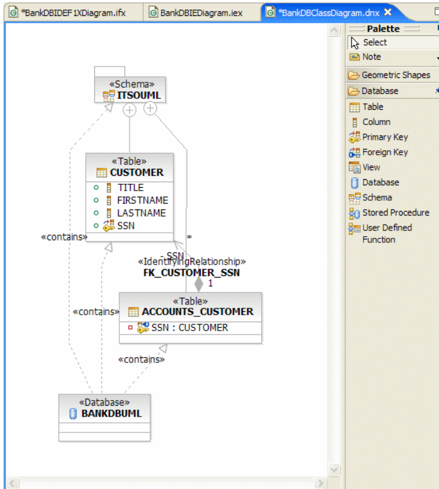
Figure 8-29 UML visualization - Class diagram
