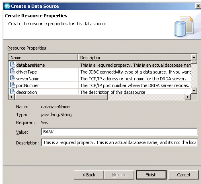
Figure 23-12 Create a Data Source (page 3)
