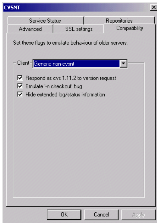
Figure 26-3 Compatibility settings required for interoperation with IBM Rational Application Developer V6 and other CVS clients
