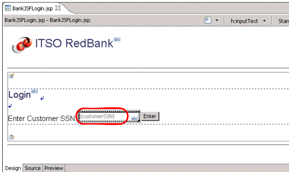
Figure 13-43 Design view - Bind input field and session scope variable
