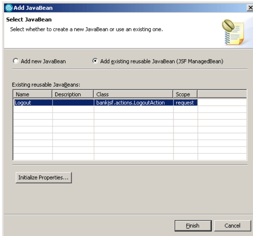
Figure 13-66 Add JavaBean wizard
