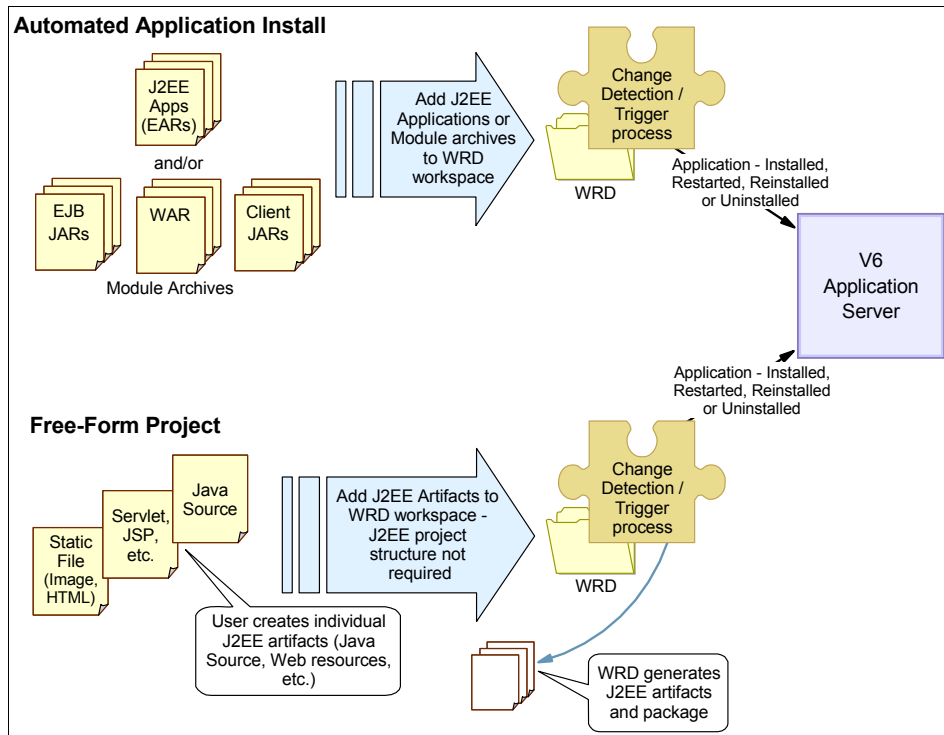
Figure 23-13 WebSphere Rapid Deployment modes
