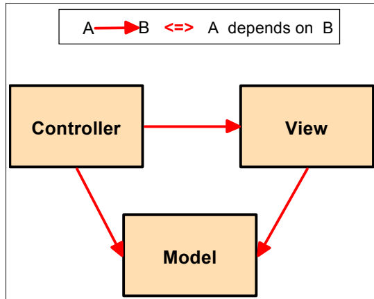
Figure 11-3 Dependencies allowed in the MVC pattern
