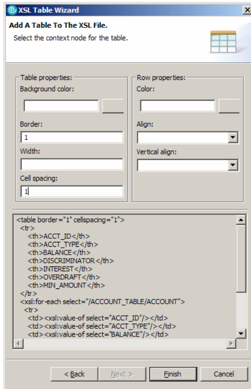
Figure 10-40 XSL Table wizard attributes
