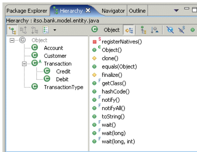
Figure 7-4 Type Hierarchy view
