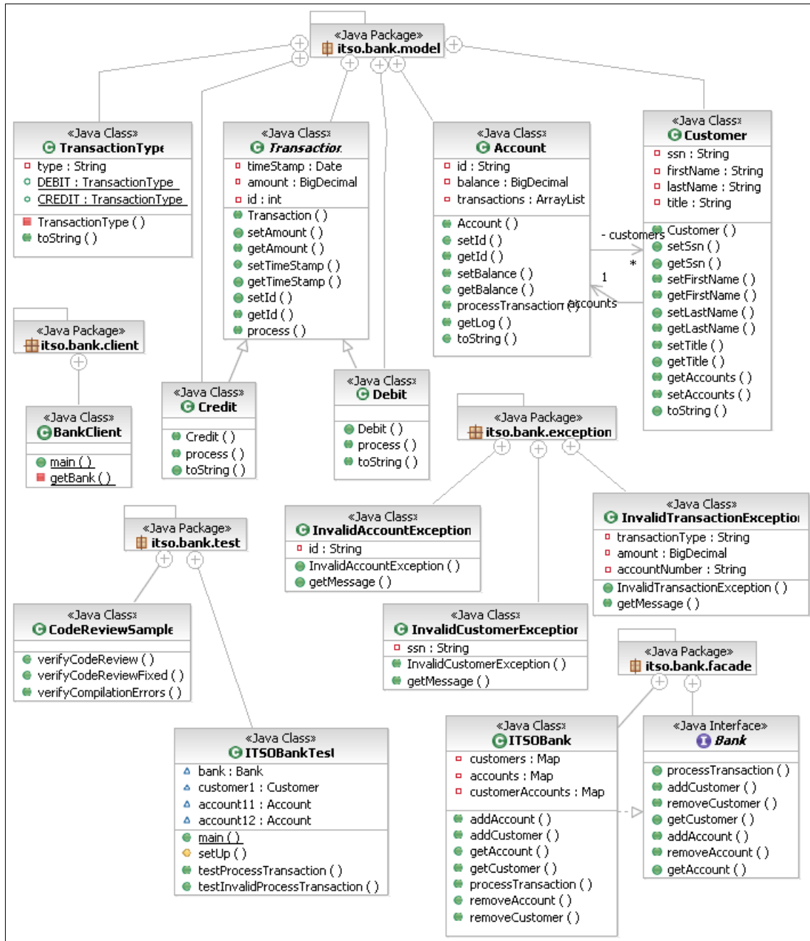
Figure 7-34 Completed class diagram - Banking sample
