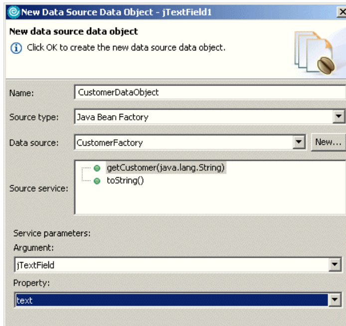
Figure 9-16 New Data Source Data Object dialog
