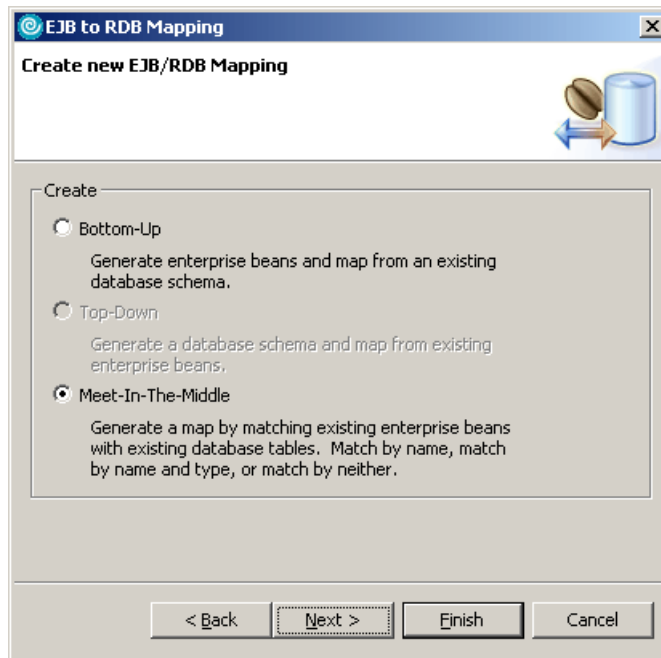
Figure 15-37 Creating a meet-in-the-middle EJB-to-RDB mapping
