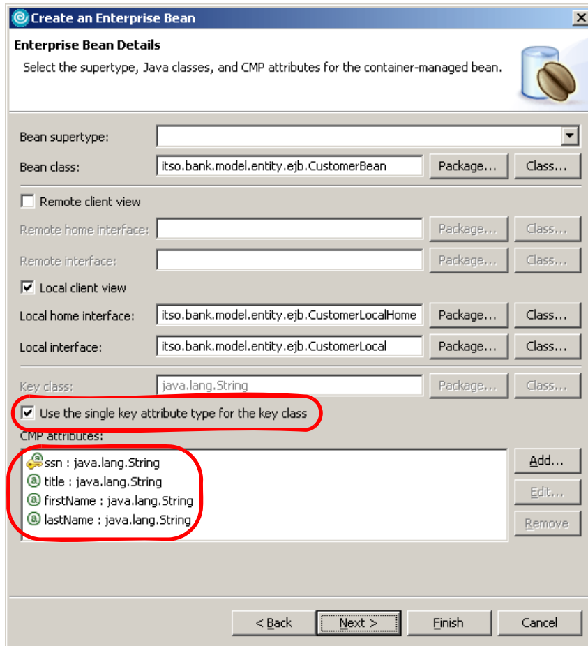
Figure 15-17 Creating an entity bean (page 2) after adding CMP attributes
