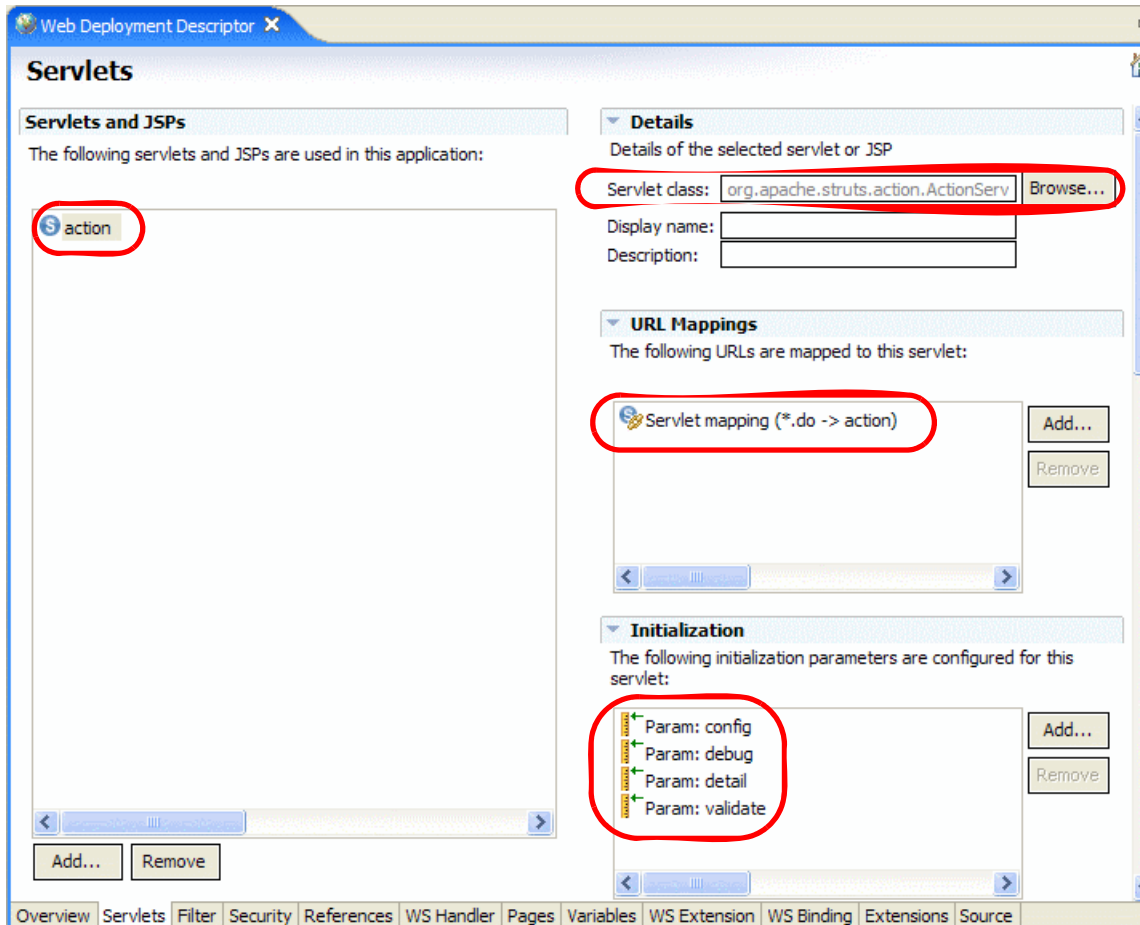
Figure 12-7 Generated Web Deployment Descriptor config for action servlet
