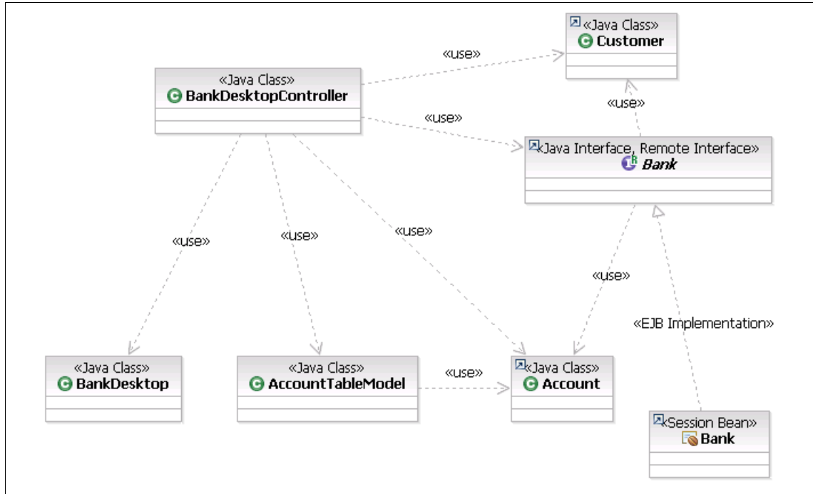
Figure 16-3 Class diagram for the ITSO Bank J2EE application client
