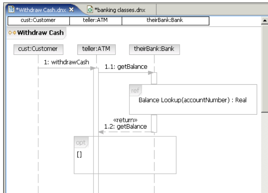
Figure 6-20 Sequence diagram with conditional fragment
