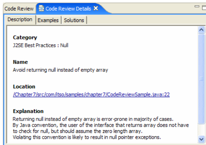
Figure 7-9 Code Review Details
