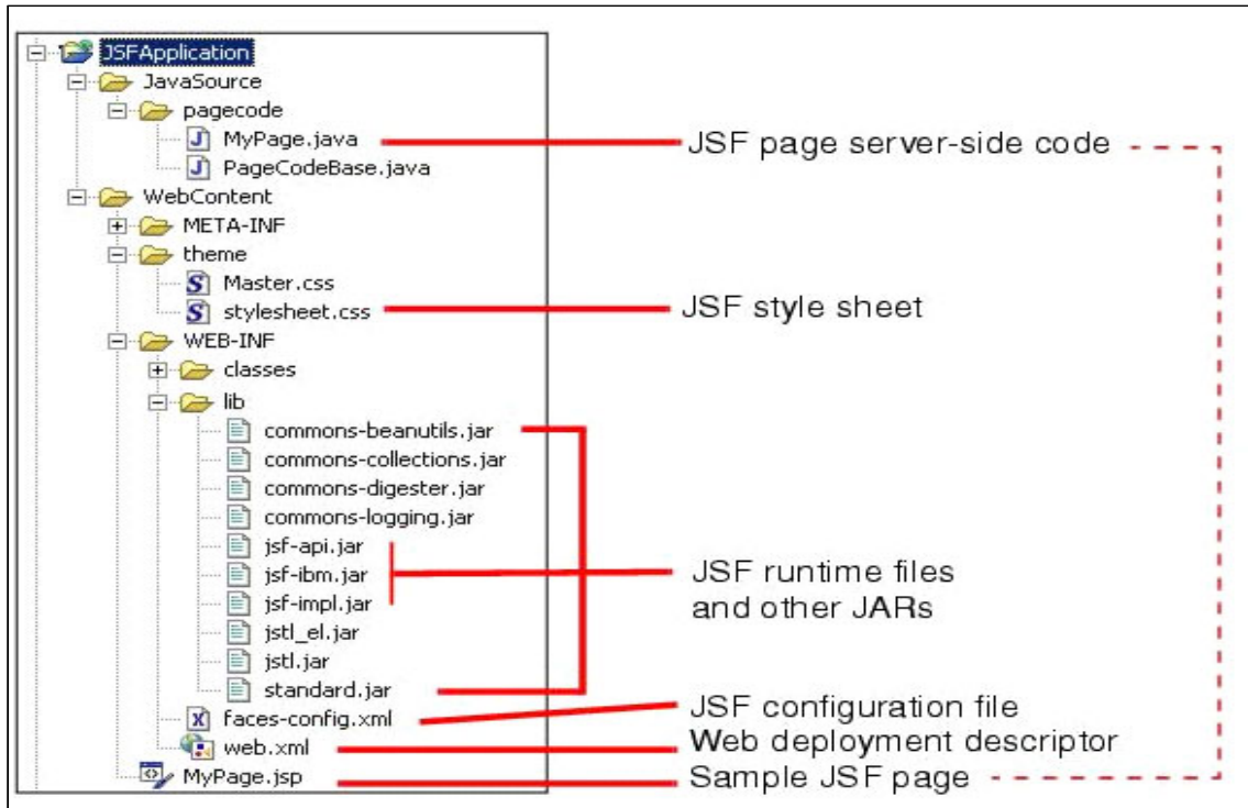
Figure 13-2 JSF application structure within Rational Application Developer
