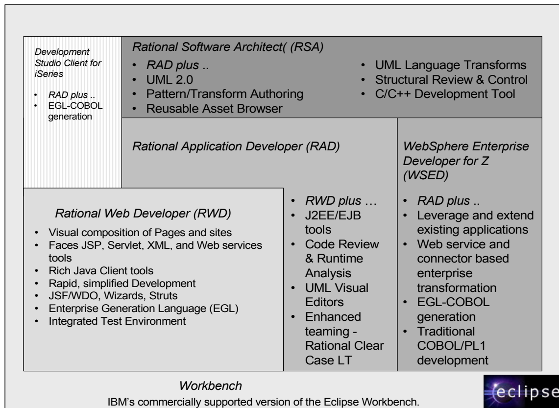
Figure 14-2 IBM Rational software containing IBM EGL
