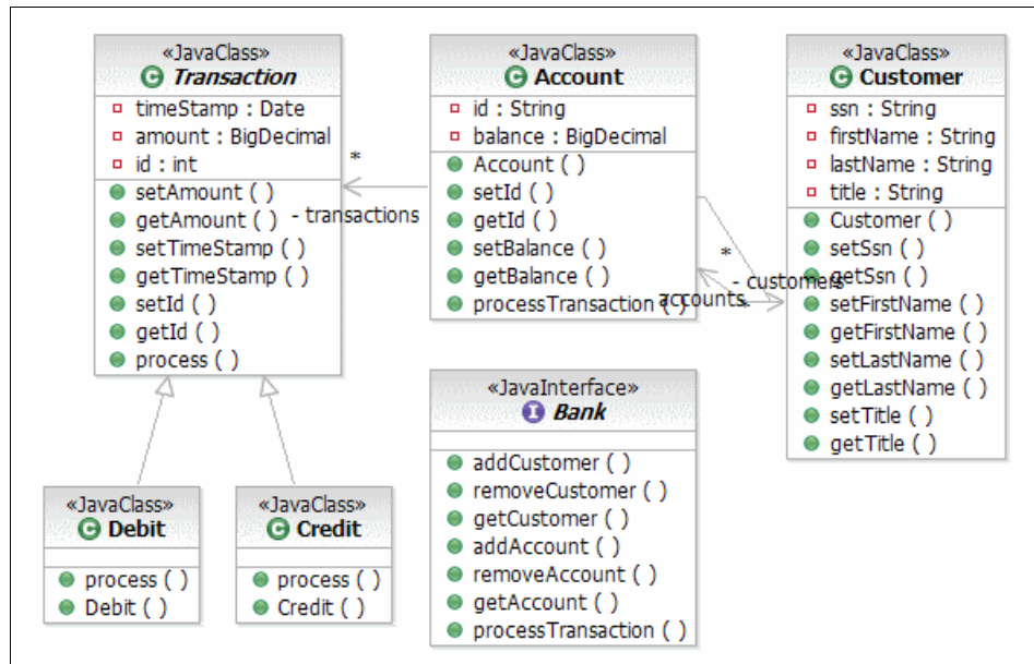
Figure 7-33 Class diagram with associations
