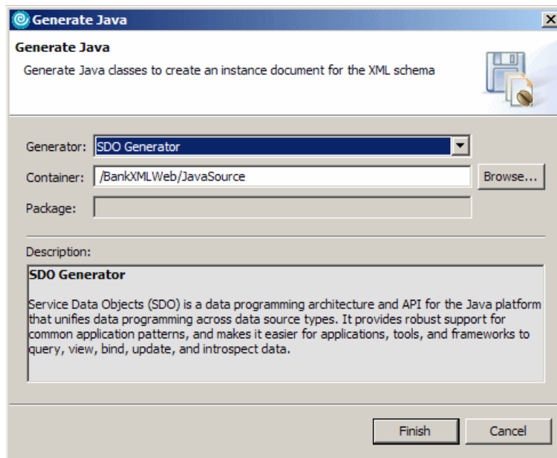
Figure 10-48 Java SDO classes generator
