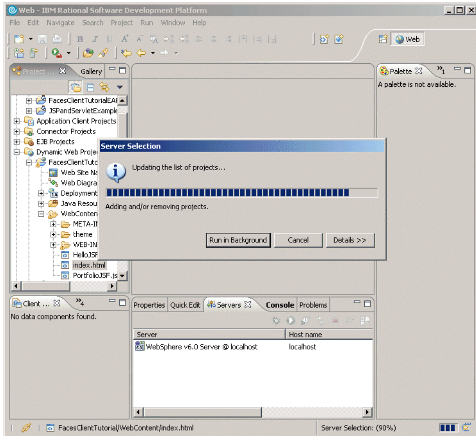
Figure 4-25 Blocking process
