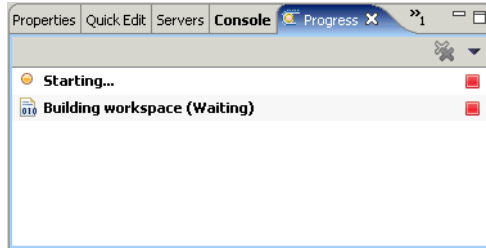
Figure 4-27 Progress view
