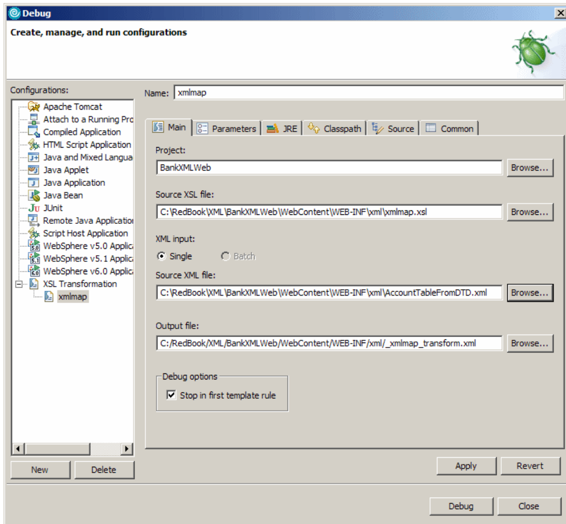
Figure 10-45 Debug dialog
