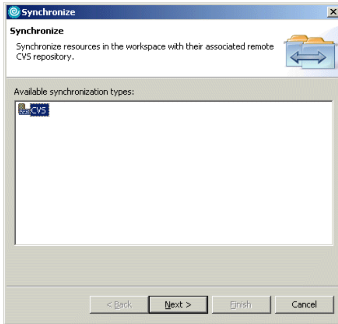
Figure 26-57 Synchronize dialog
