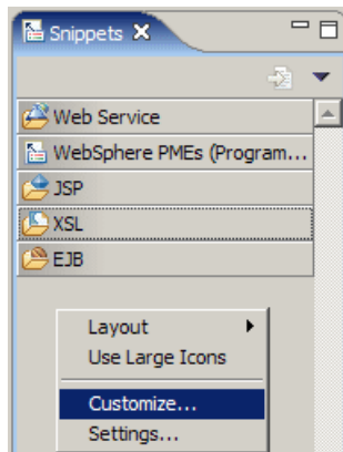
Figure 22-3 Customizing snippets
