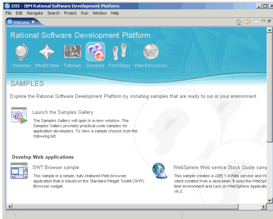
Figure 5-9 Samples page
