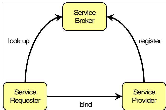
Figure 17-1 Service-oriented architecture
