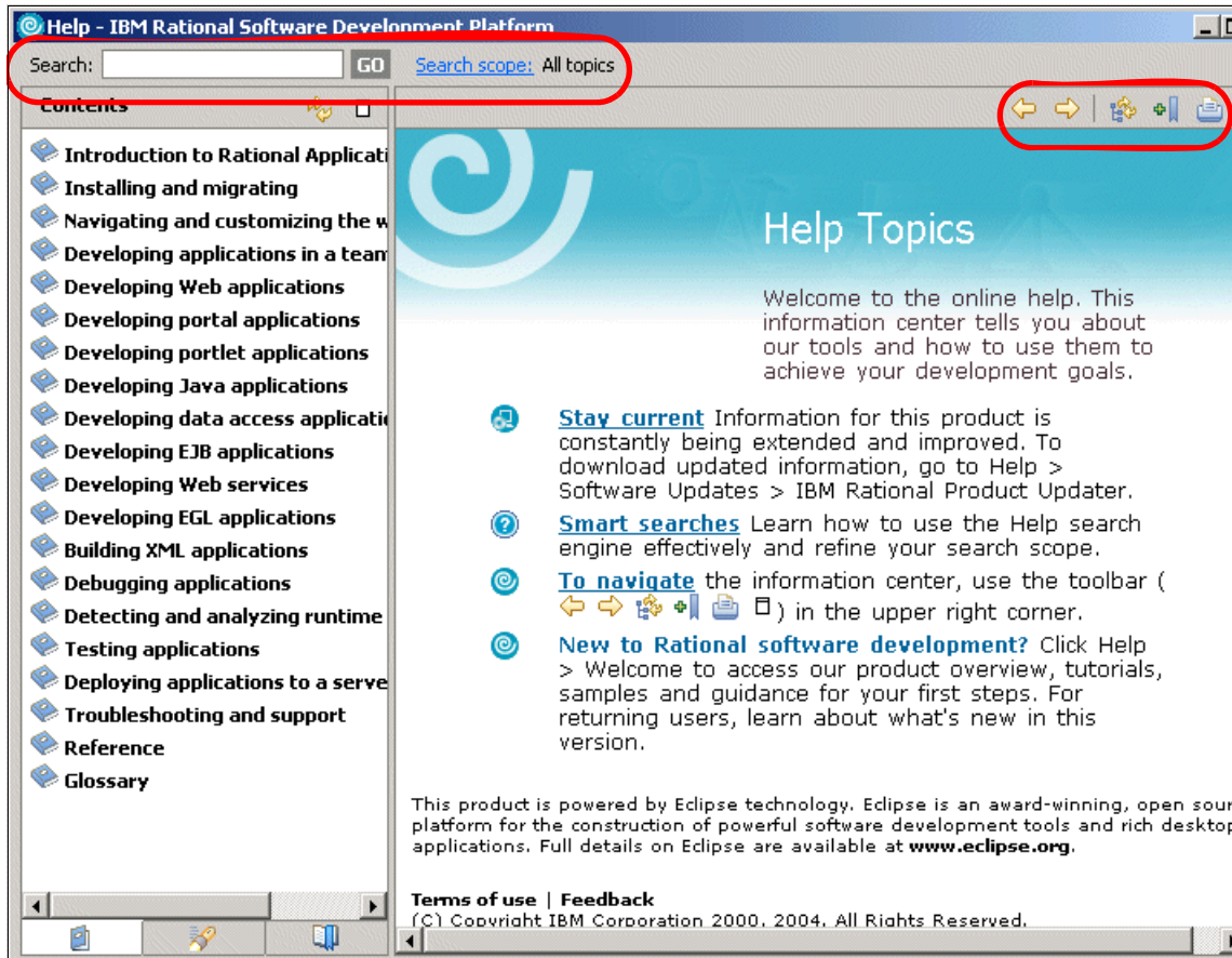
Figure 4-1 Help window
