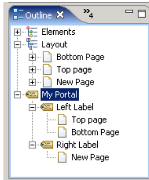
Figure 18-26 Outline view
