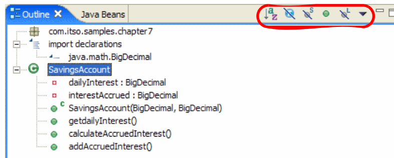
Figure 7-10 Outline view
