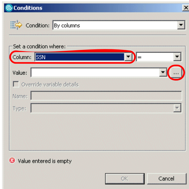
Figure 13-51 The Conditions dialog
