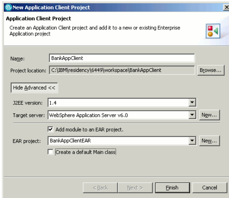
Figure 16-6 New Application Client Project wizard
