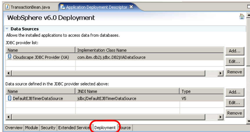
Figure 19-13 Enhanced EAR Editor
