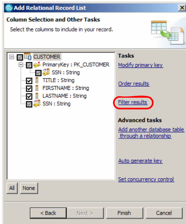
Figure 13-49 Column selection
