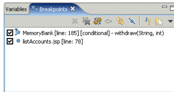
Figure 21-15 Debugging views
