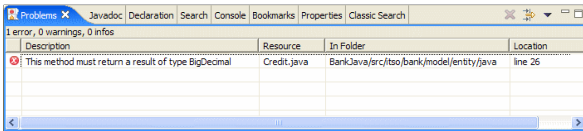
Figure 7-5 Problems view
