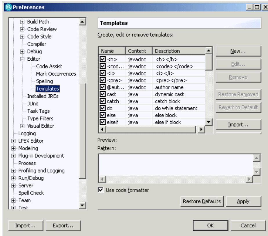
Figure 3-36 Templates preferences
