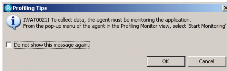
Figure 24-6 Profiling Tips
