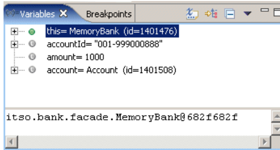
Figure 21-16 Displaying variables
