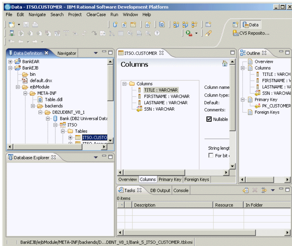
Figure 4-10 Data perspective
