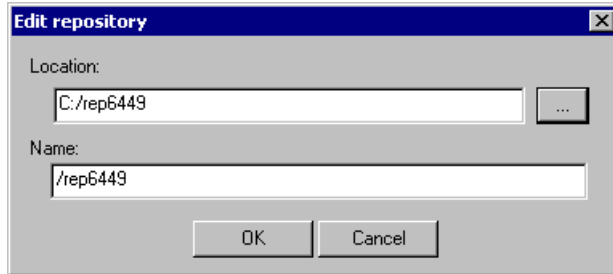
Figure 26-1 Add repository
