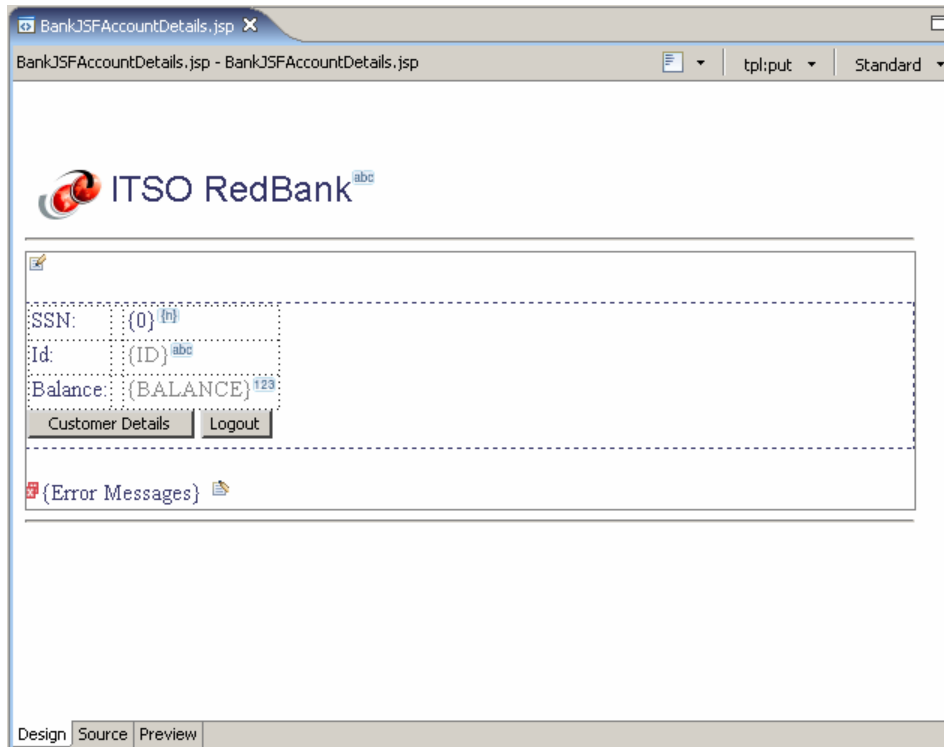
Figure 13-67 Finished BankJSFAccountDetails.jsp
