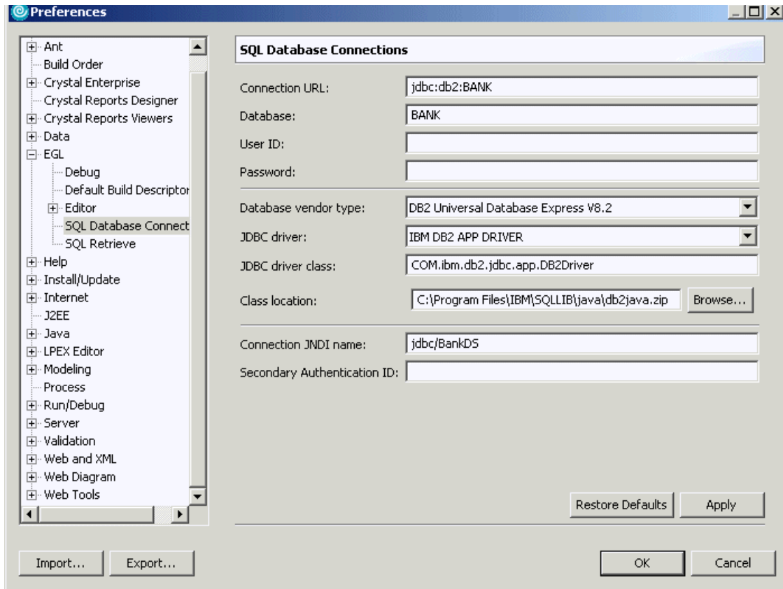
Figure 14-12 EGL preferences
