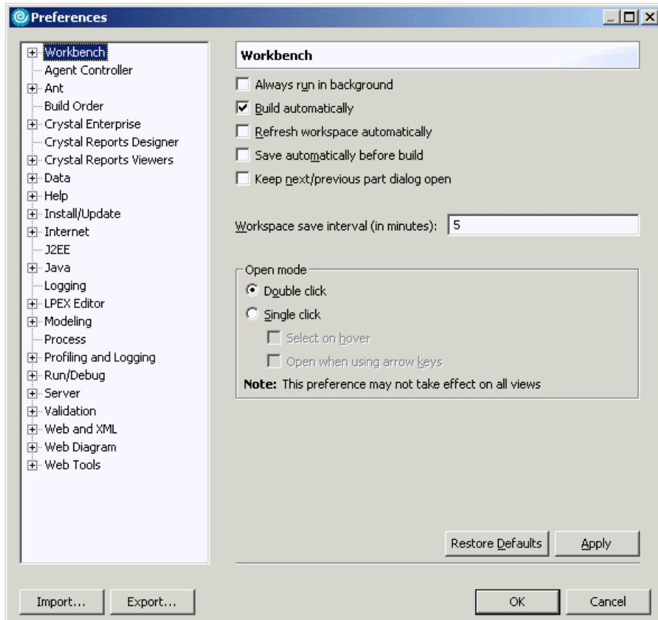
Figure 3-5 Workbench preferences
