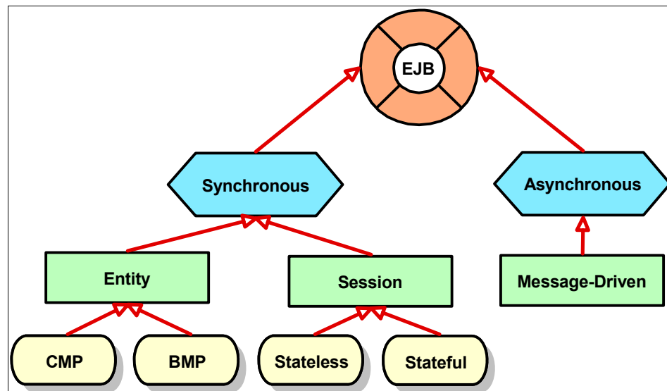
Figure 15-2 EJB types
