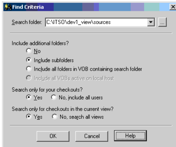
Figure 25-21 Finding checkouts
