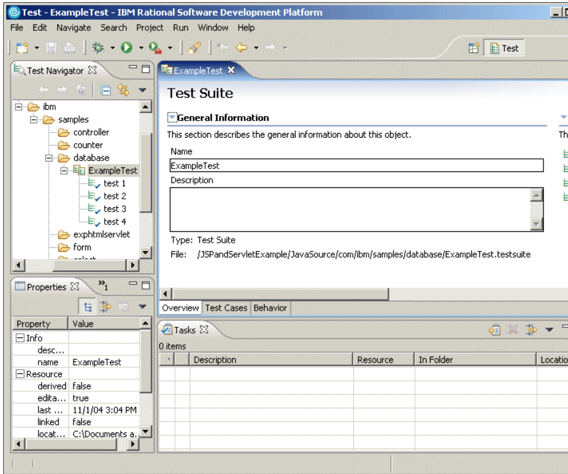
Figure 4-22 Test perspective
