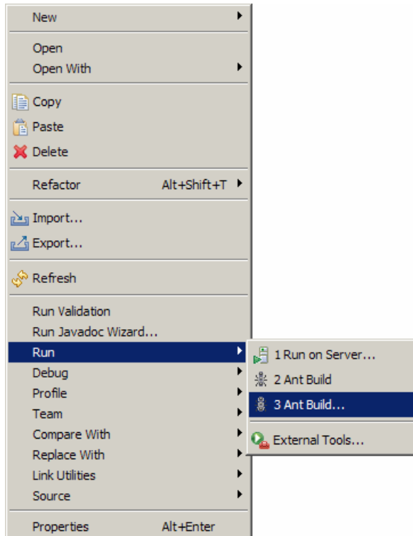
Figure 22-13 Launching Ant
