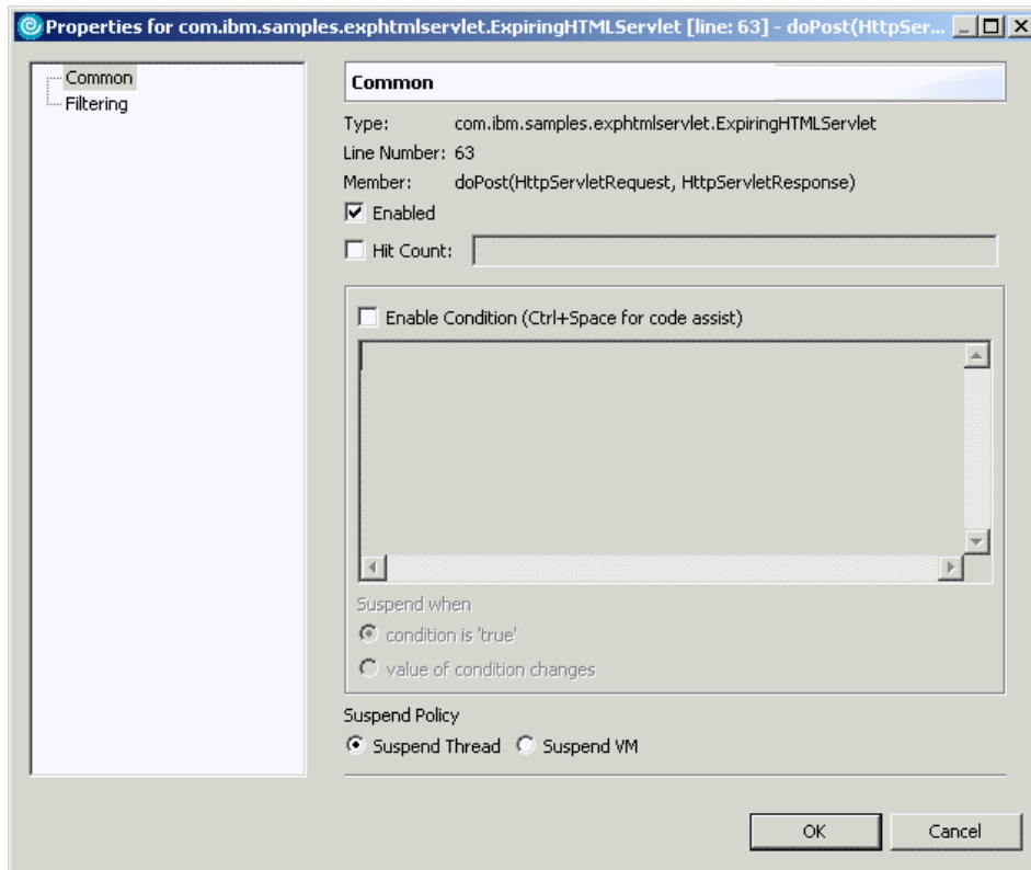
Figure 21-8 Breakpoint properties
