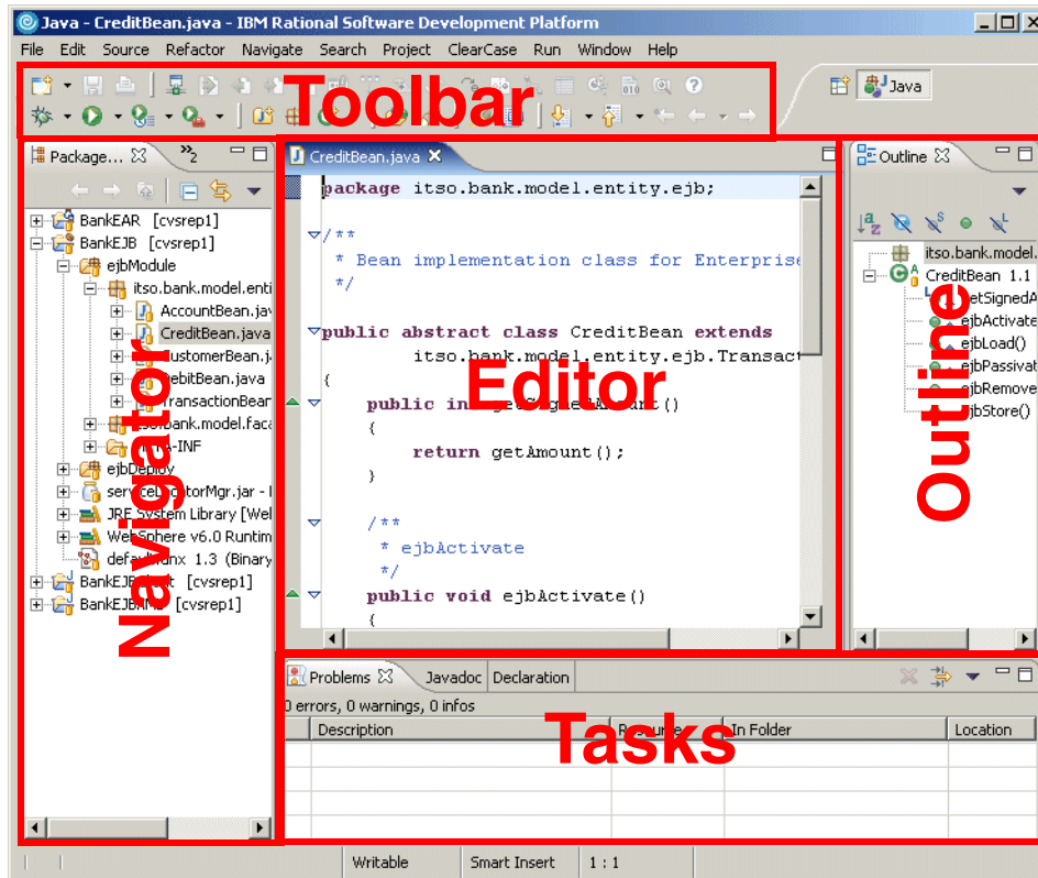
Figure 4-5 Perspective layout
