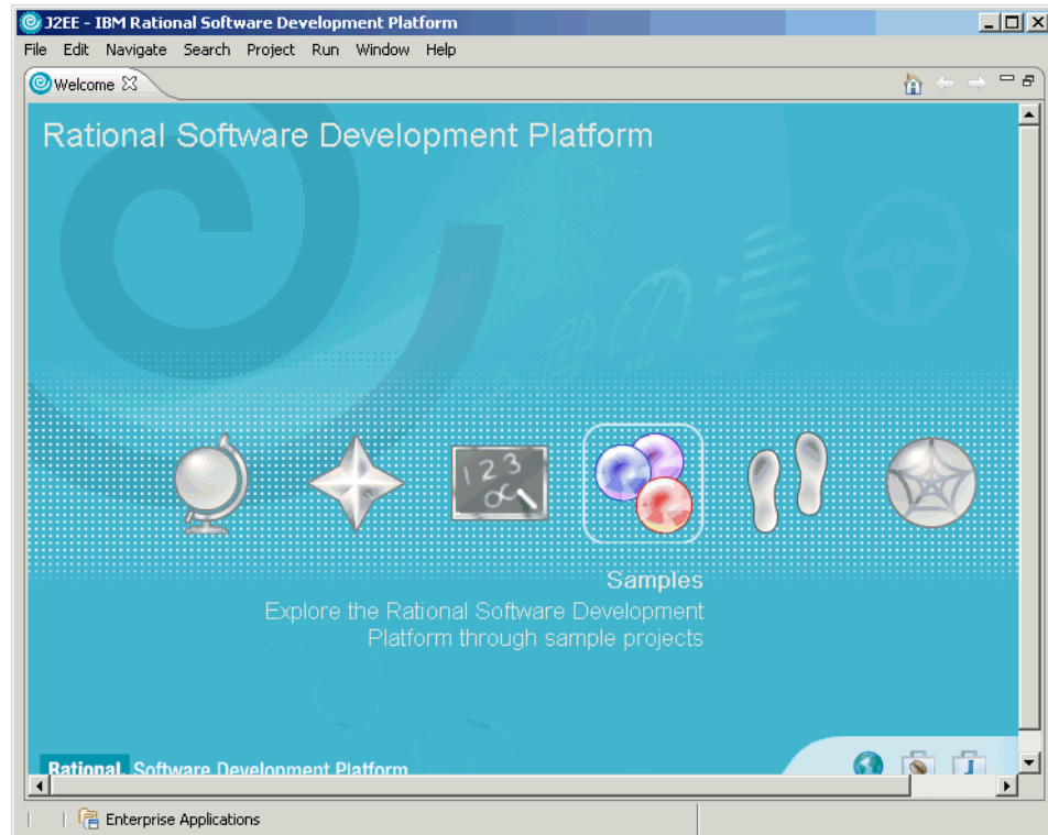
Figure 5-8 Welcome page
