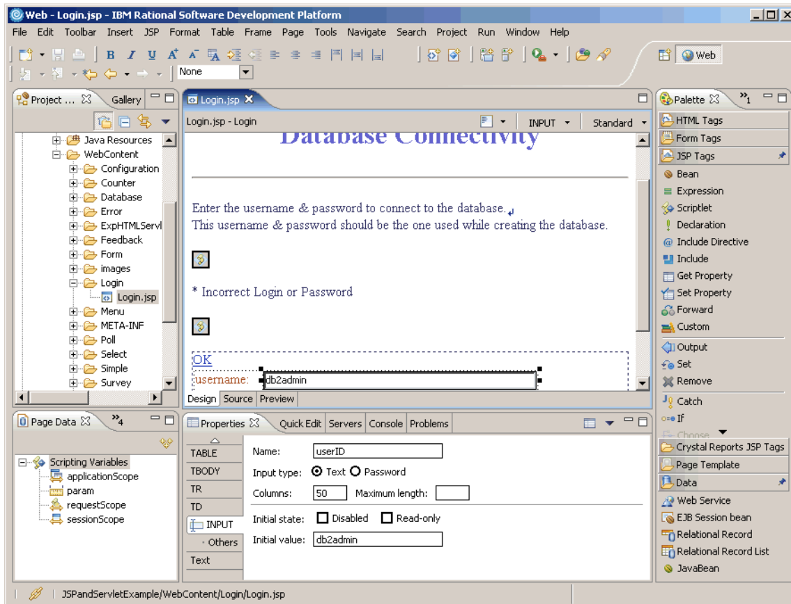
Figure 4-23 Web perspective
