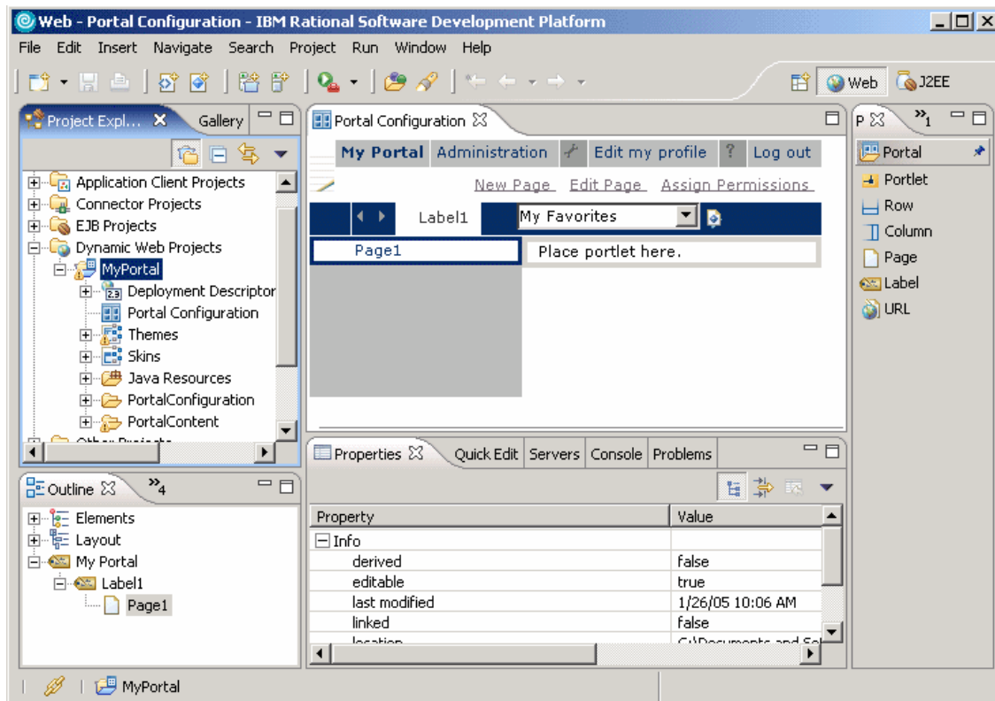
Figure 18-6 Portal Designer
