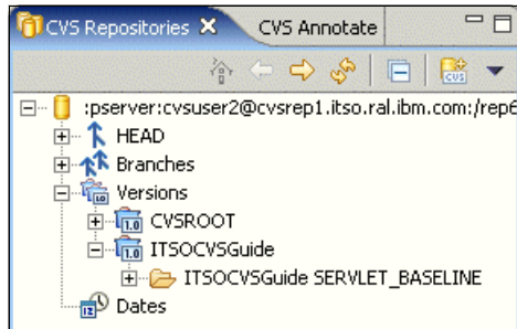
Figure 26-36 Project version
