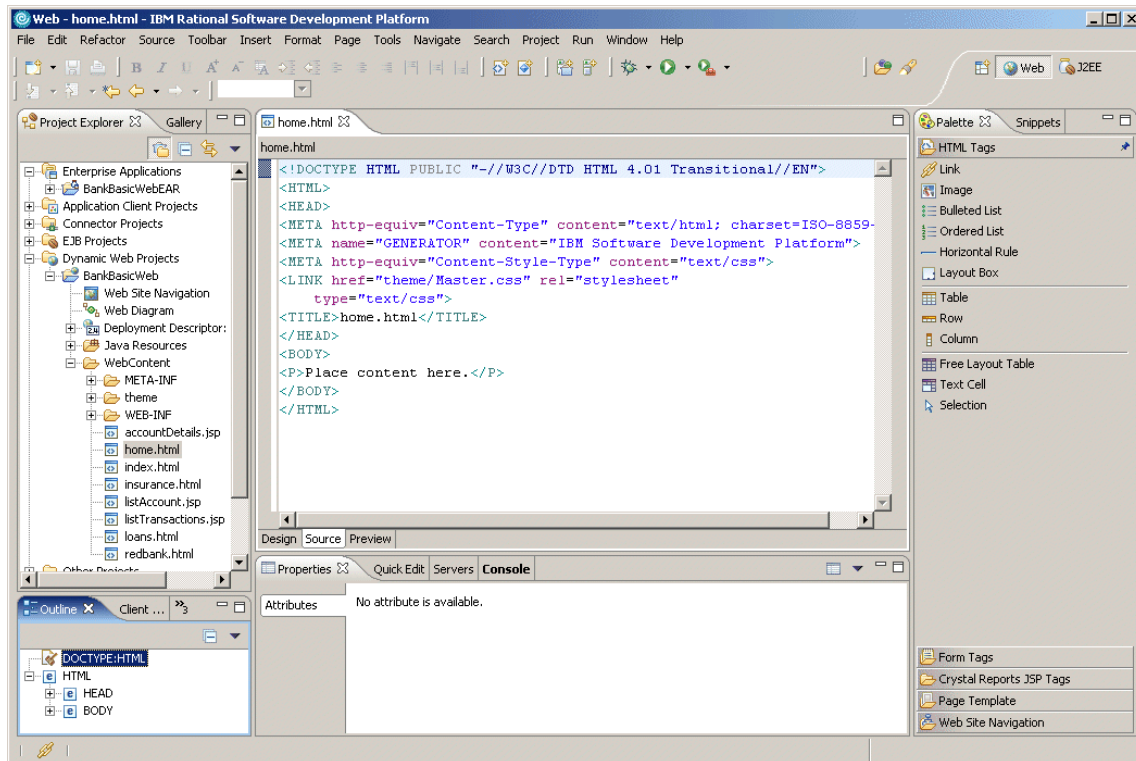
Figure 11-4 Web perspective
