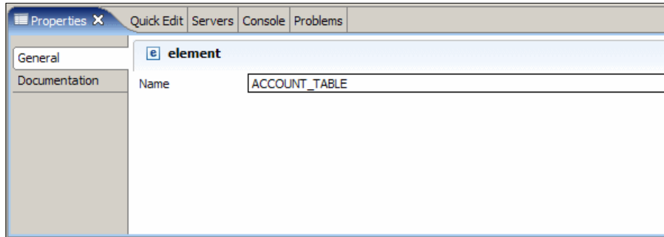
Figure 10-6 Properties view
