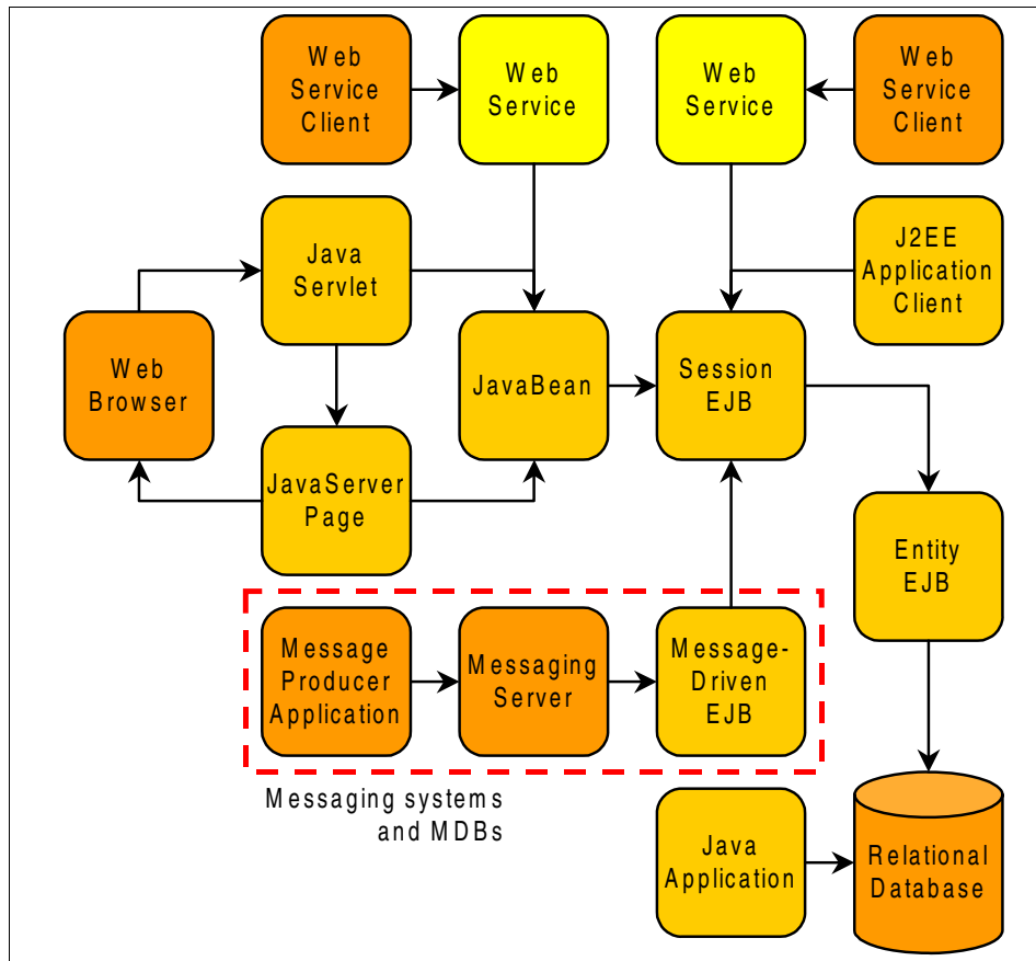
Figure 2-8 Messaging systems
