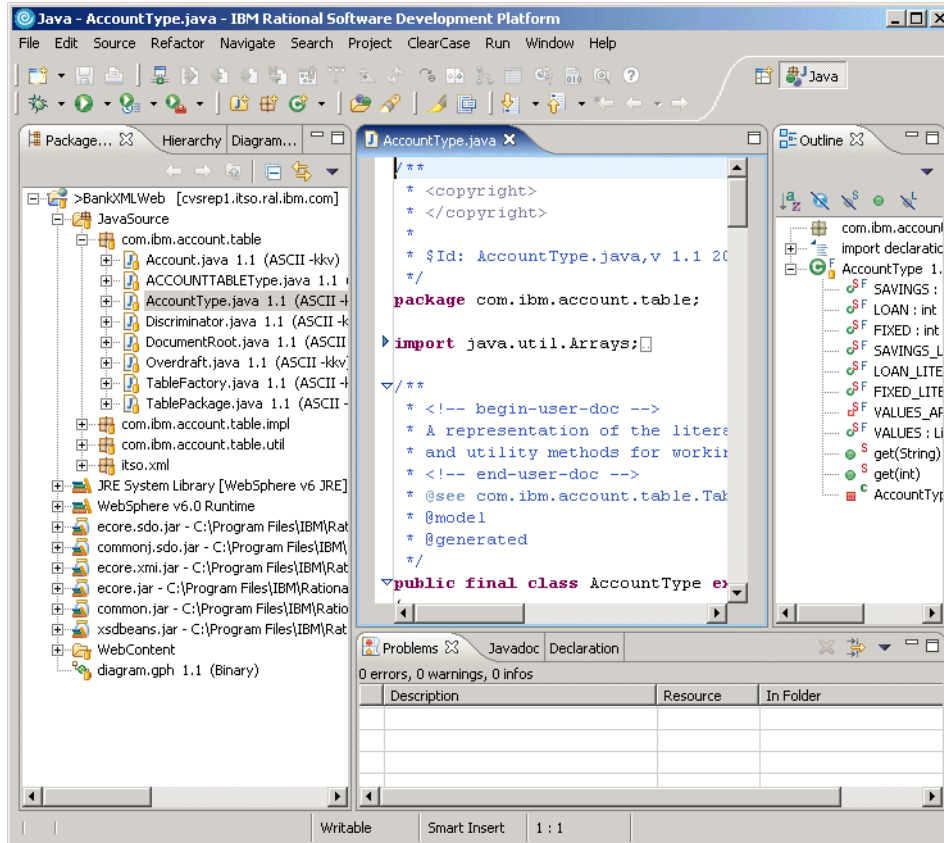
Figure 4-13 Java perspective
