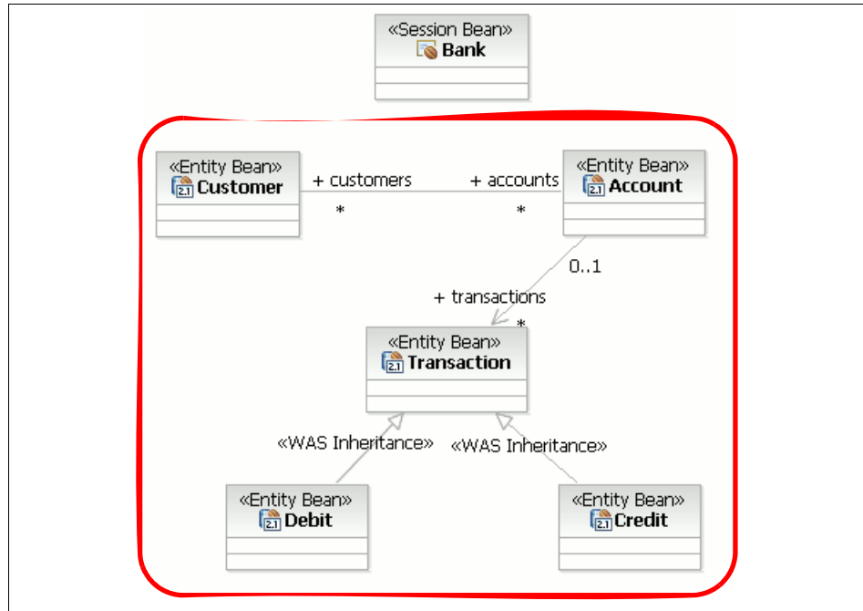
Figure 15-13 Business entities
