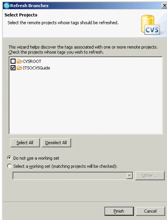
Figure 26-53 Refreshing branches
