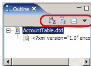
Figure 10-5 Outline view
