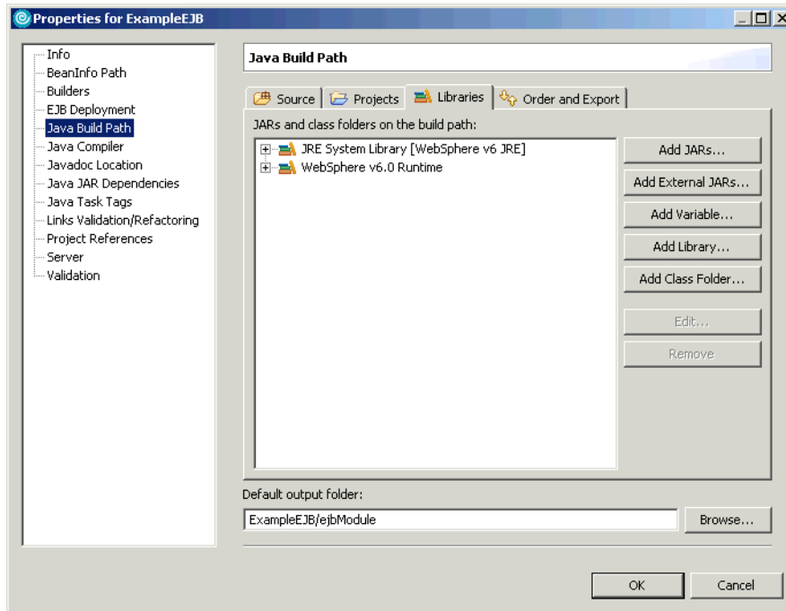
Figure 5-7 Project properties
