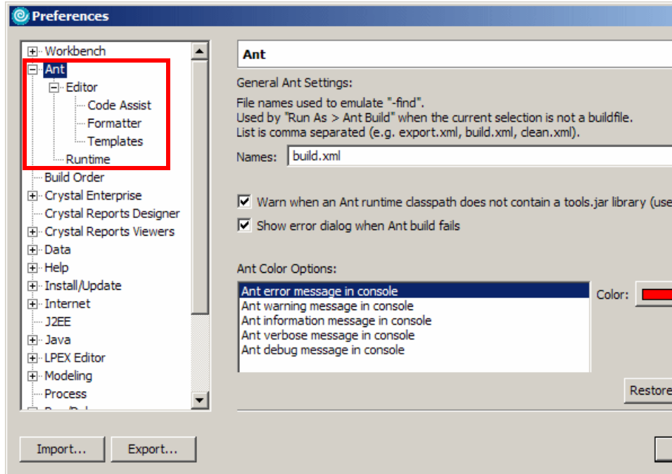
Figure 22-8 Ant preferences
