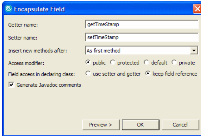
Figure 7-29 Encapsulate Field
