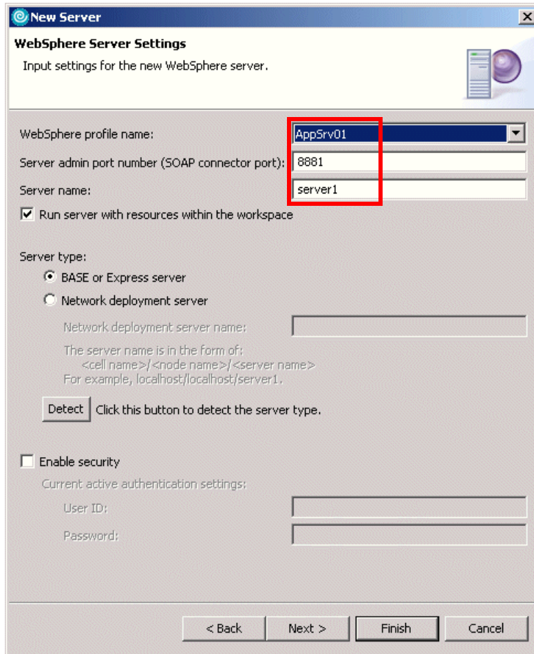
Figure 19-7 Define a New Server - WebSphere Server Settings
