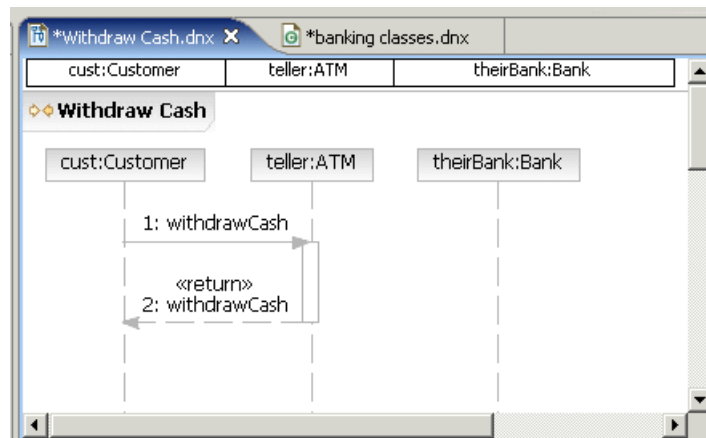
Figure 6-19 Adding a message to sequence diagram
