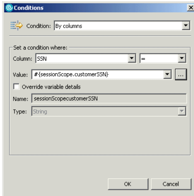
Figure 13-53 Conditions dialog with values
