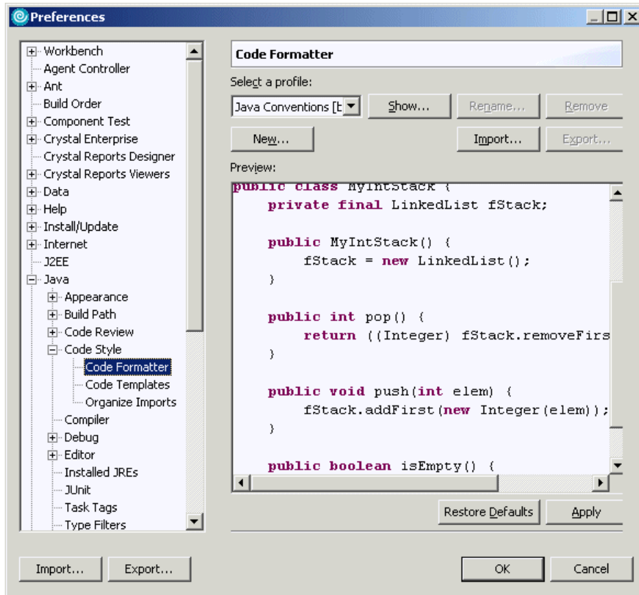
Figure 3-23 Code formatter profiles setup in IBM Rational Application Developer V6
