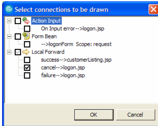
Figure 12-33 Struts Configuration Editor - Selecting Struts components to draw
