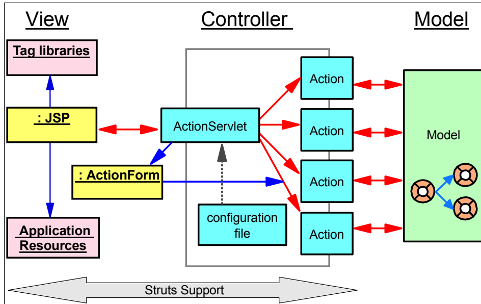
Figure 12-1 Struts components in the MVC architecture
