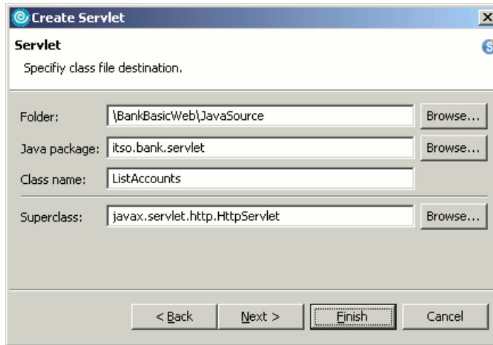
Figure 11-36 New servlet wizard (page 2)
