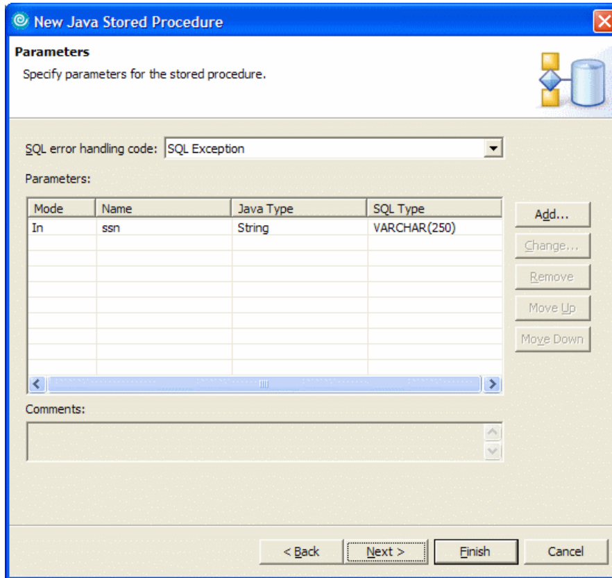
Figure 8-48 Java stored procedure - Specify parameters for the stored procedure
