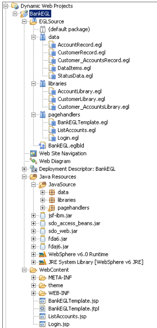
Figure 14-4 Components of a sample EGL Web application
