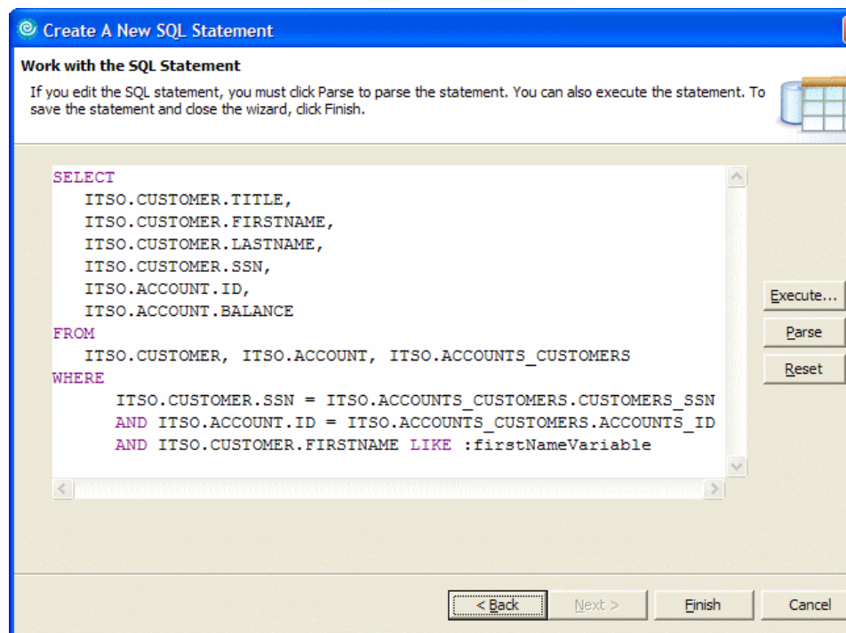
Figure 8-36 SQL Statement wizard - Construct an SQL Statement - Generated SQL
