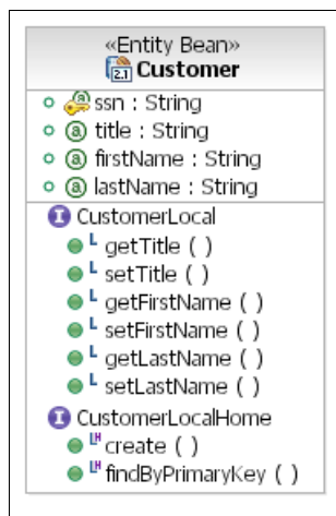
Figure 15-21 Class diagram with Customer entity bean
