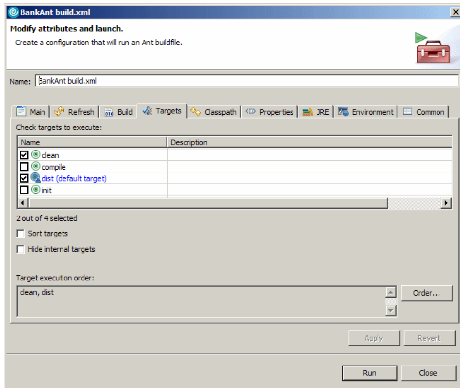
Figure 22-16 Launching Ant to generate complete build
