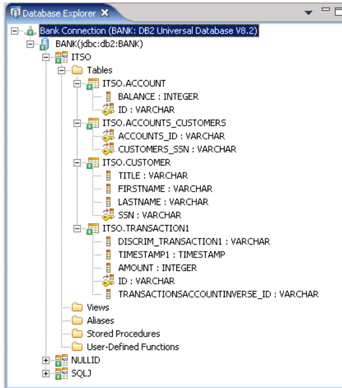
Figure 14-10 BANK database schema in the Database Explorer view
