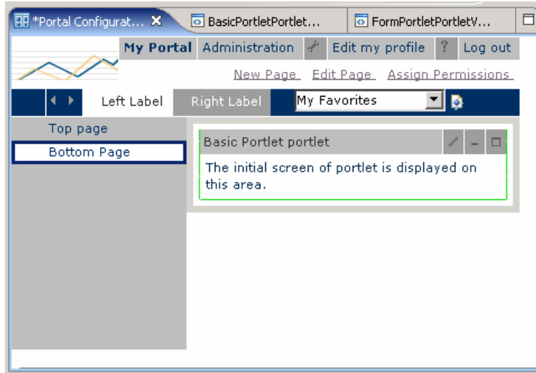
Figure 18-31 Basic portlet on the bottom page of the left label
