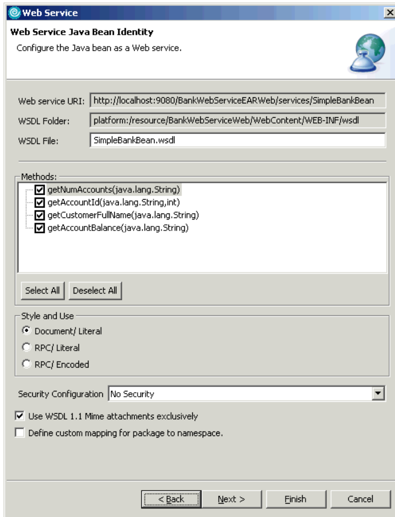
Figure 17-6 New Web Service wizard - Configure the Web Service
