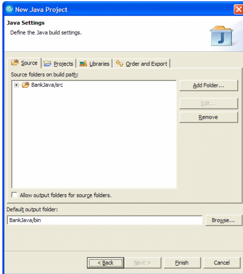
Figure 7-15 New Java project: Source settings
