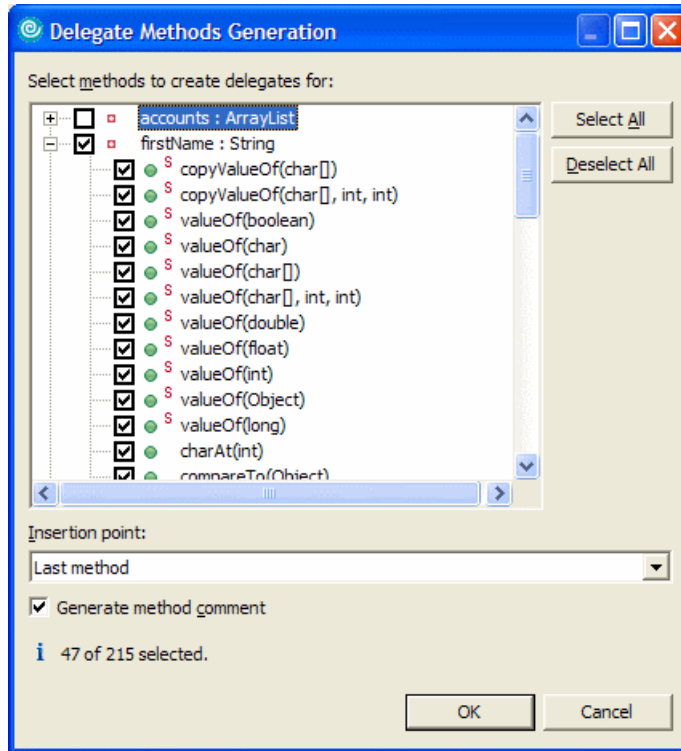
Figure 7-64 Java editor - Delegate Method Generator
