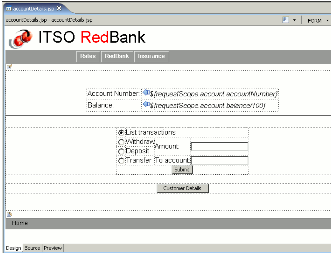
Figure 11-43 Completed accountDetails.jsp in the Design view
