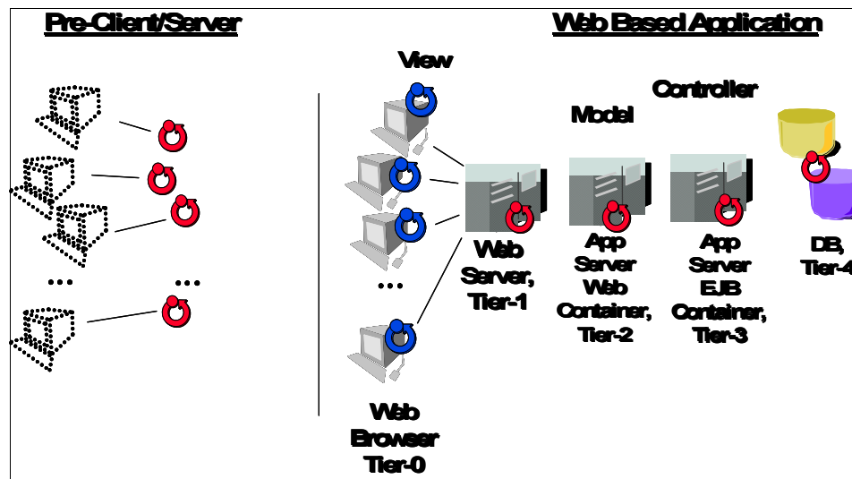
Figure 14-1 Architecture for a standard Web-based application
