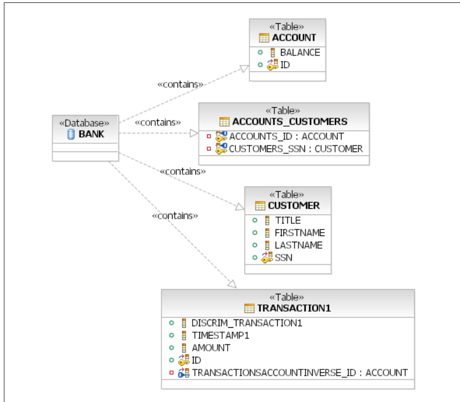
Figure 15-35 Existing relational model
