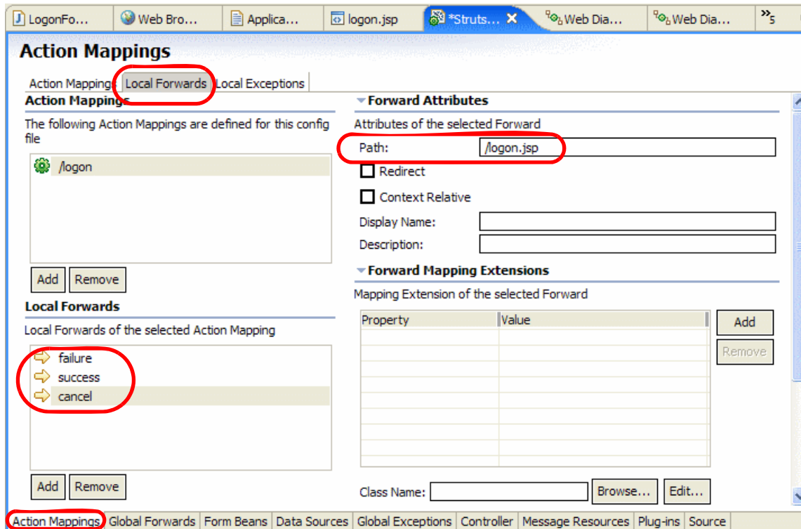
Figure 12-32 Struts Configuration Editor - Creating new forward
