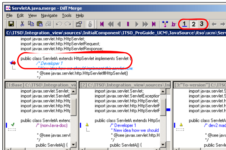
Figure 25-44 Diff Merge tool
