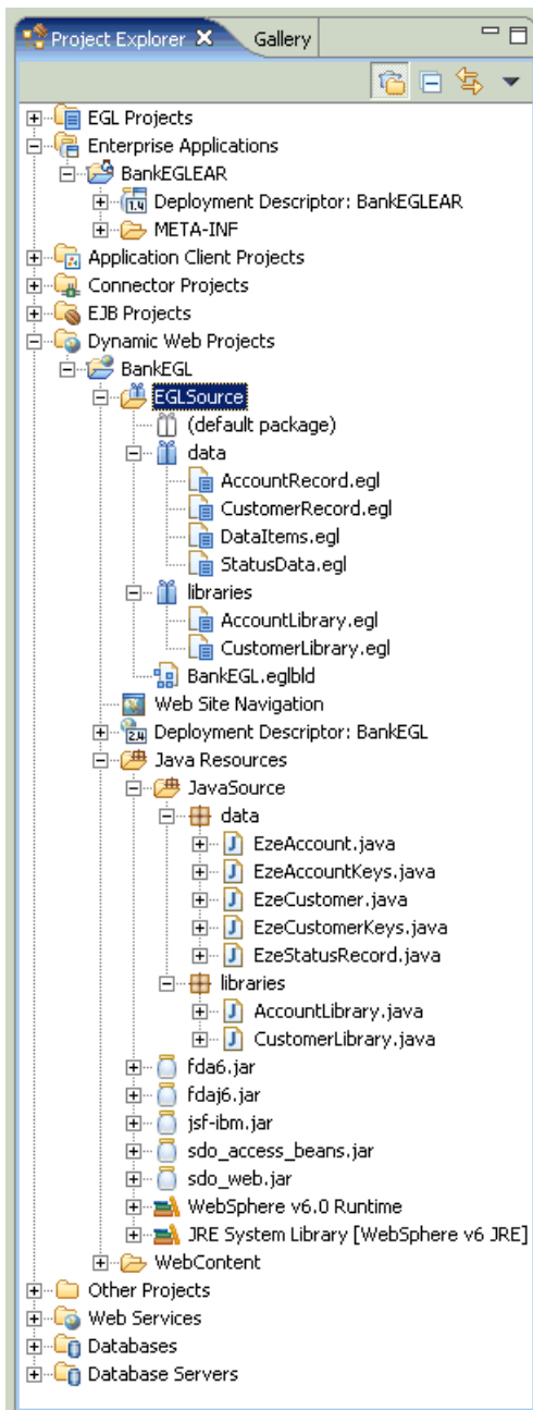
Figure 14-17 EGL and Java source files generated by the EGL Data Parts wizard
