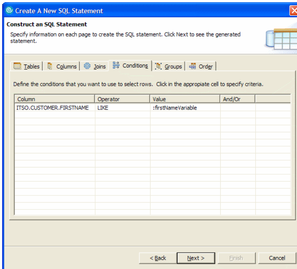
Figure 8-35 SQL Statement wizard - Construct an SQL Statement - Create conditions
