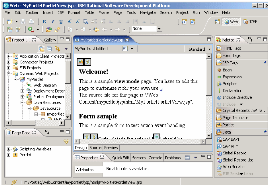
Figure 18-19 Page Designer showing the Design page
