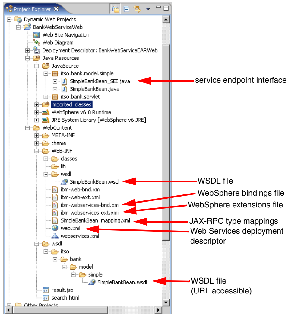
Figure 17-7 Web Services generated resources - Web project view
