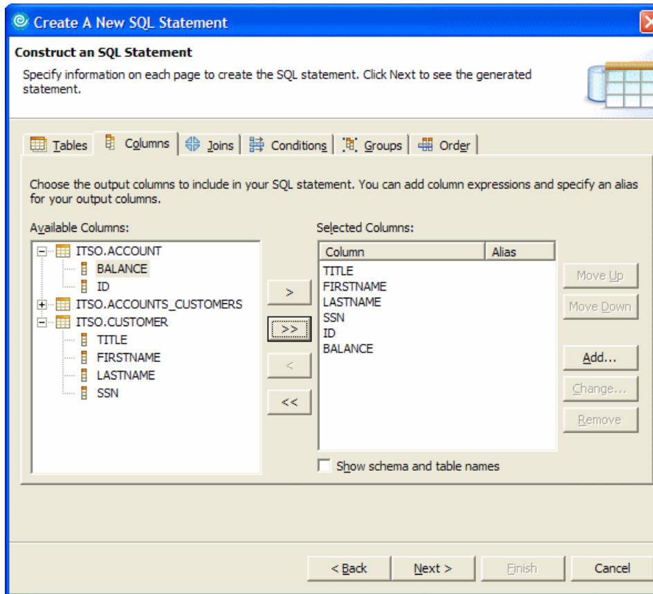
Figure 8-33 SQL Statement wizard - Construct an SQL Statement - Choose Columns
