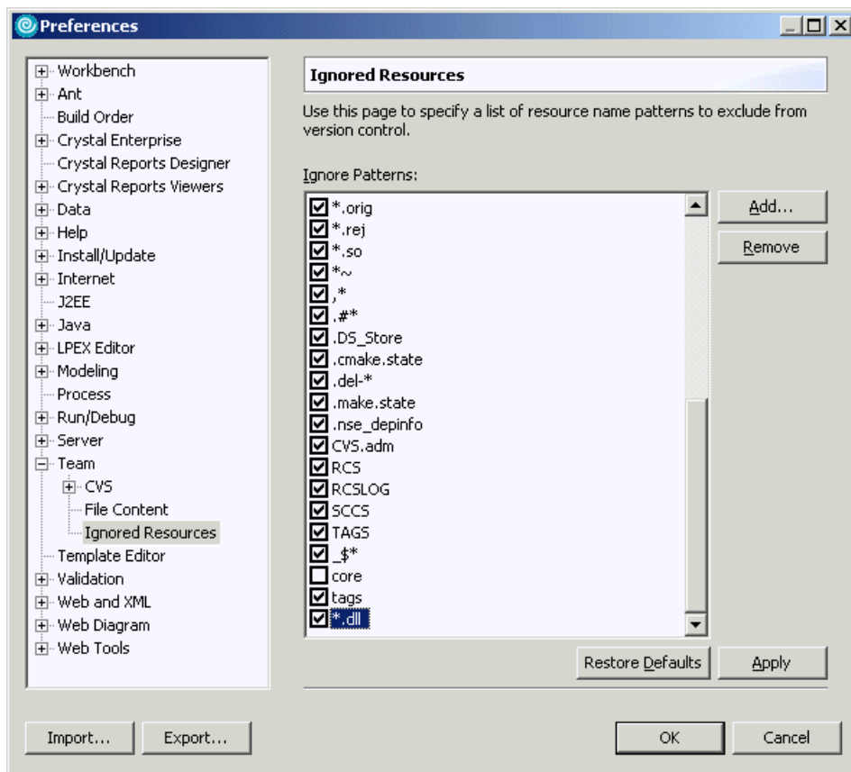
Figure 26-11 Resources that will be ignored when saving to the repository
