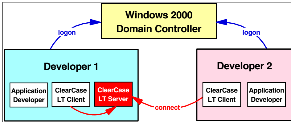
Figure 25-1 Sample ClearCase LT setup between two developers
