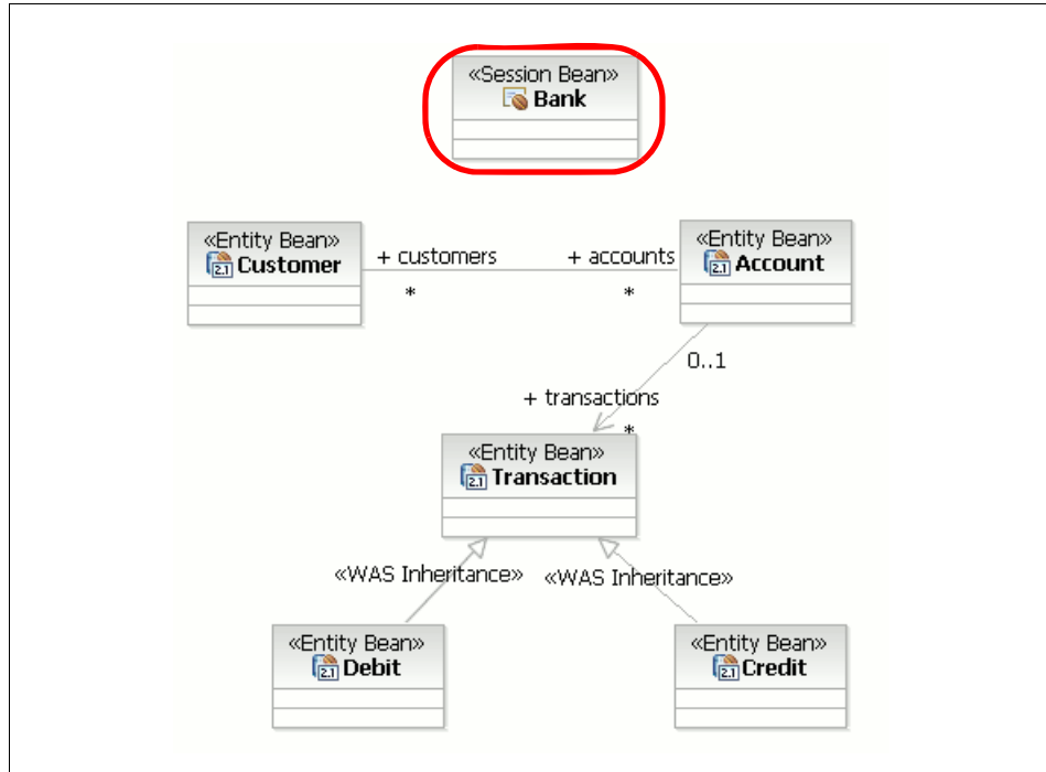
Figure 15-42 Business model session facade
