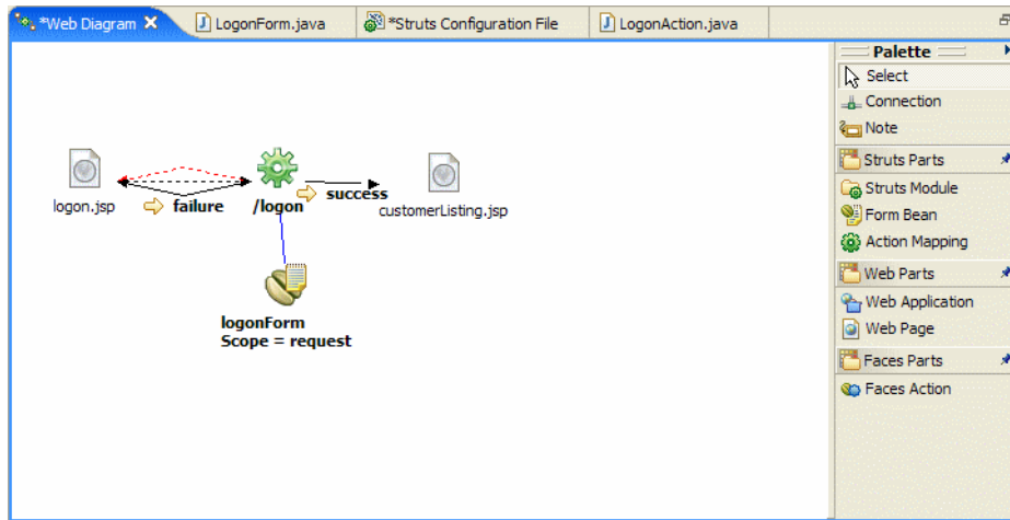
Figure 12-22 Realize Struts components - Logon action realized
