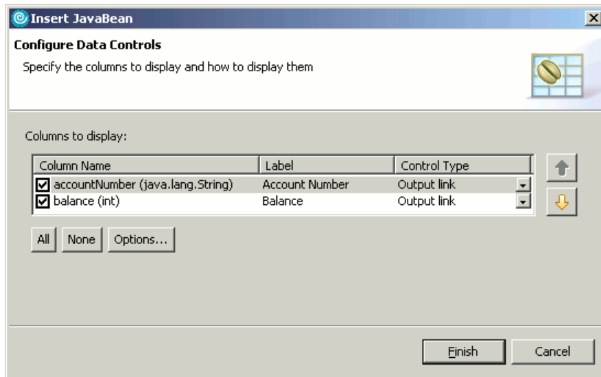
Figure 11-39 Inserting the accounts JavaBean
