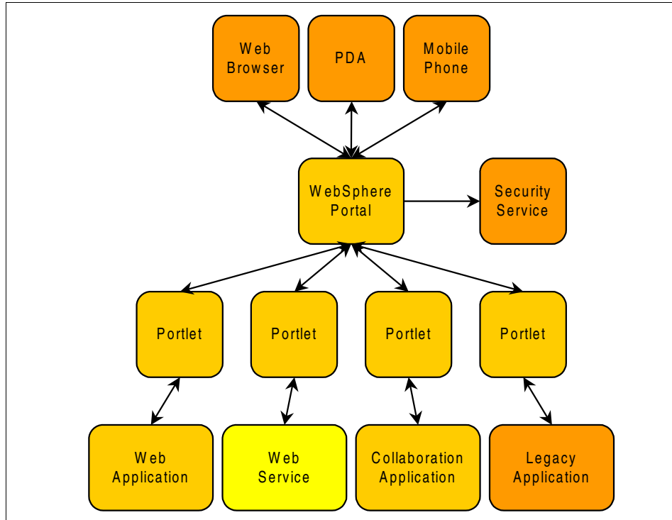
Figure 2-3 Portal applications
