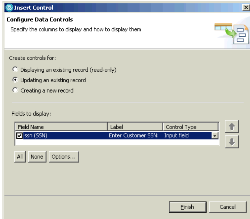
Figure 14-25 Insert Control
