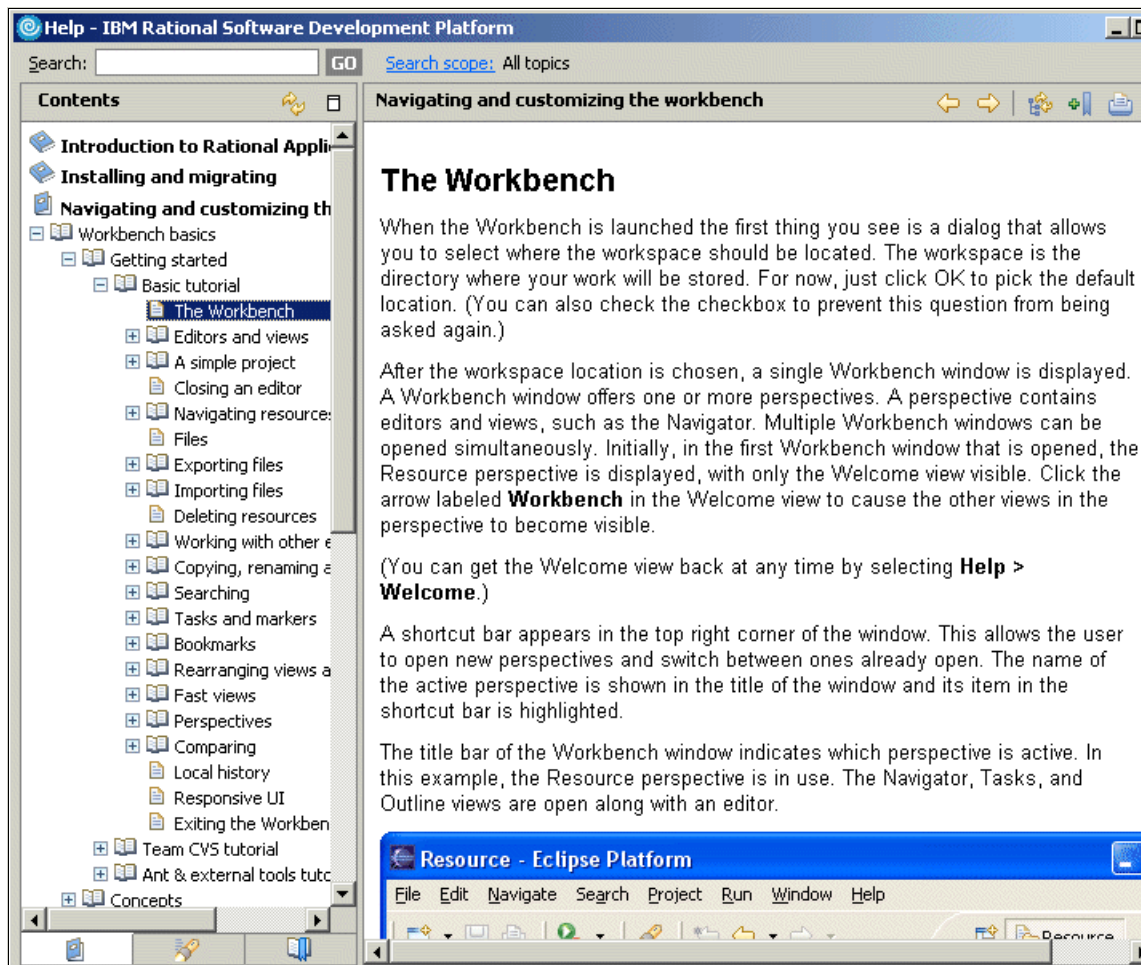
Figure 4-2 Workbench help
