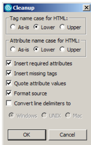
Figure 13-10 Cleanup dialog
