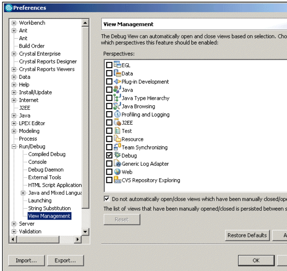
Figure 21-5 View Management
