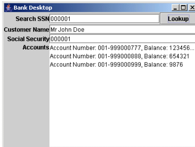
Figure 9-1 Sample GUI
