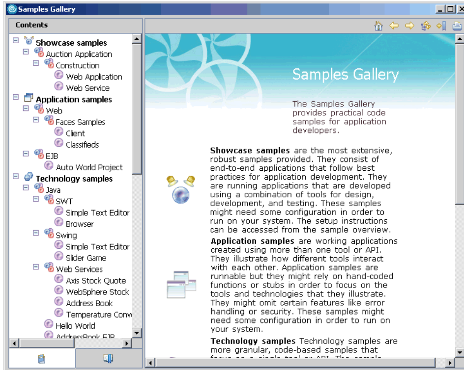
Figure 5-10 Samples Gallery
