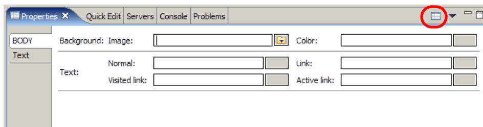
Figure 13-15 Properties view
