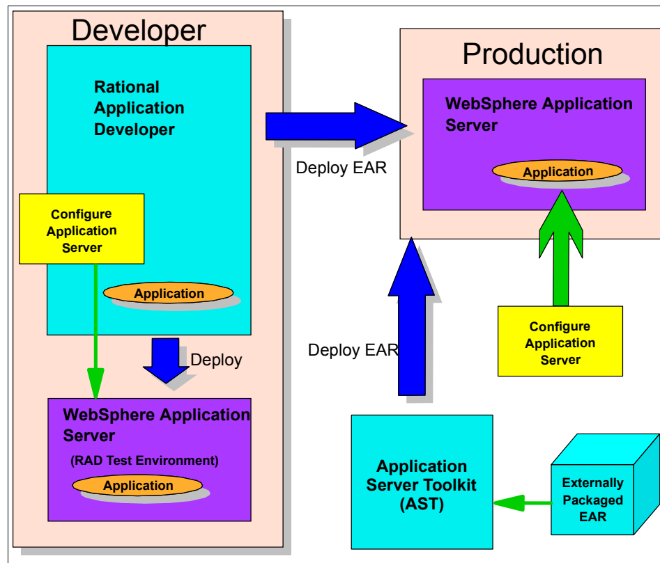
Figure 23-5 Deployment architecture
