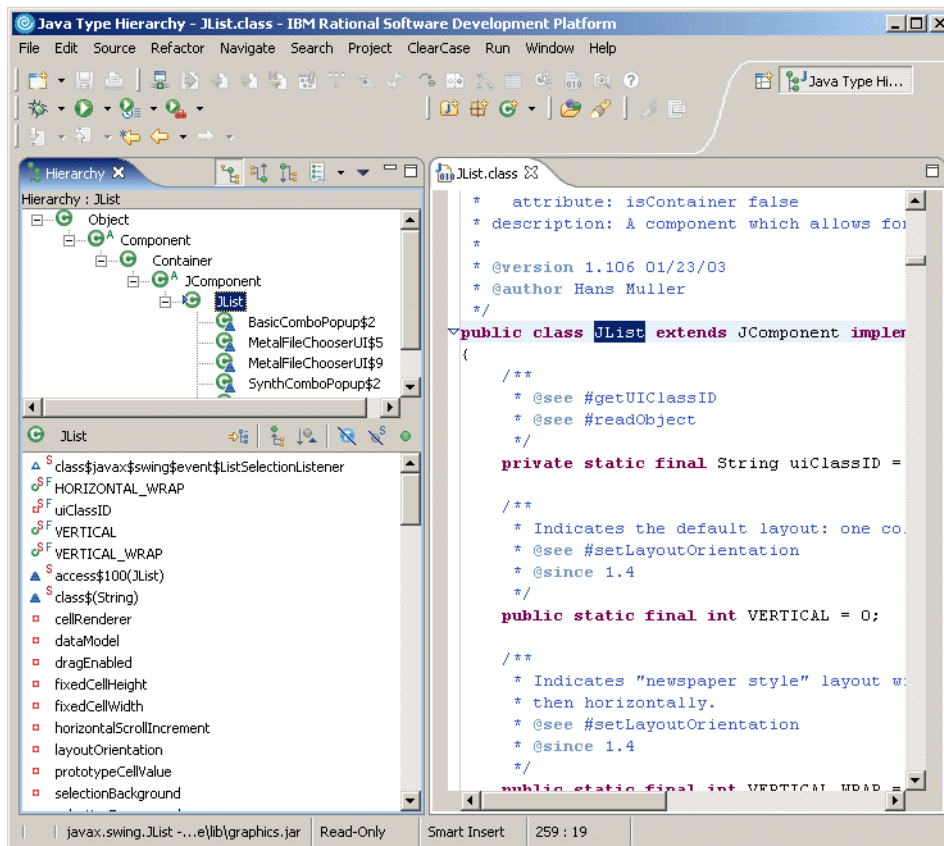
Figure 4-17 Hierarchy view
