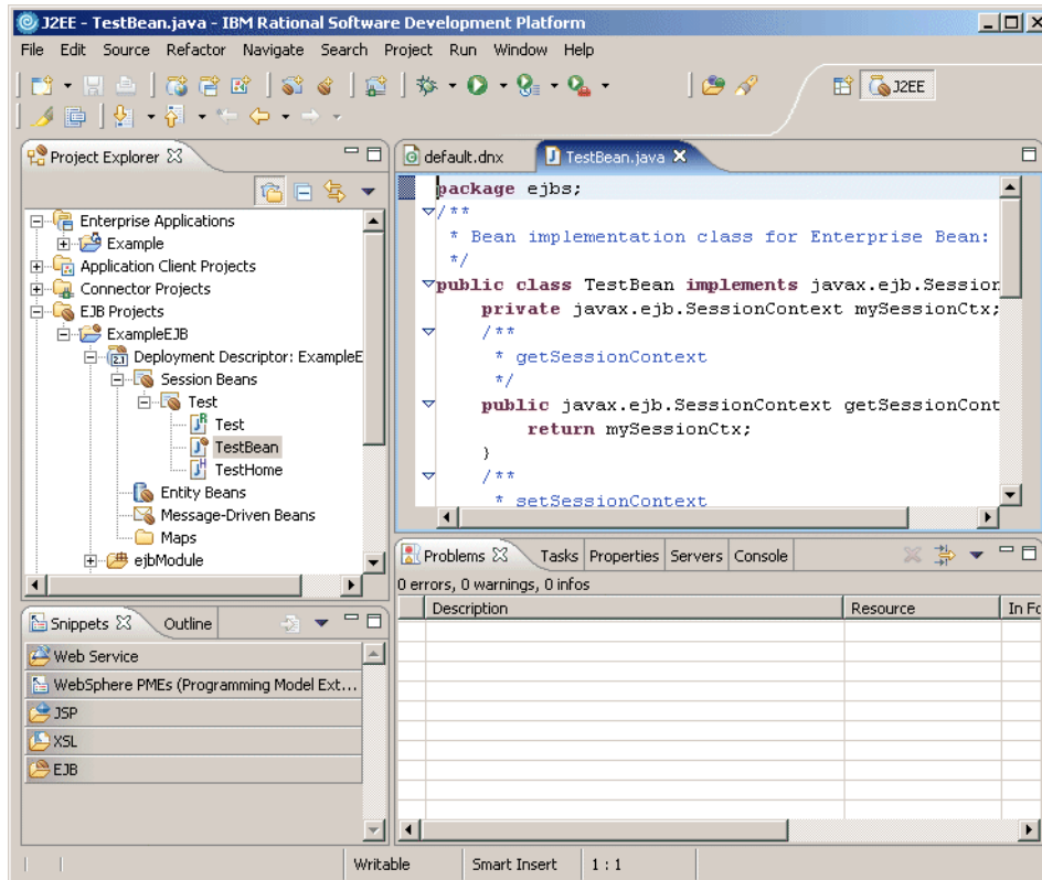
Figure 4-12 J2EE perspective
