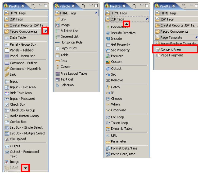
Figure 13-13 Palettes views
