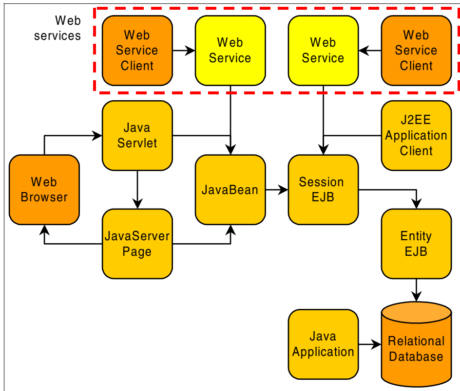
Figure 2-7 Web services
