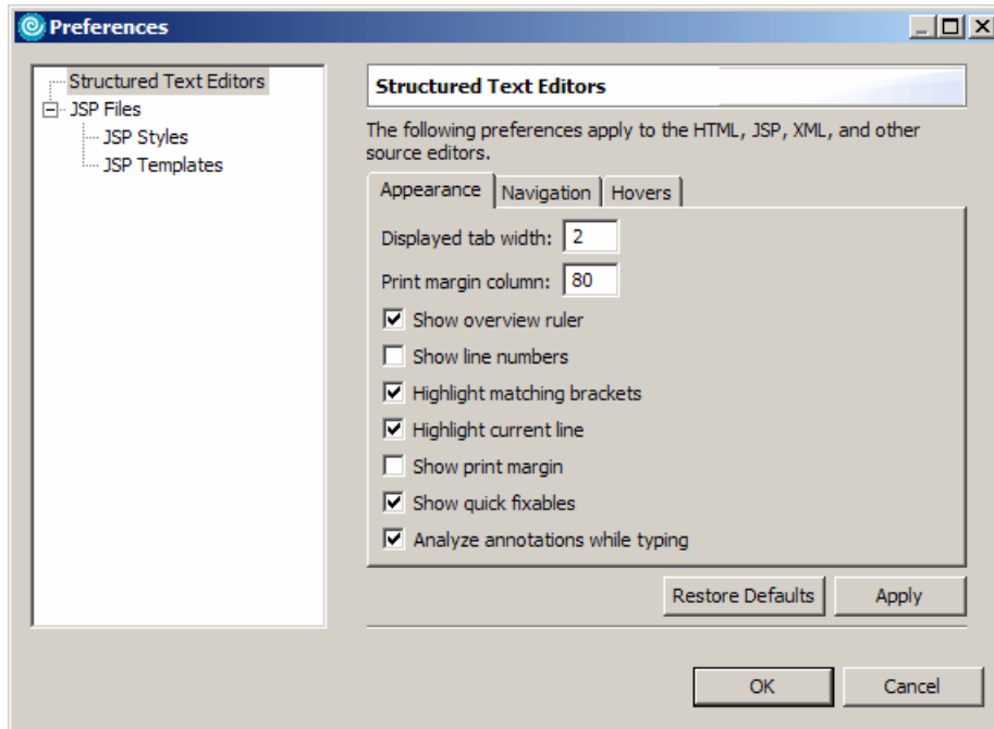
Figure 13-11 Preferences dialog
