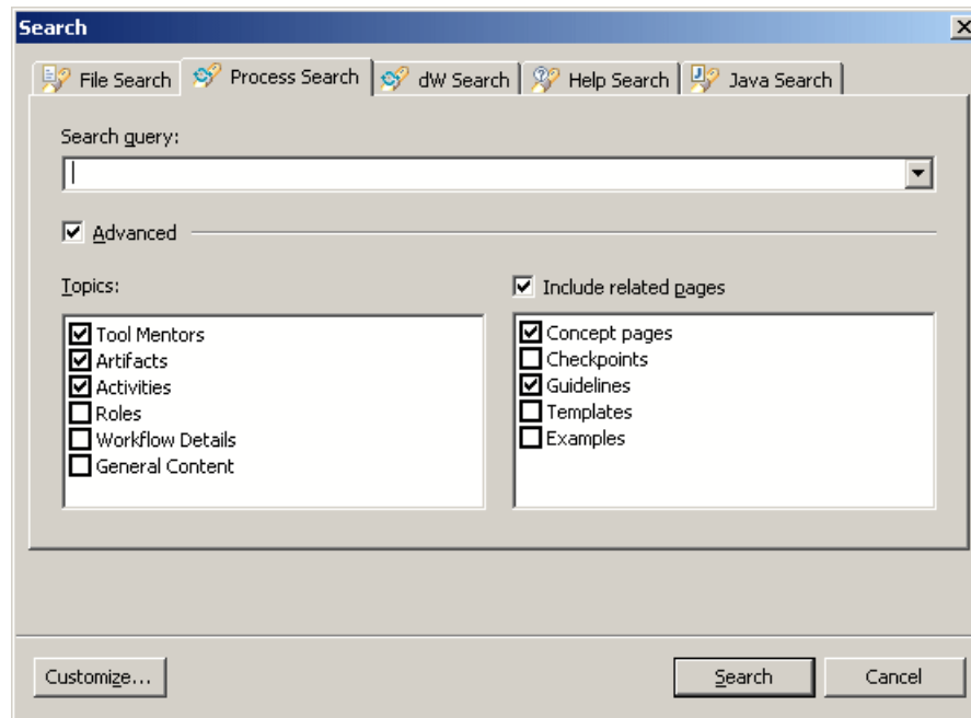
Figure 6-2 Process Search
