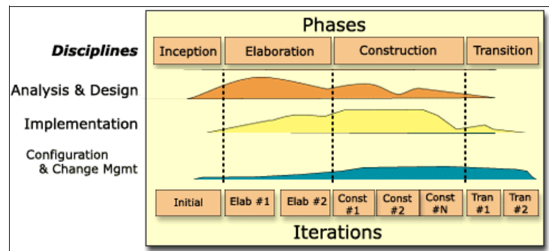
Figure 6-1 RUP overview
