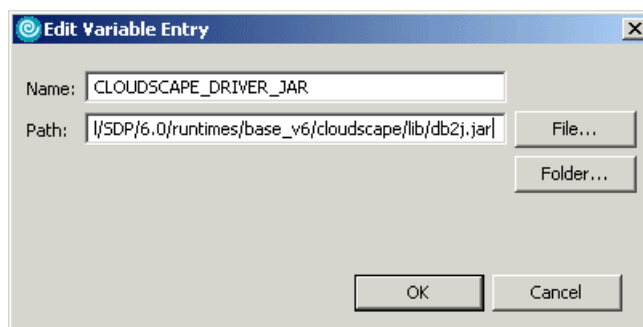
Figure 23-14 CLOUDSCAPE_DRIVER_JAR variable
