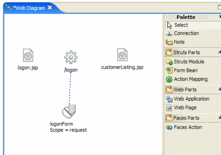
Figure 12-12 Struts components - Create Web pages
