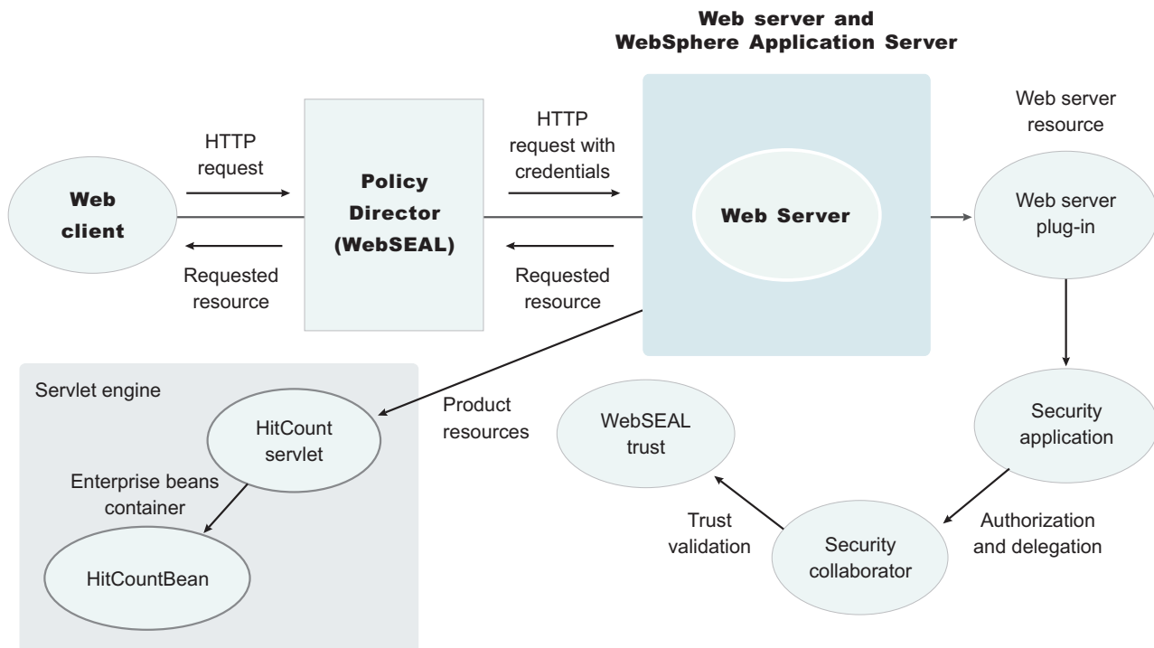
Figure 2. Figure 2. Policy director (WebSEAL server)
