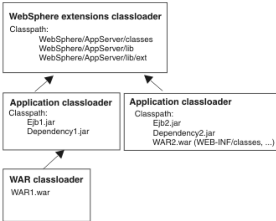
Figure 6. MULTIPLE classloader policy
