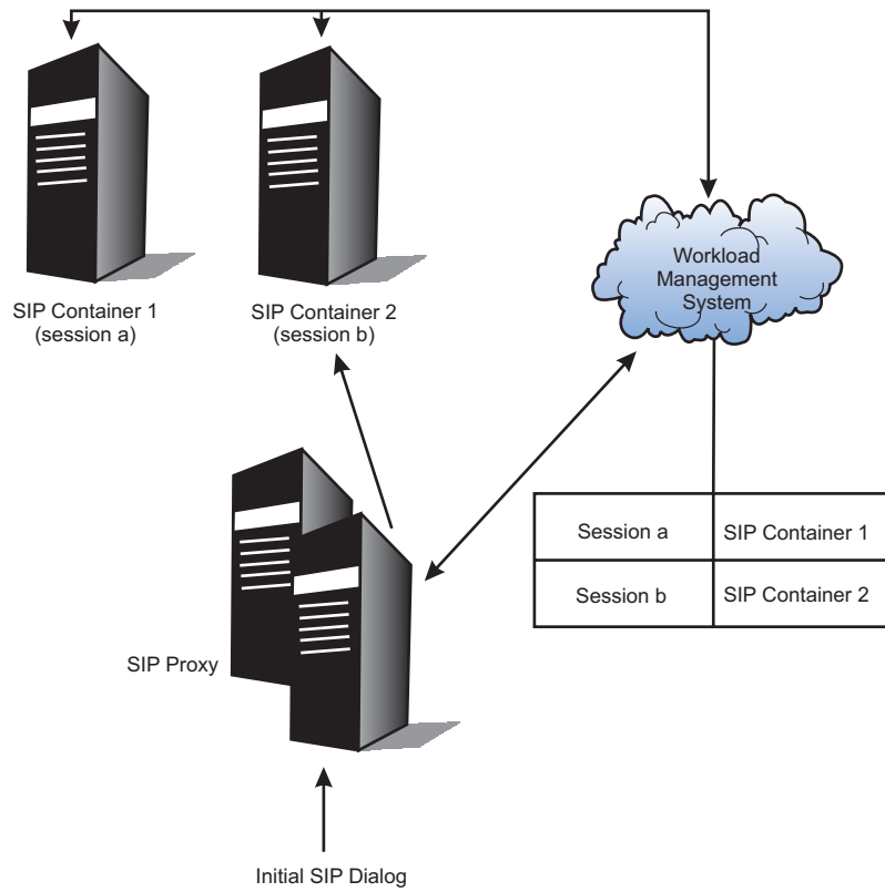
Figure 172. SIP Container Failover within a Cluster (Before)
