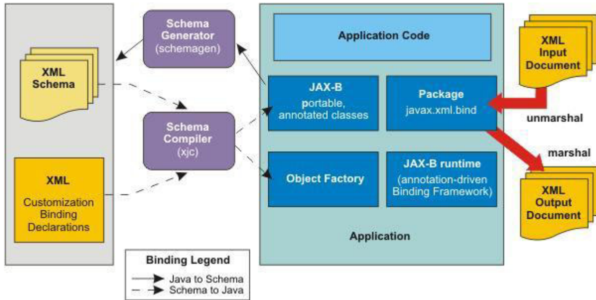
Figure 184. JAXB architecture
