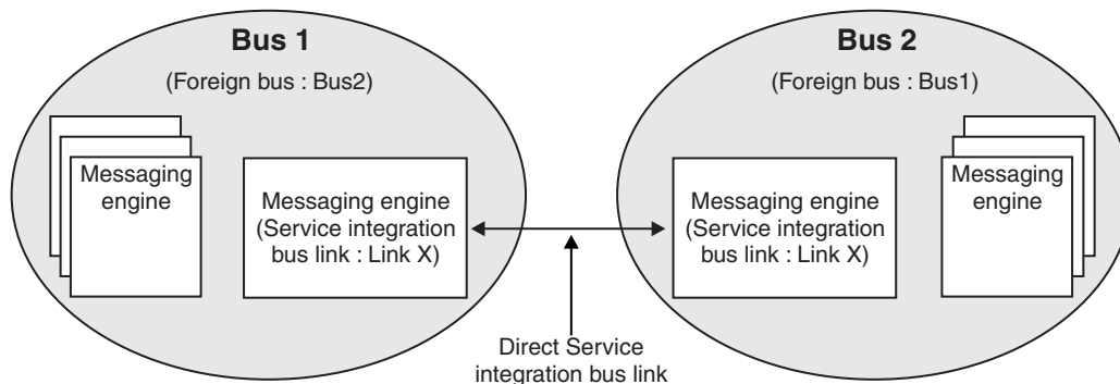
Figure 168. Direct connection between two service integration buses by using a service integration bus link
