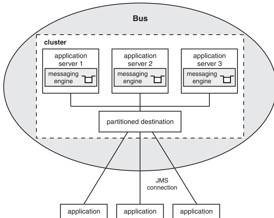
Figure 153. Service integration bus with partitioned destinations
