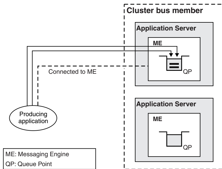
Figure 113. Default behavior: messages are sent to the local queue point
