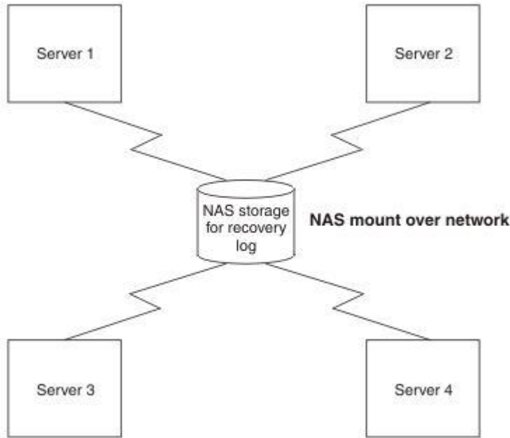
Figure 27. Recovery logs on NAS storage are available to all servers
