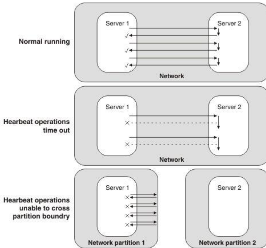
Figure 181. Heartbeats in a system running normally, compared to heartbeats after the apparent server failures of system overloading and network partitioning
