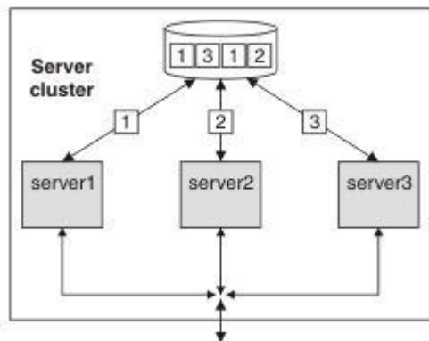
Figure 176. Server cluster up and running, just before server failure
