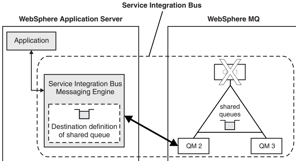
Figure 81. A messaging engine connecting to a second queue manager to access a queue sharing group, after the original queue manger it was using failed
