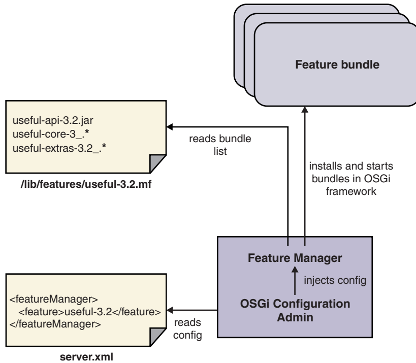
Figure 31. Feature management
