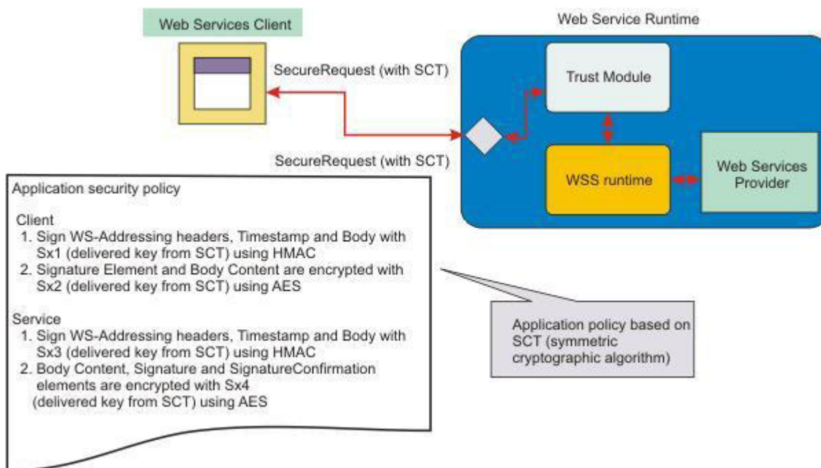
Figure 25. Securing application messages with keys derived from secret of the security context token
