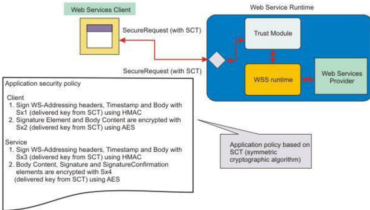
Figure 24. Securing application messages with keys derived from secret of the security context token
