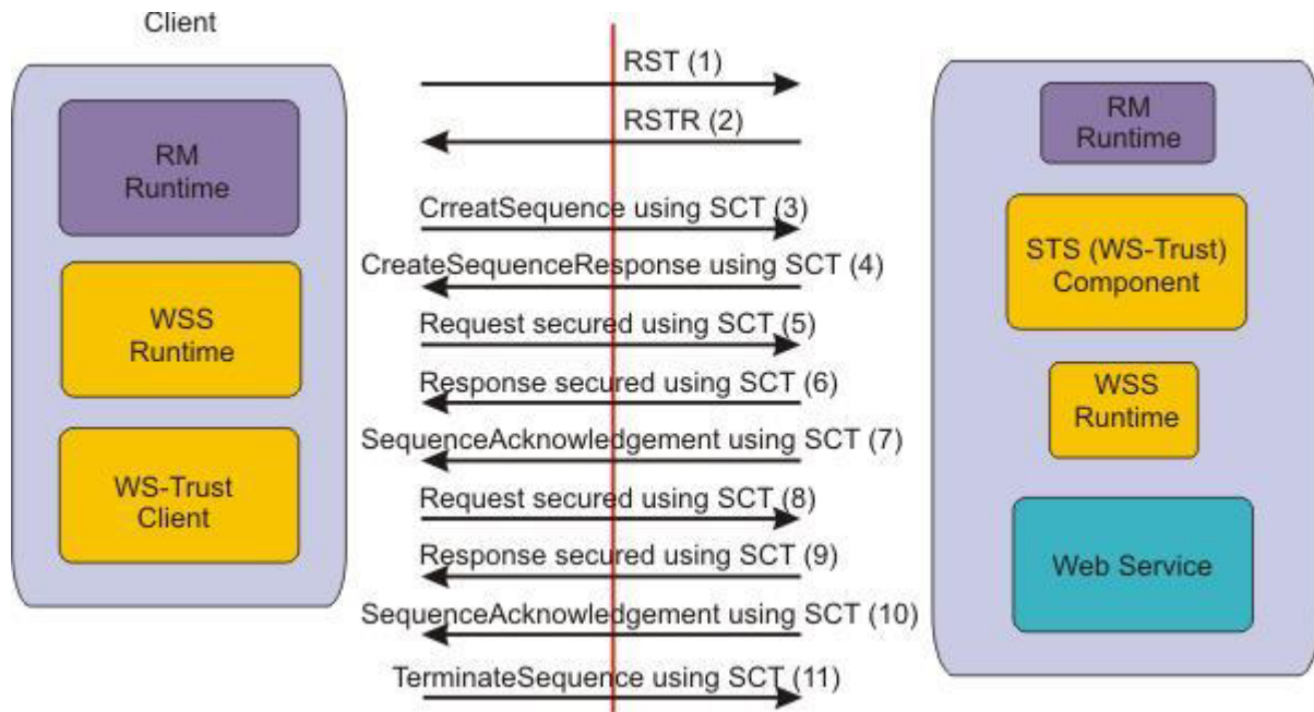
Figure 25. Messages exchange for the SCT and reliable messaging
