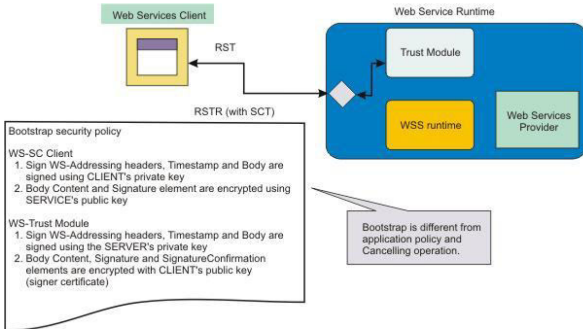
Figure 53. Using WS-Trust protocols RST and RSTR to establish the SCT between the initiator and the recipient
