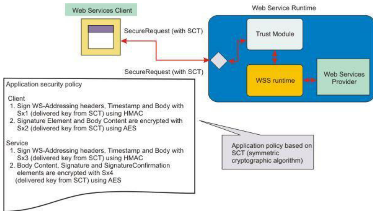
Figure 54. Securing application messages with keys derived from secret of the security context token
