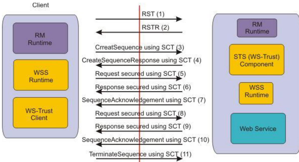
Figure 55. Messages exchange for the SCT and reliable messaging
