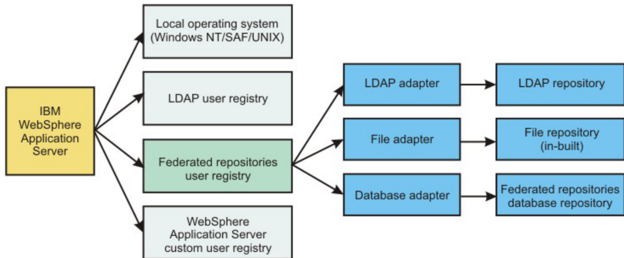
Figure 5. Configuring a federated repository user registry without the user registry bridge
