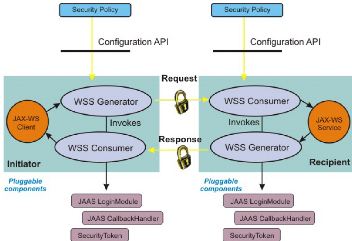
Figure 20. Pluggable token architecture using the JAX-WS programming model
