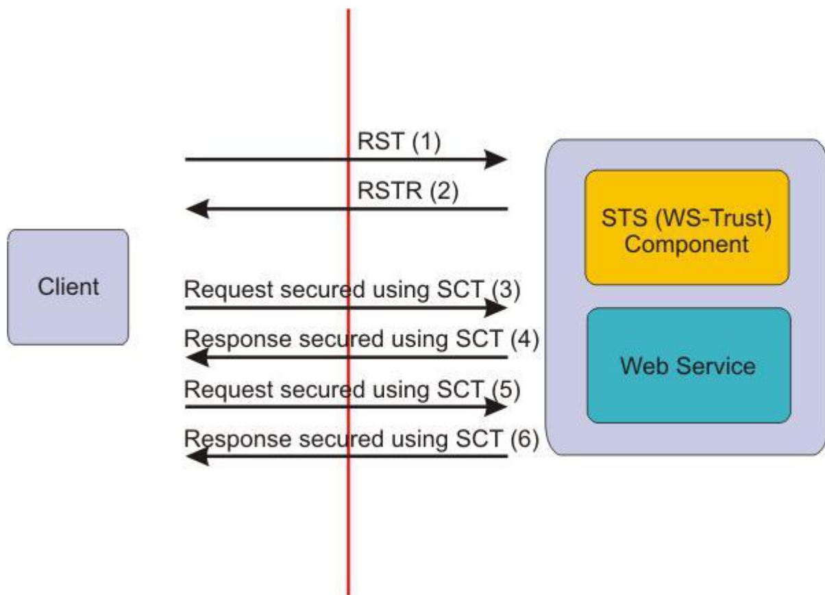
Figure 23. Displaying the flow between the client and the Web service and security token service
