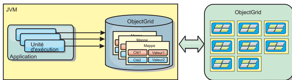
Figure 43. Cache local
