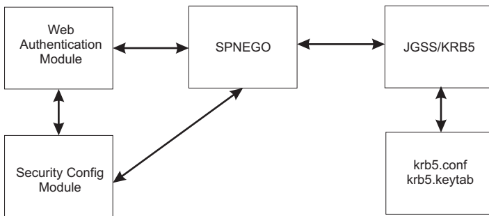
Figure 13. SPNEGO web authentication and security configuration elements
