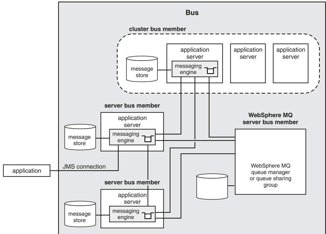
Figure 58. Bus members
