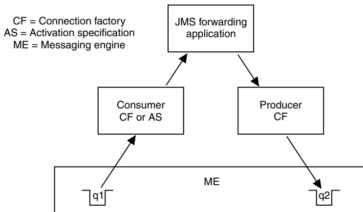
Figure 17. Forwarding messages
