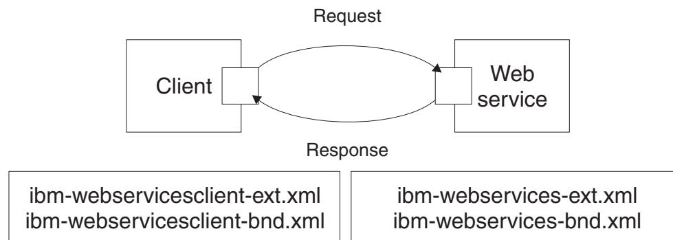
Figure 104. Message flows
