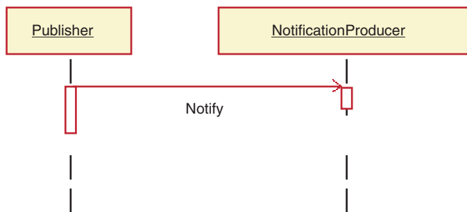
Figure 106. Simple publishing
