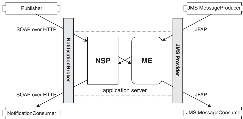
Figure 113. Example of the message paths from a publisher and a JMS MessageProducer
