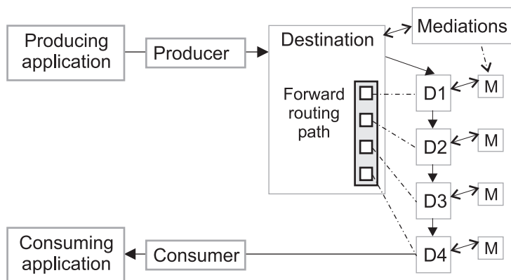
Figure 66. Routing paths
