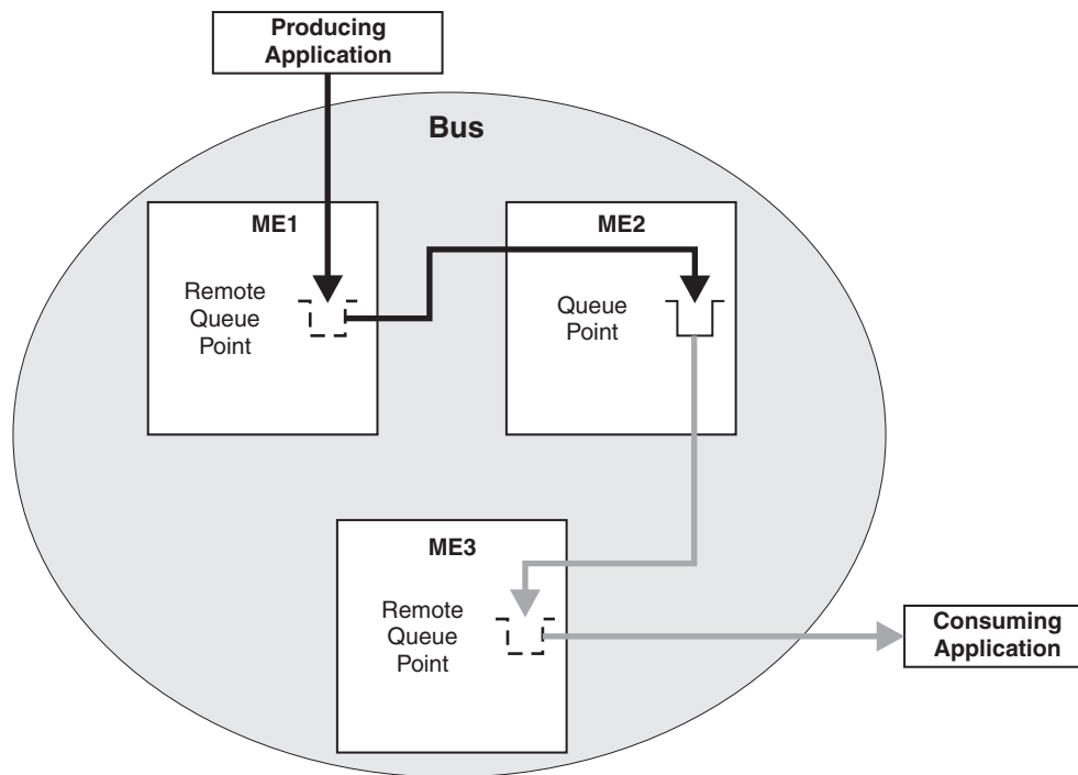
Figure 67. Point-to-point message production and consumption by using remote queue points.
