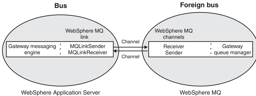
Figure 39. Exchanging messages between WebSphere MQ link sender and receiver channels, and a gateway queue manager with receiver and sender channels.
