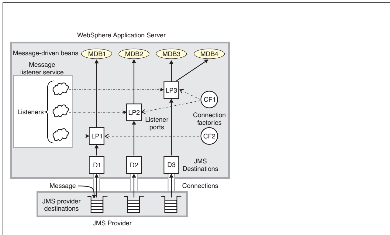
Figure 10. The main components for message-driven beans
