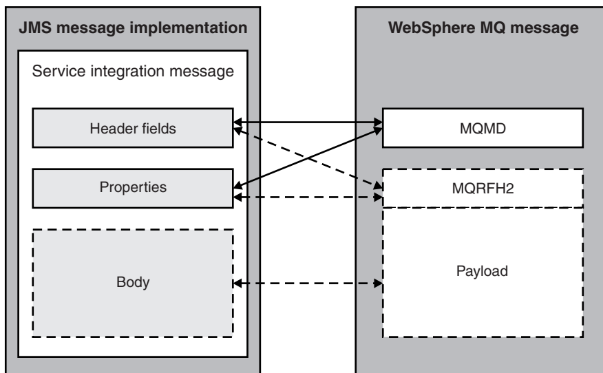
Figure 27. Message conversion to and from WebSphere MQ format
