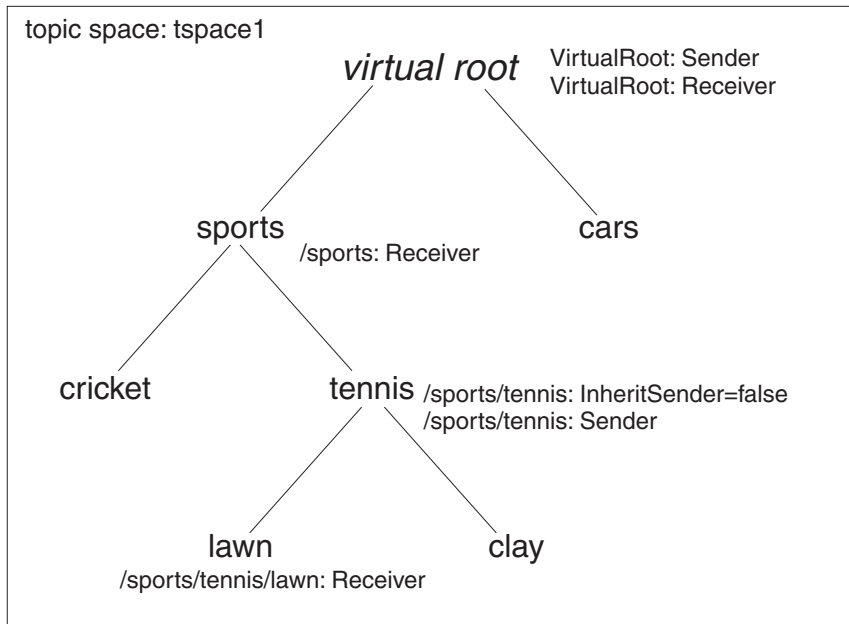
Figure 72. Example of a topic space with topic-level authorization
