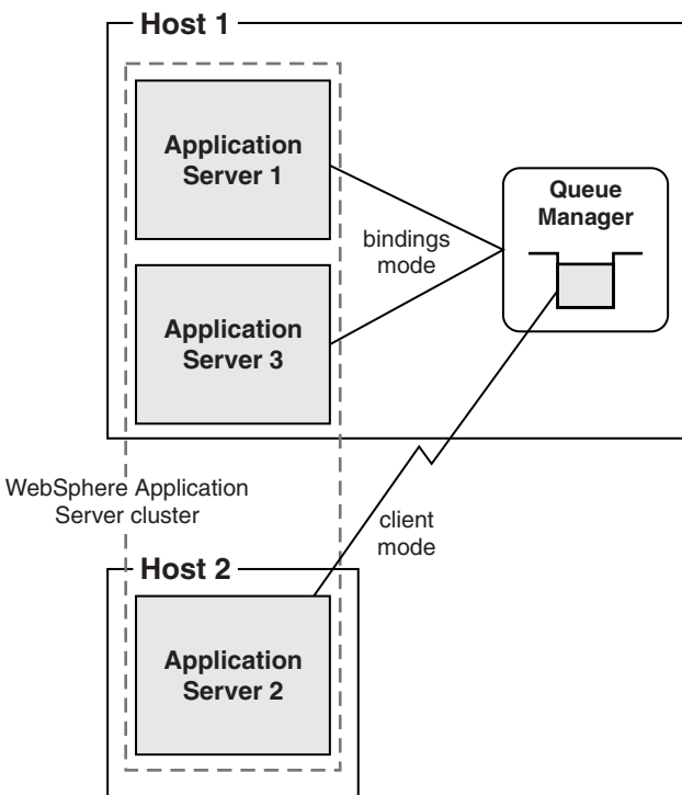
Figure 21. WebSphere Application Server clustering: bindings then client mode attachment to queue manager
