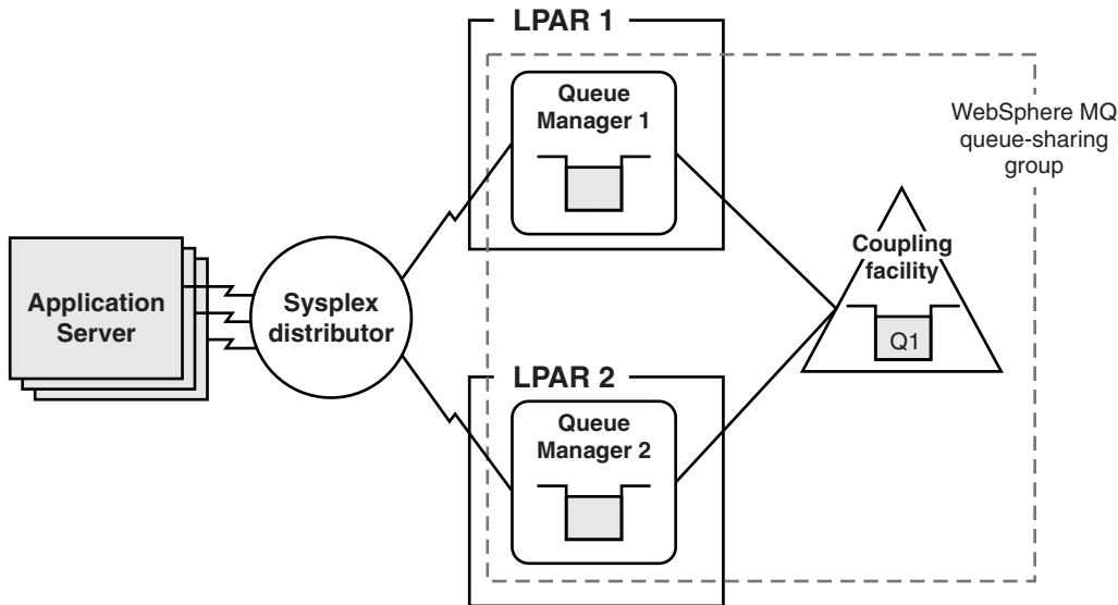
Figure 25. WebSphere Application Server with client mode connection to WebSphere MQ for z/OS
