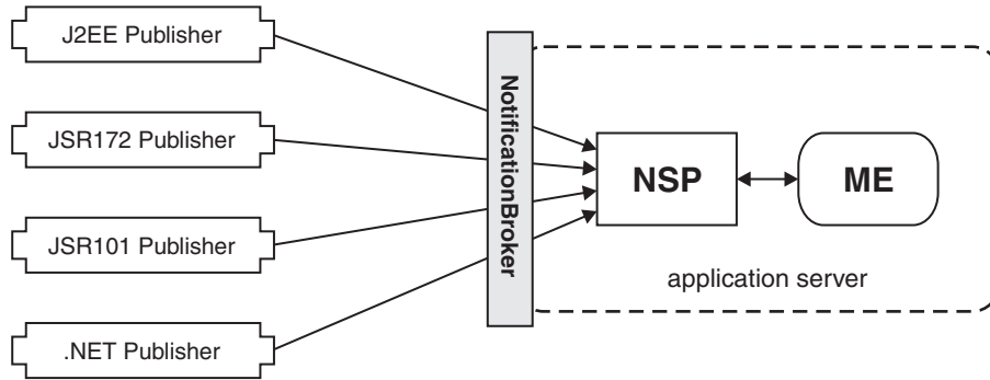
Figure 111. Example of the variety of clients that can connect to the notification broker
