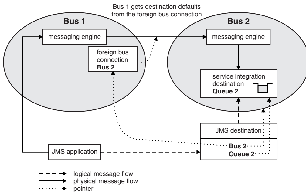
Figure 63. Point-to-point messaging between two buses with no foreign destination configured
