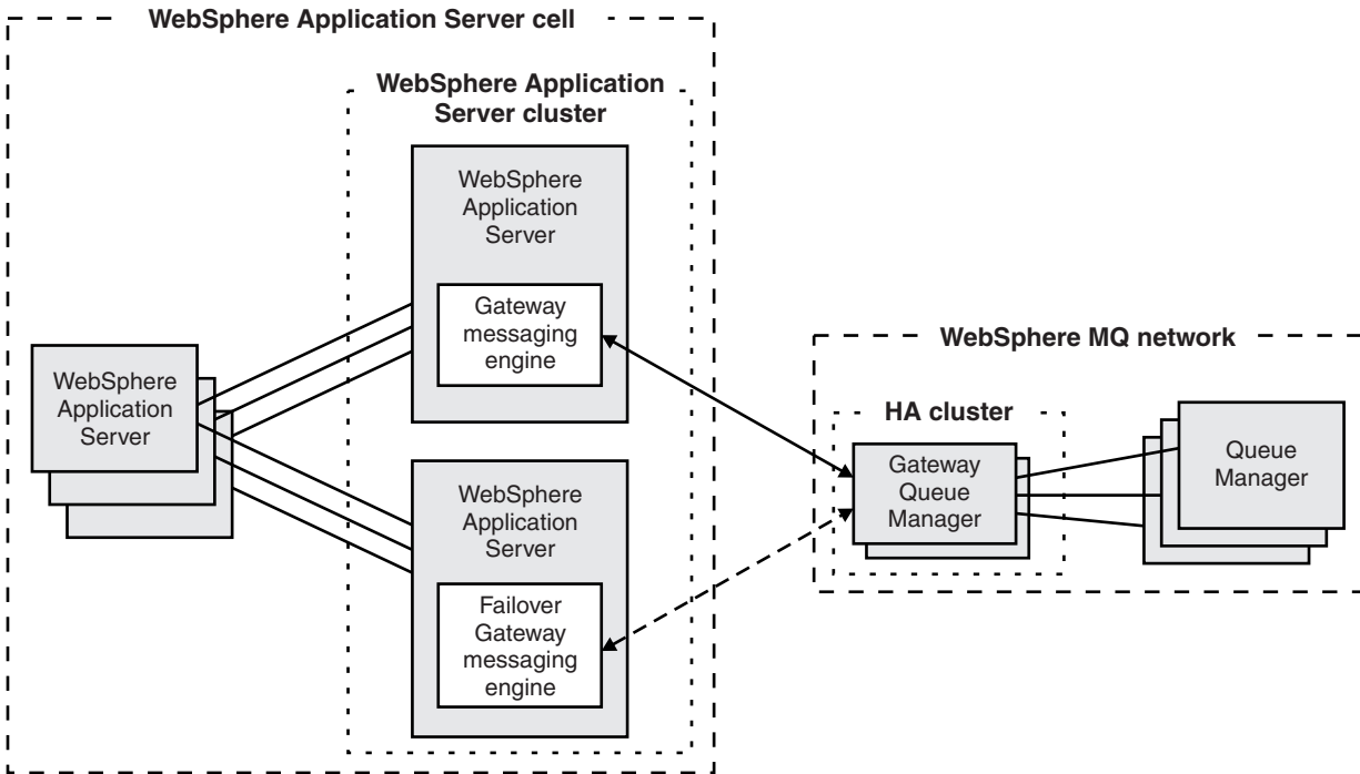
Figure 32. High availability for multiple application servers connected to multiple queue managers
