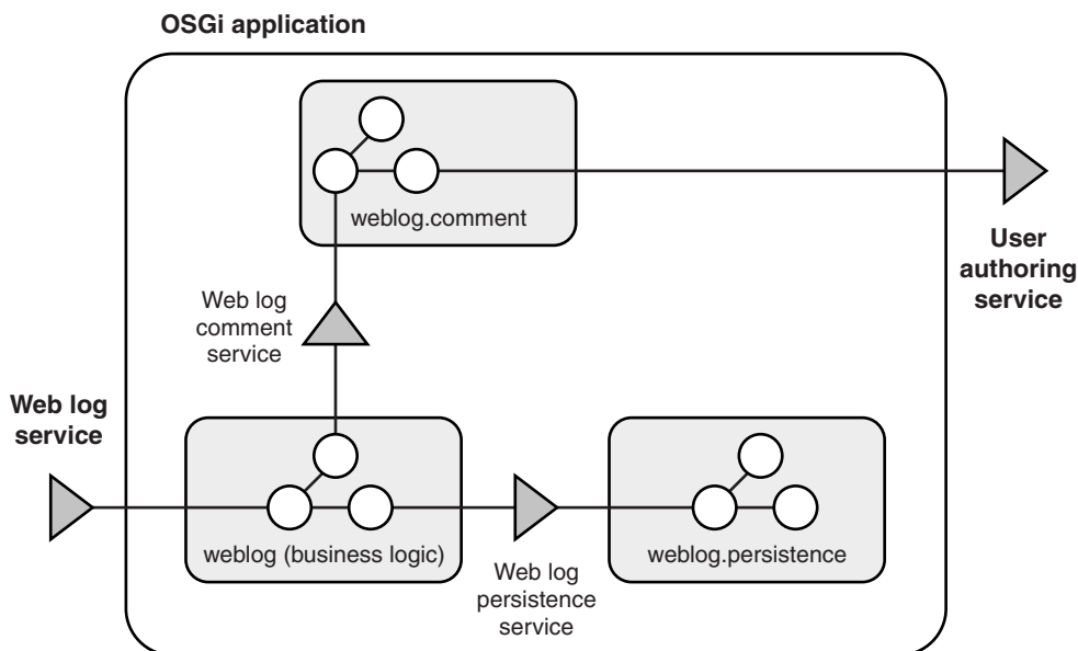
Figure 54. Bundles and services in an example application for a weblog service
