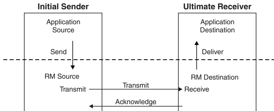
Figure 100. The interactions used to exchange web services messages reliably.
