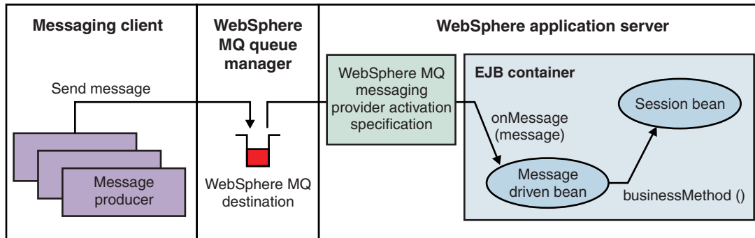
Figure 26. WebSphere MQ messaging provider activation specification in action
