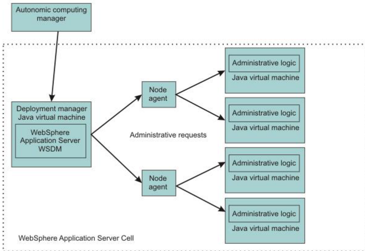
Figure 98. WSDM application in a WebSphere Application Server, Network Deployment cell
