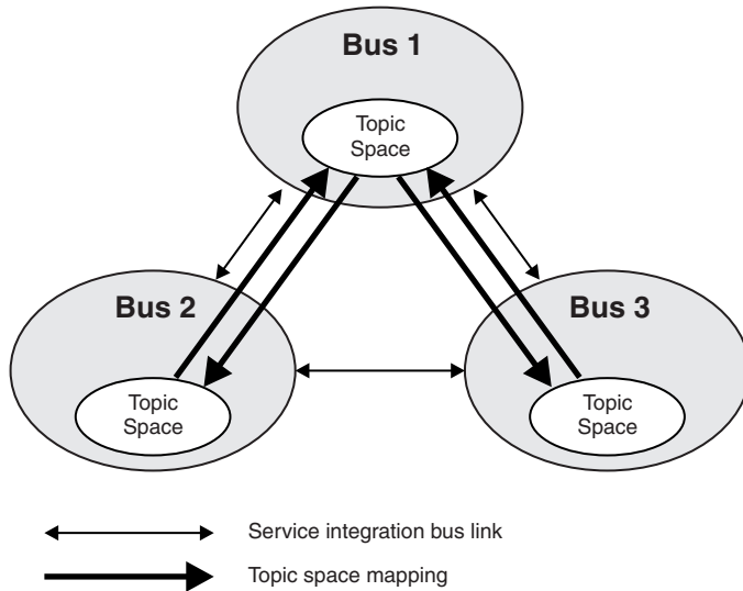
Figure 85. Network of buses with topic space mappings in both directions
