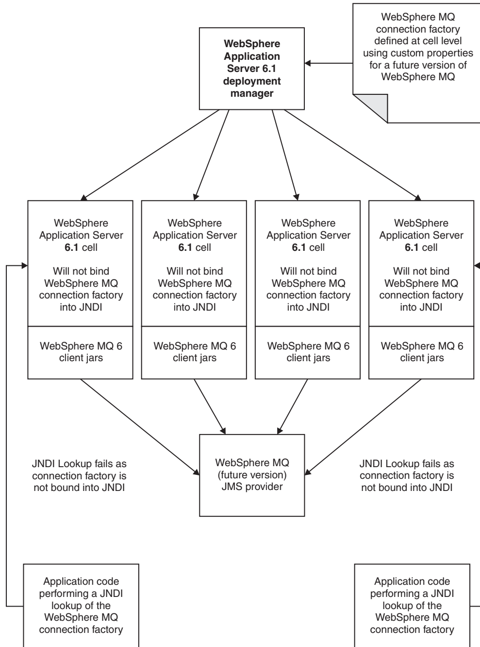
Figure 9. Future version of WebSphere MQ scenario
