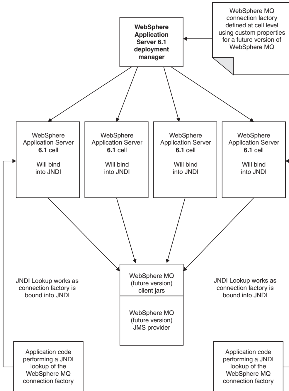
Figure 10. Correctly configured scenario
