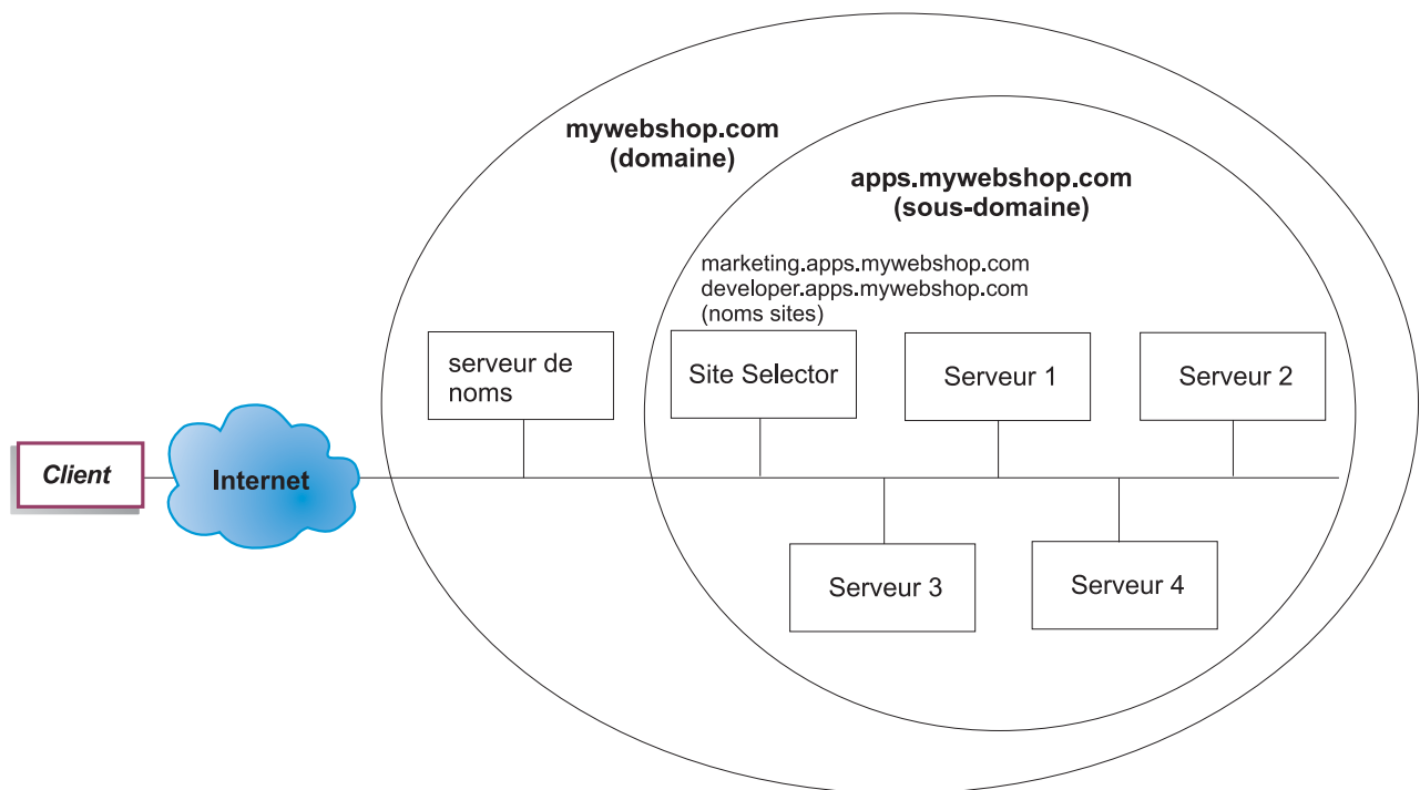
Figure 23. Configuration Site Selector simple
