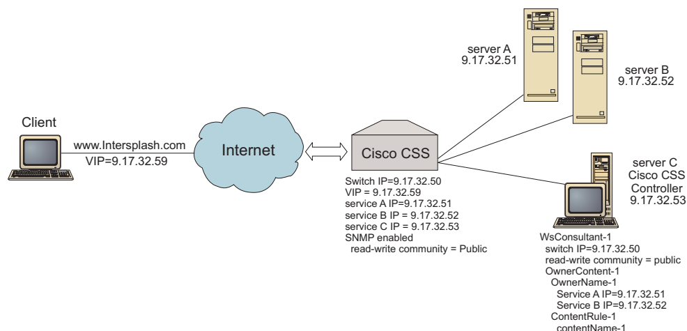
Figure 25. Configuration Cisco CSS Controller simple
