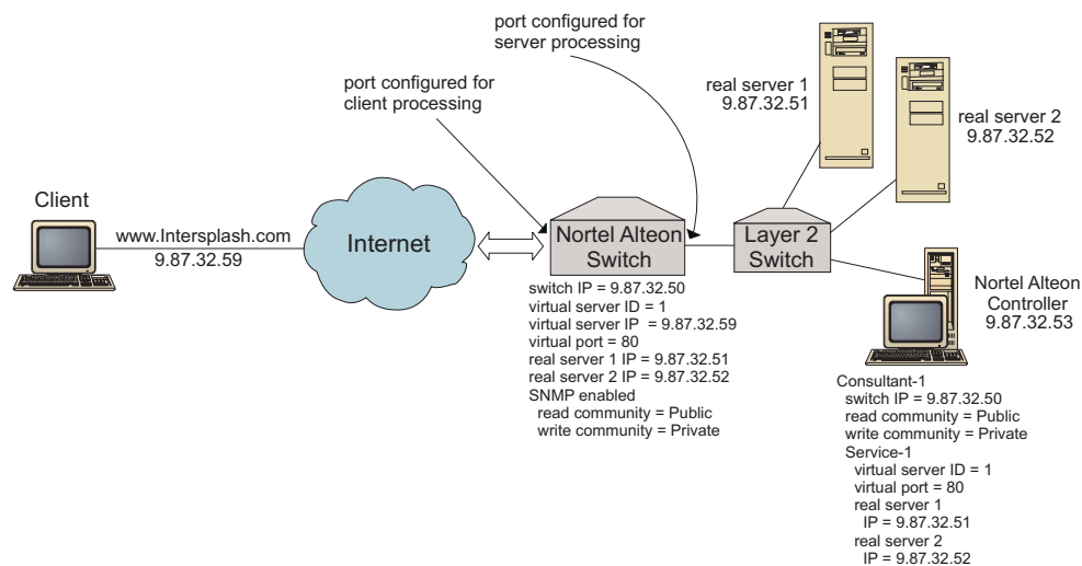
Figure 28. Configuration Nortel Alteon Controller simple
