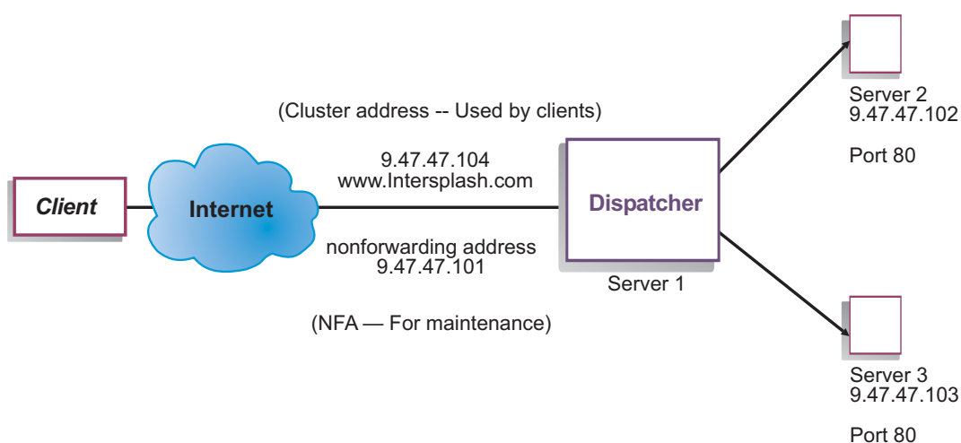
Figure 8. Configuration Dispatcher locale simple
