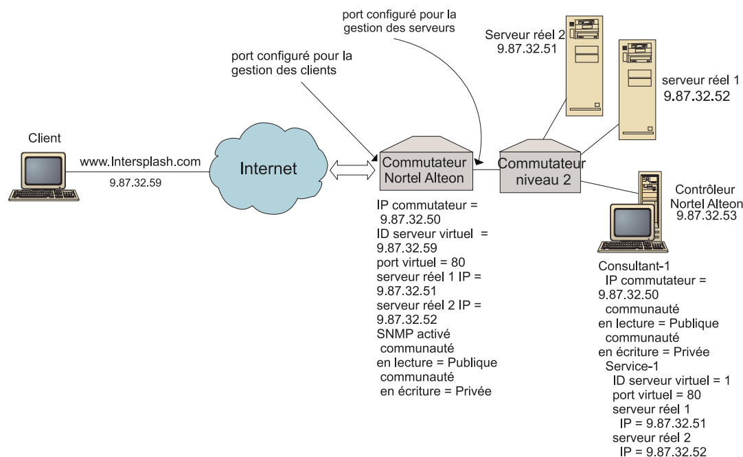
Figure 28. Configuration Nortel Alteon Controller simple
