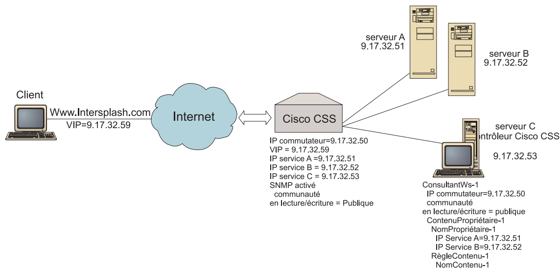
Figure 25. Configuration Cisco CSS Controller simple
