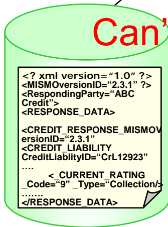
File System
