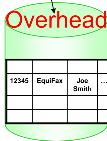
Shredded (Oracle)
