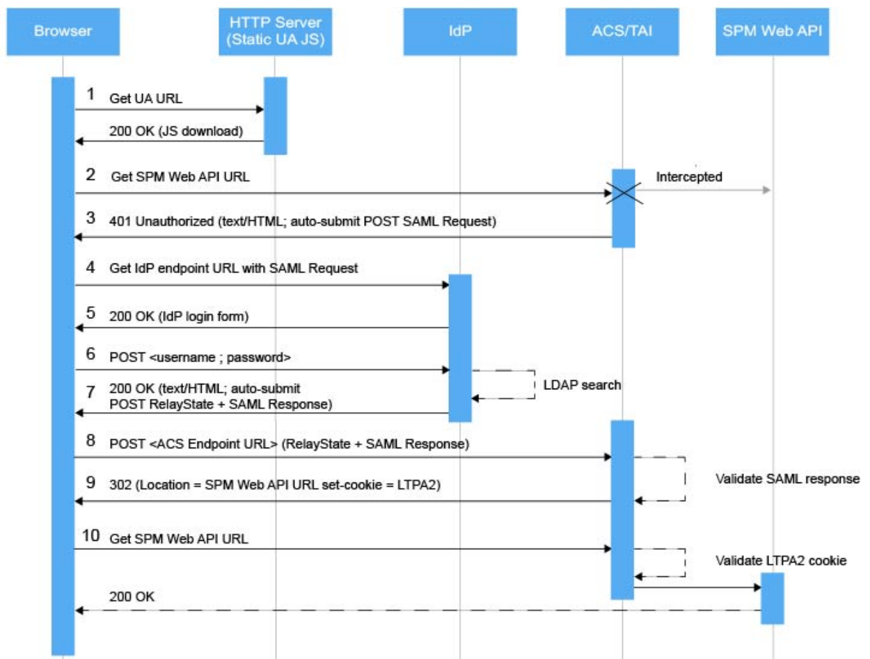
Figure 4. SP-initiated flow in Universal Access
