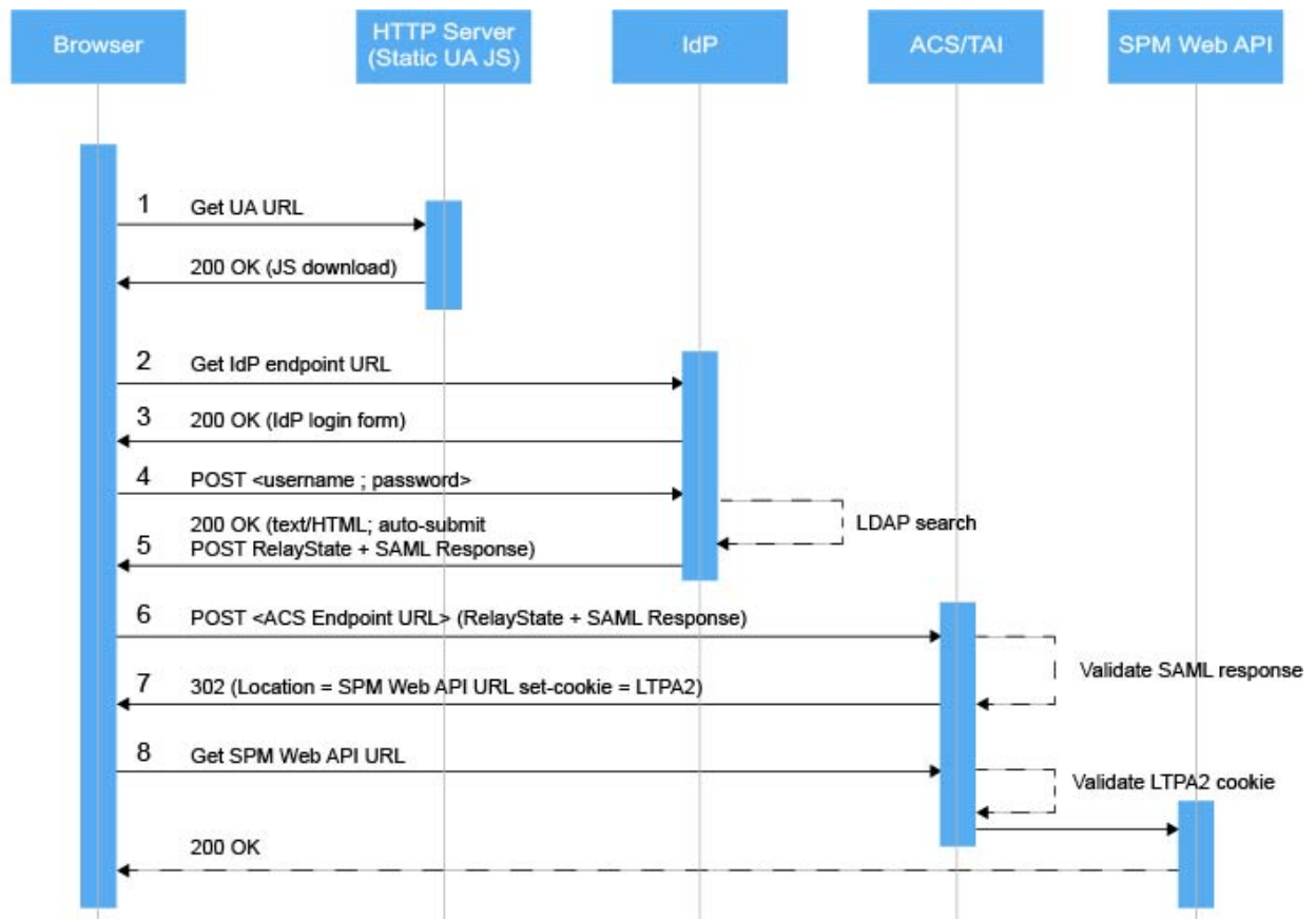
Figure 3. IdP-initiated flow in Universal Access
