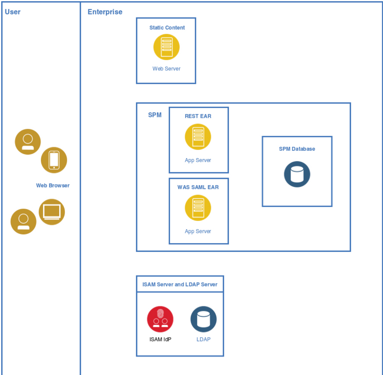
Figure 6. Universal Access SSO configuration components
