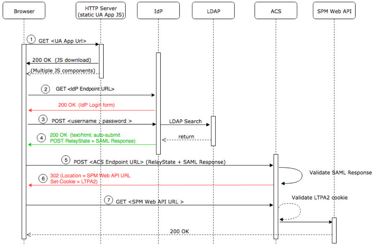
Figure 2: IdP initiated flow in IBM Cúram Universal Access
