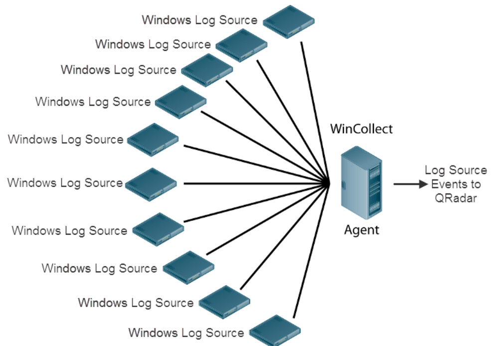
Figure 7-1 A single WinCollect agent configured for remote collection.
