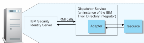
Figure 1. The architecture of the CyberArk adapter
