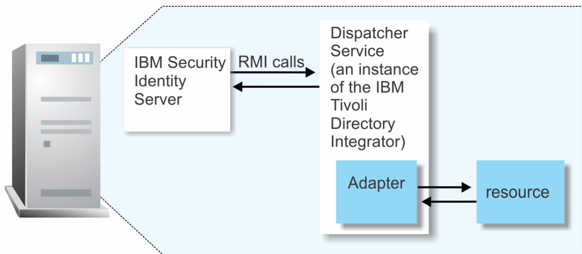
Figure 1. The architecture of the CLIX Adapter
