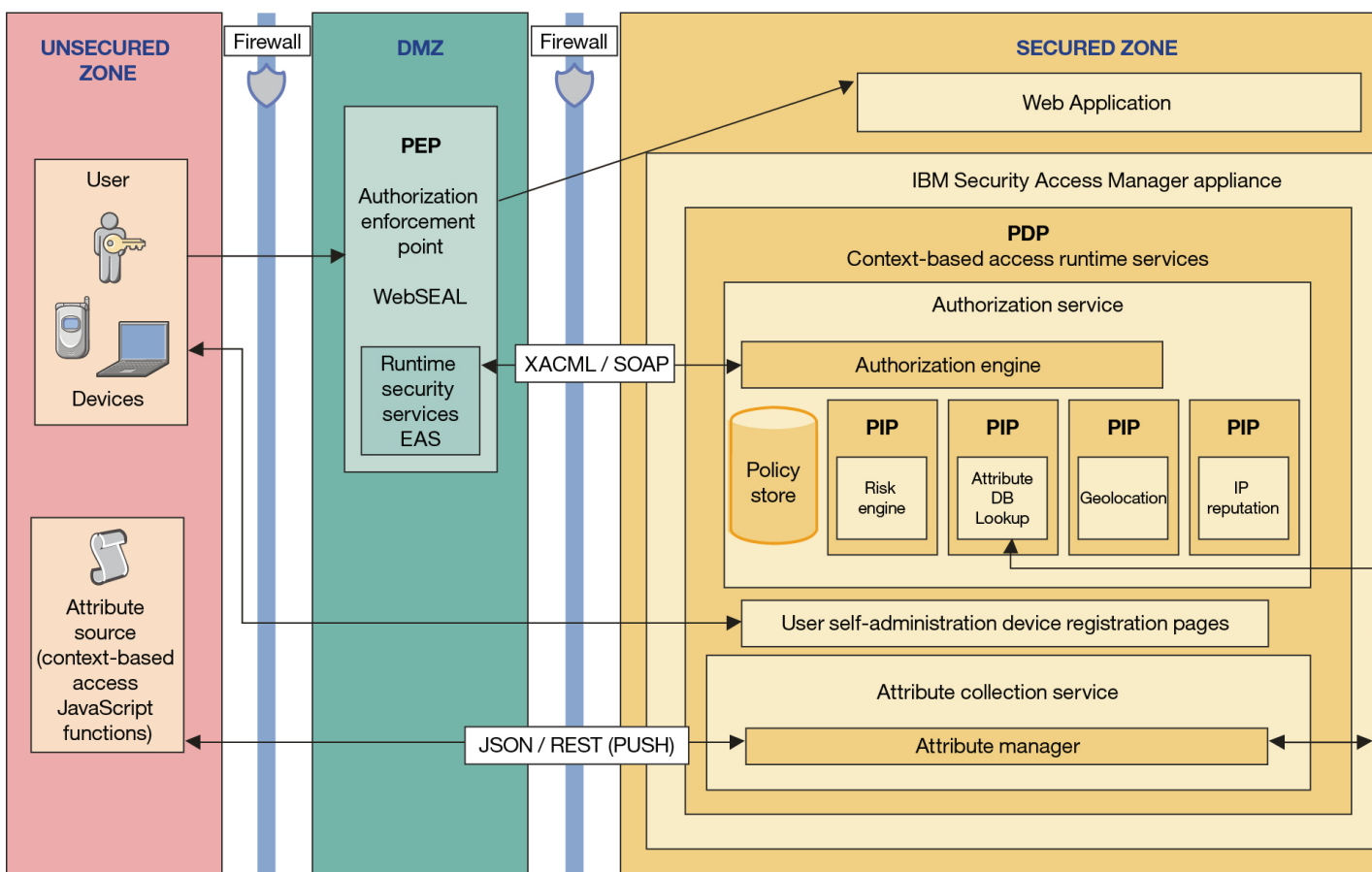
Figure 1. Context-based access architecture
