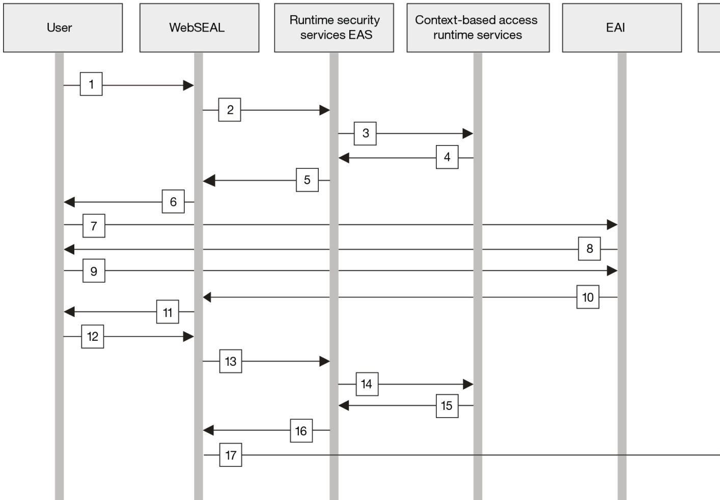
Figure 2. Context-based access transaction flow example
