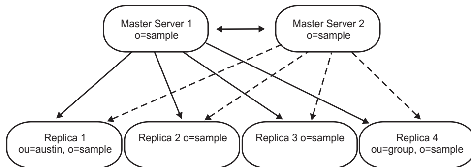
Figure 9. Peer-to-peer replication
