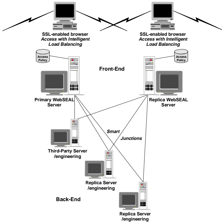
Figure 4. Junctioning of Replicated WebSEAL and Back-end Servers
