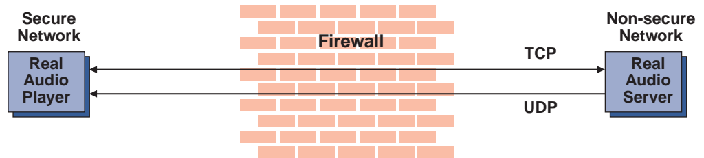
Figure 49. RealAudio Connections through the IBM Firewall. Once a RealAudio TCP connection is detected, the back channel UDP packet from the RealAudio server to the RealAudio player will be permitted to pass through the Firewall as long as the TCP connection is active.
