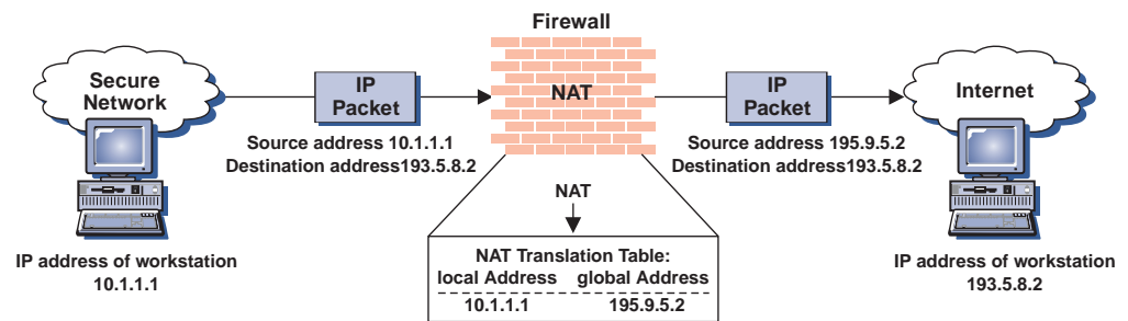
Figure 50. Network Address Translation
