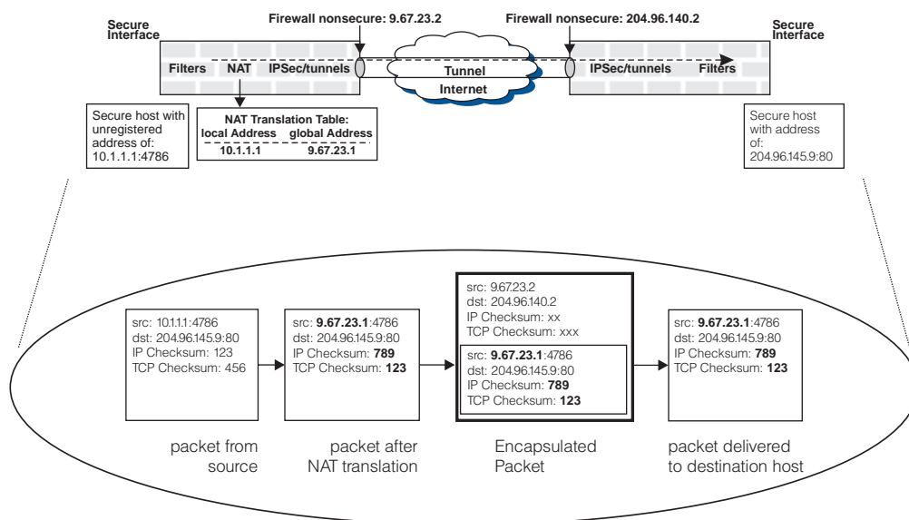
Figure 51. Example Interaction between NAT, Filters and Tunnels
