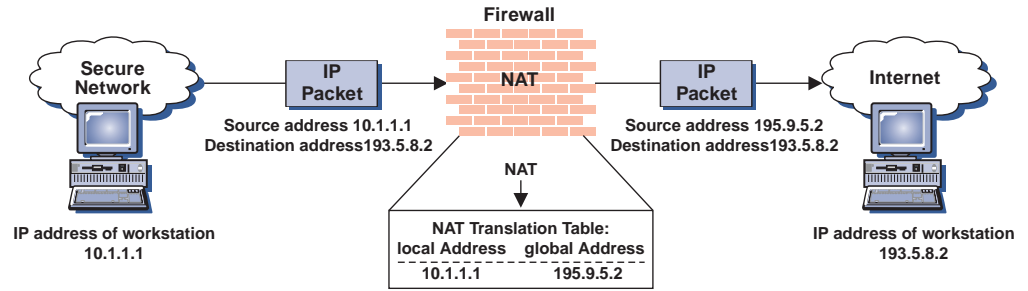
Figure 4. Network Address Translation
