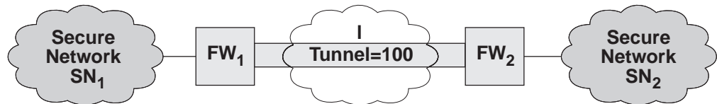
Figure 29. Tunnel, All IP Traffic between Two Secure Networks. FW 1 and FW 2 represent nonsecure interface IP address and mask. SN 1 and SN 2 represent any host in the secure network. The shaded area of the picture represents a VPN.
