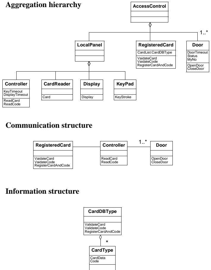
Figure 4: The analysis object model of the Access Control system (basic version)
