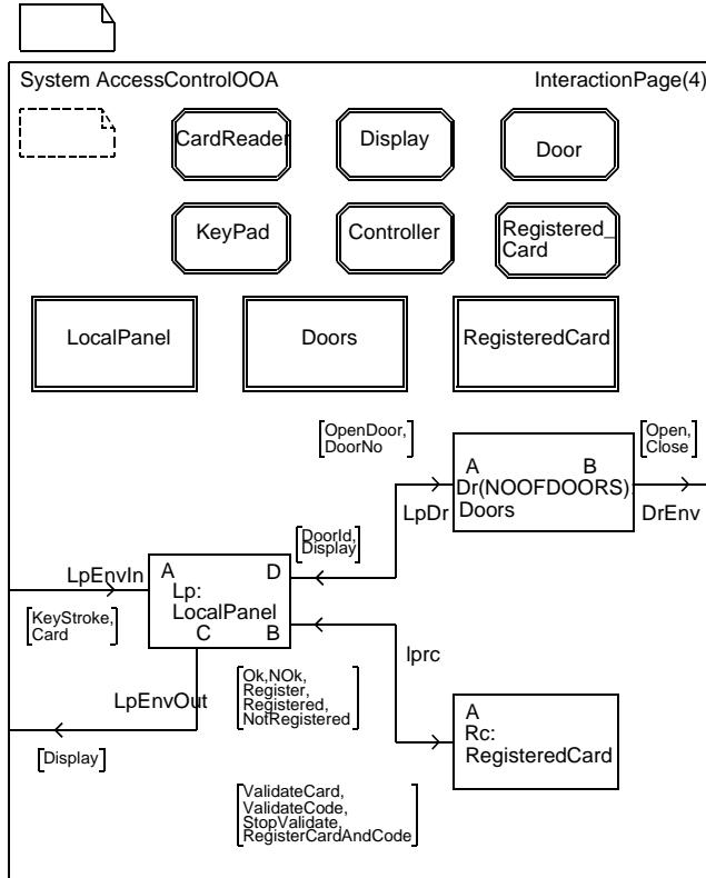
Figure 7: System diagram AccessControlOOA
