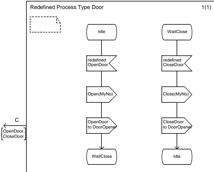
Figure 18: The redefined process type Door
