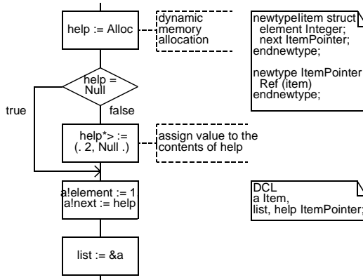
Figure 43: Building a linked list
