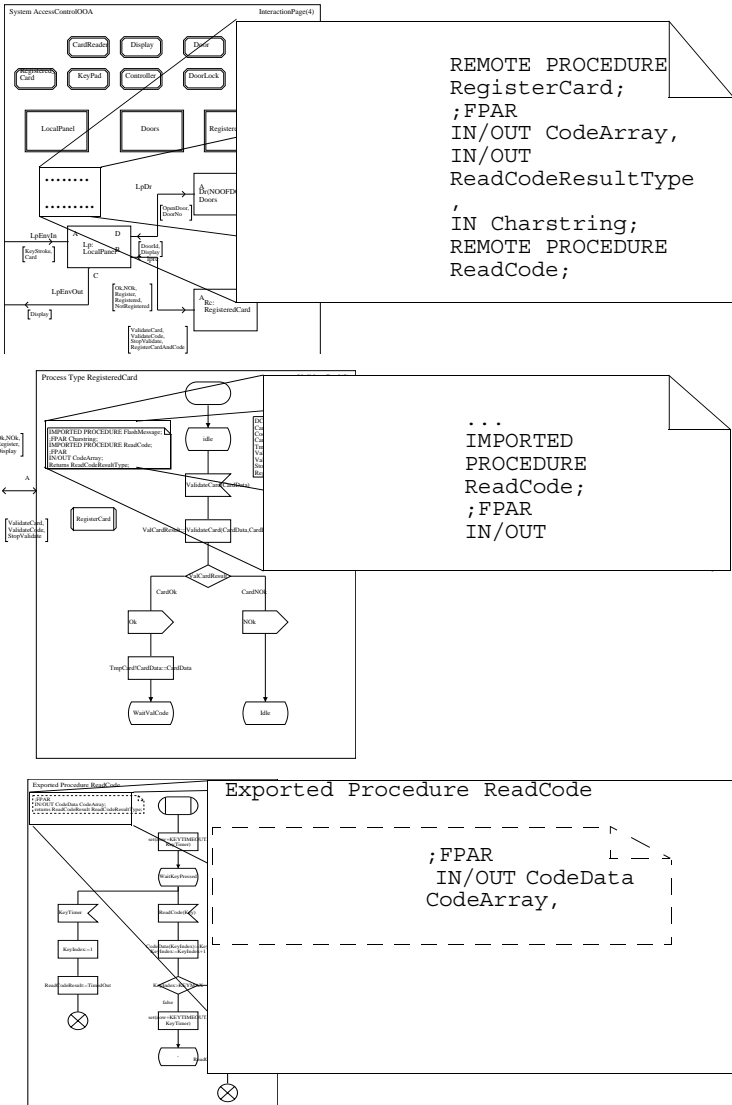
Figure 14: Declaration of a remote procedure
