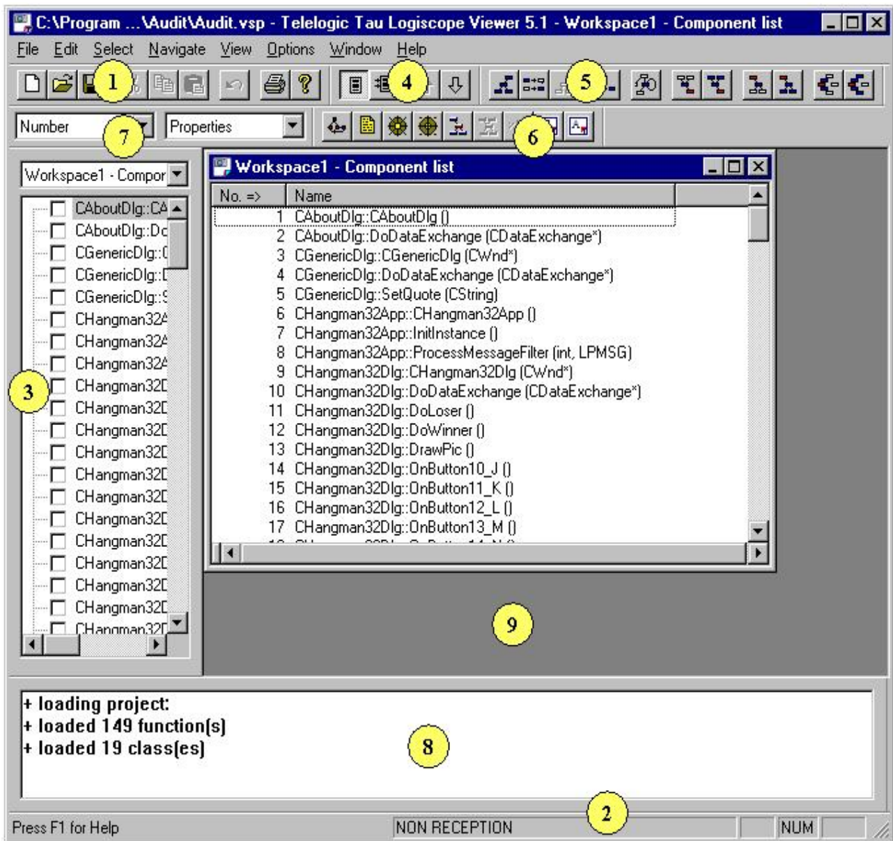
Viewer Main Window
