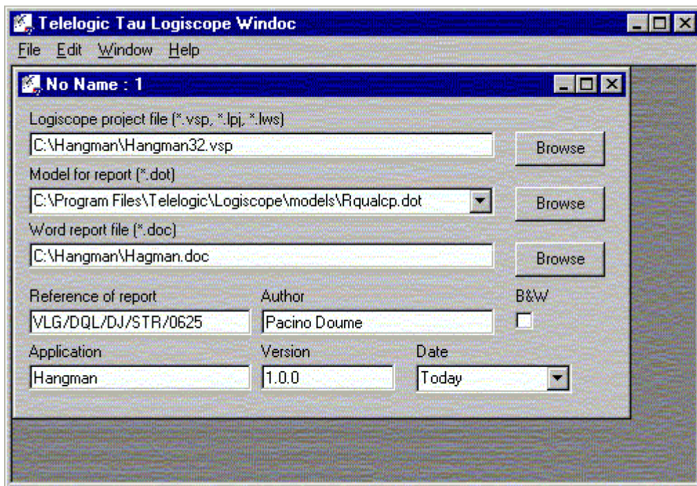
WinDoc Main Window
