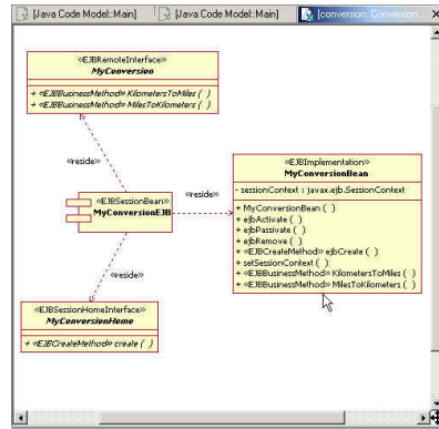
Figure 5: MyConversion EJB
