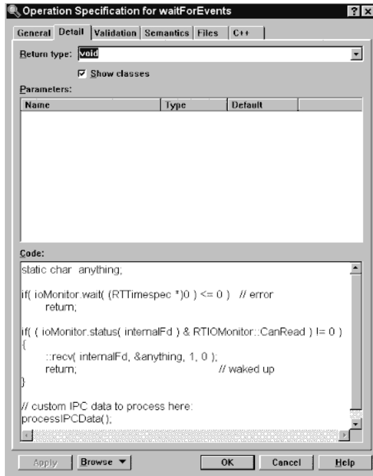
Figure 4. An implementation for the waitForEvents function called when the RTCustomController has no messages left to deliver (TCPClient::waitForEvents).
