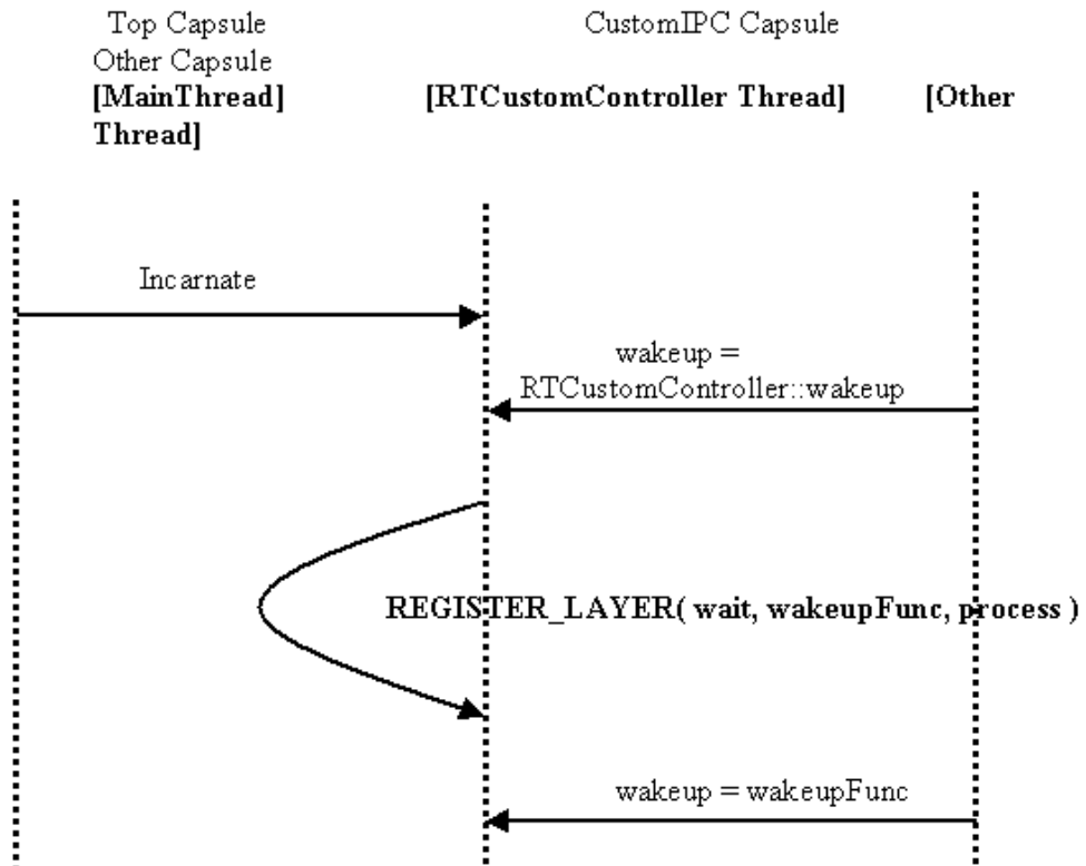
Figure 6: Wakeup control flow of inter-thread message send involving RTCustomController .
