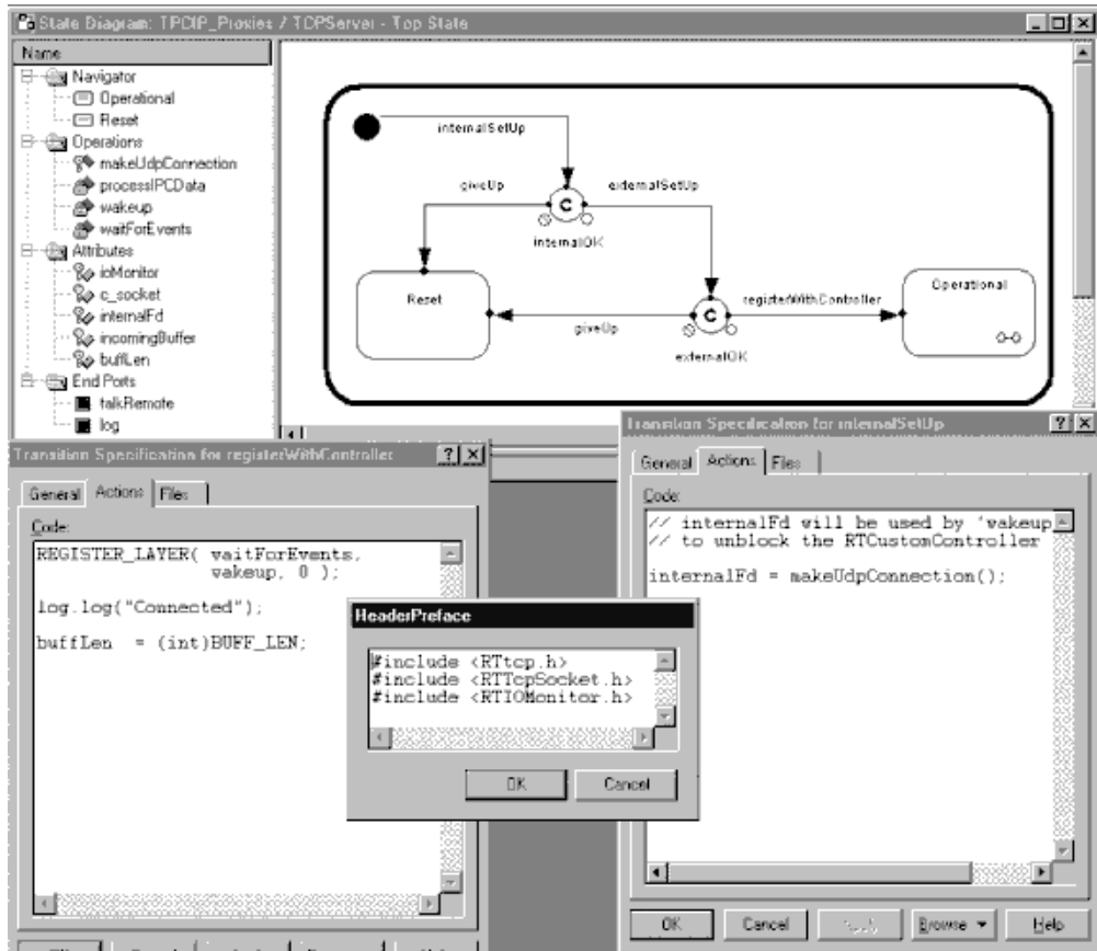
Figure 3. Behavior of a capsule monitoring a TCP/IP socket connection
