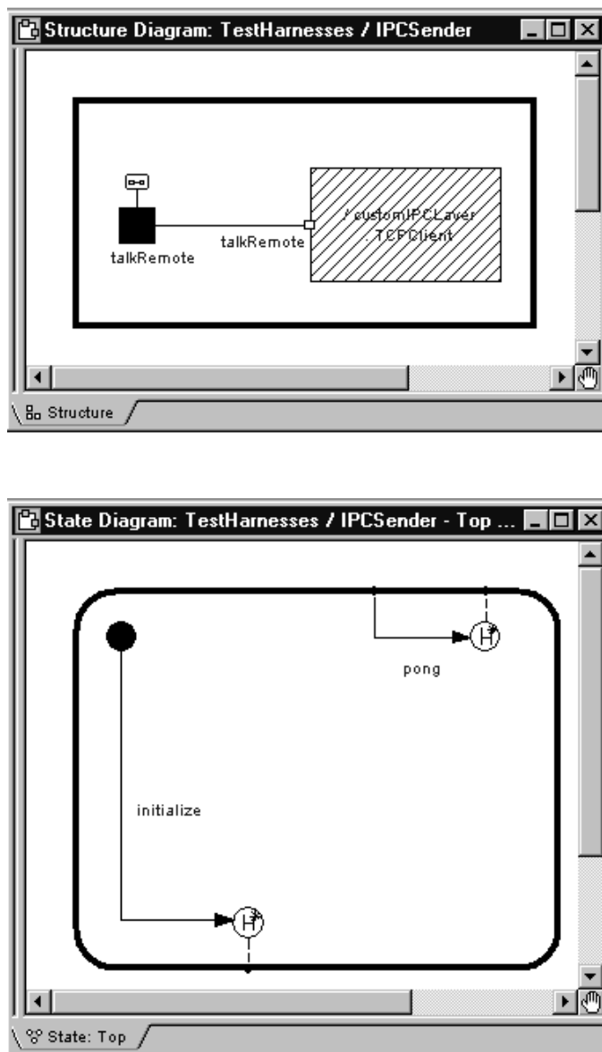
Figure 1-2. The IPCSender incarnates an IPC monitoring capsule on the RTCustomeController thread.
