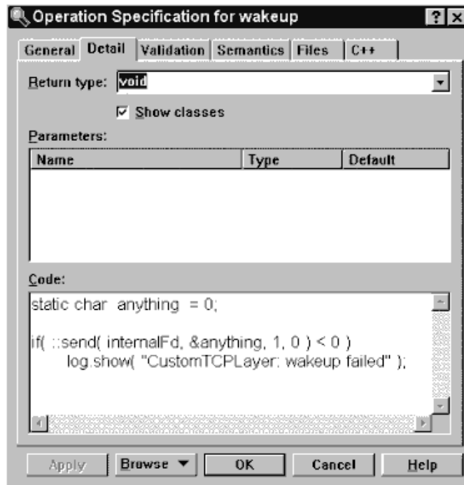
Figure 5. An implementation for the wakeup function called when the RTCustomController receives an inter-thread message (TCPClient::wakeUp).
