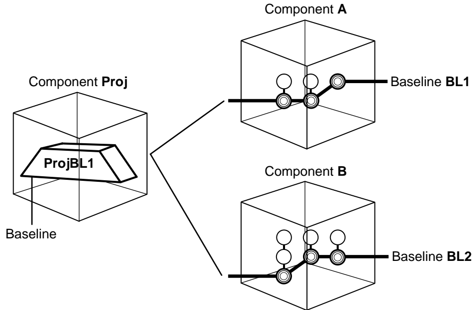
Figure 8 Composite Baseline
