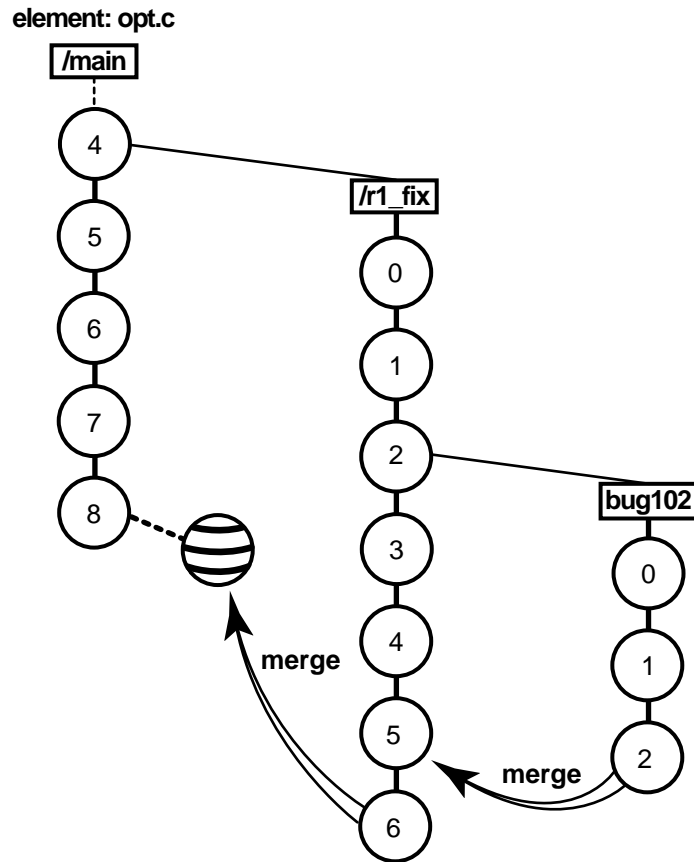
Figure 19 Merging Branches
