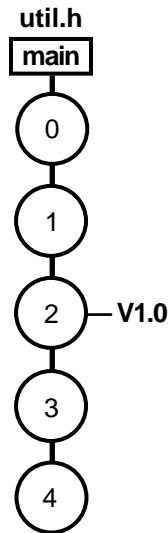
Figure 14 Version Label
