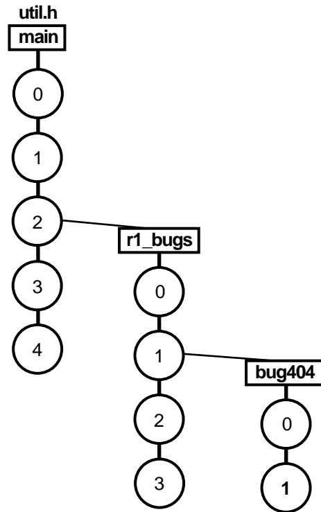
Figure 13 Branches
