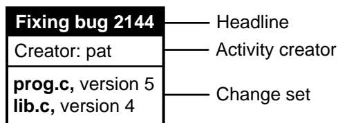
Figure 5 An Activity
