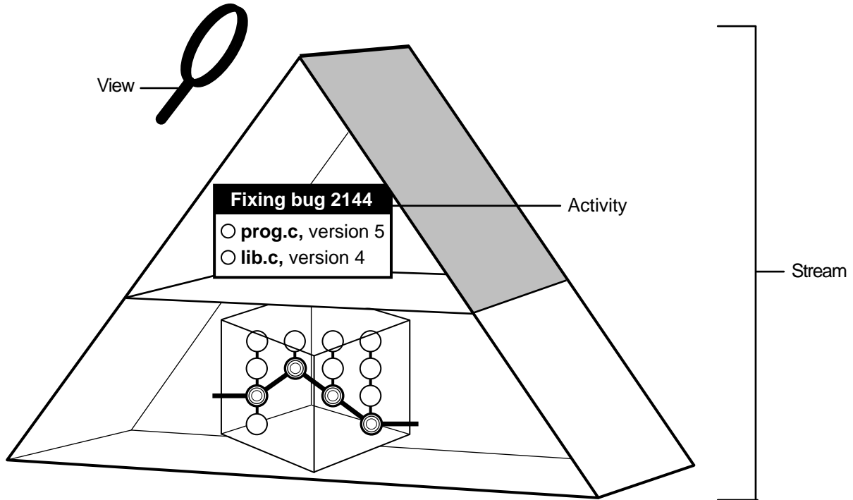
Figure 6 A Stream
