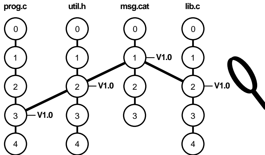
Figure 16 Selecting Versions Included in a Particular Release
