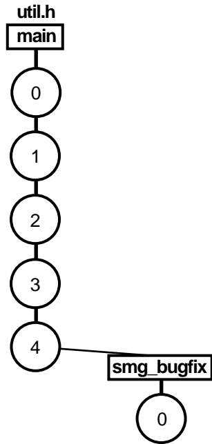
Figure 18 Working on a Private Branch
