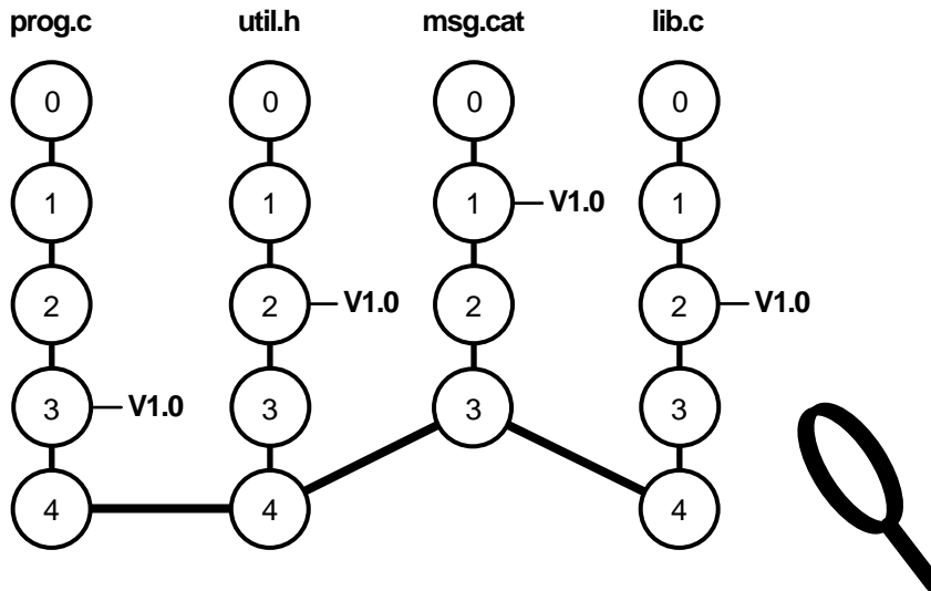
Figure 15 Selecting Versions Used in Development Work
