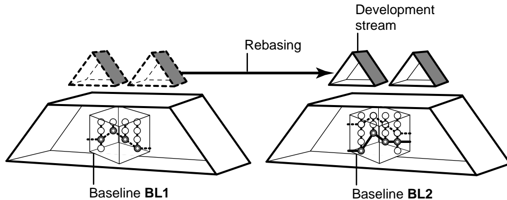
Figure 12 Rebasing the Development Stream
