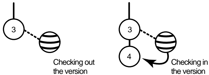
Figure 3 Using the Check Out/Check In Model
