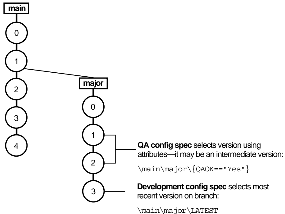
Figure 39 Development Config Spec vs. QA Config Spec
