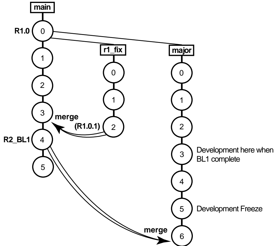
Figure 53 Merging Baseline 1 Changes into the major Branch
