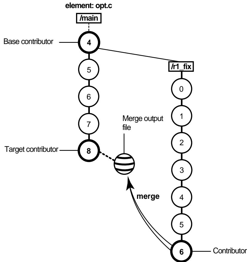
Figure 42 Versions Involved in a Typical Merge
