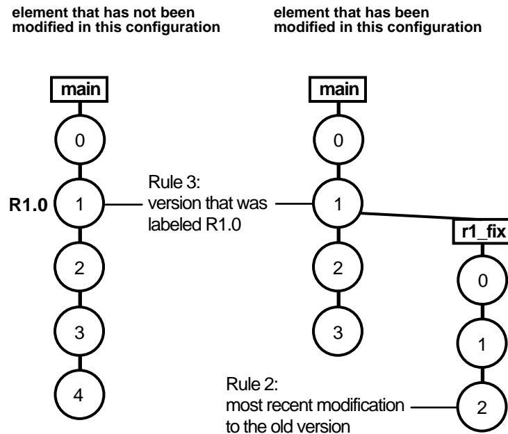
Figure 37 Making a Change to an Old Version
