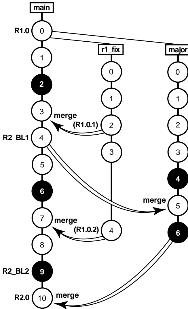
Figure 50 Development Milestones: Evolution of a Typical Element
