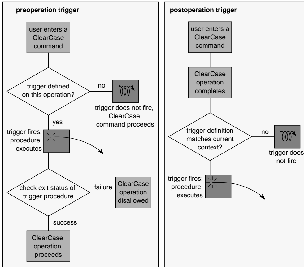
Figure 34 Preoperation and Postoperation Triggers
