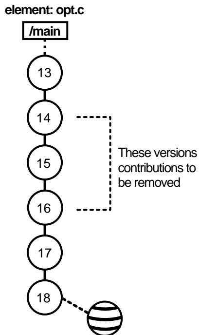
Figure 45 Removing the Contributions of Some Versions
