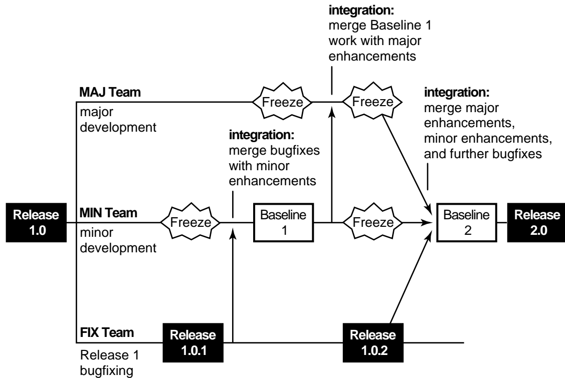
Figure 49 Project Plan for Release 2.0 Development
