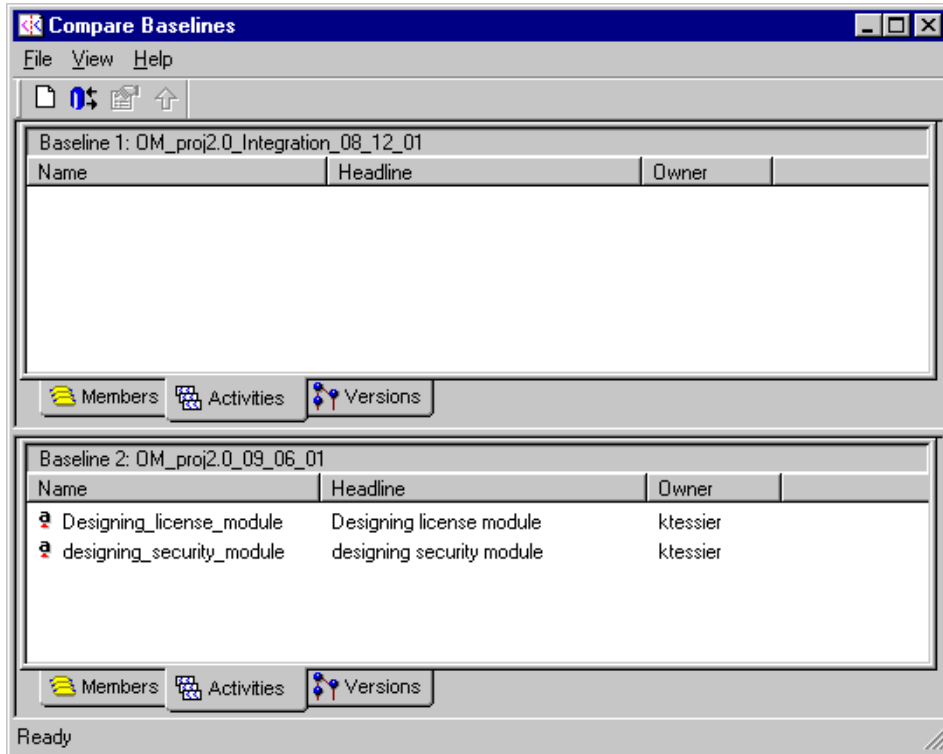
Figure 33 Comparing Baselines by Activity
