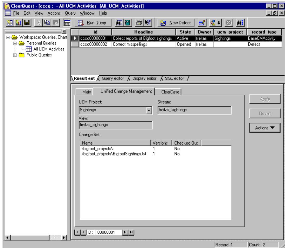
Figure 57 Change Sets in ClearQuest GUI
