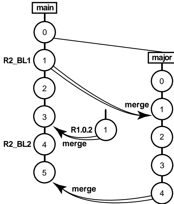
Figure 55 Element Structure After the Pre-Baseline-2 Merge
