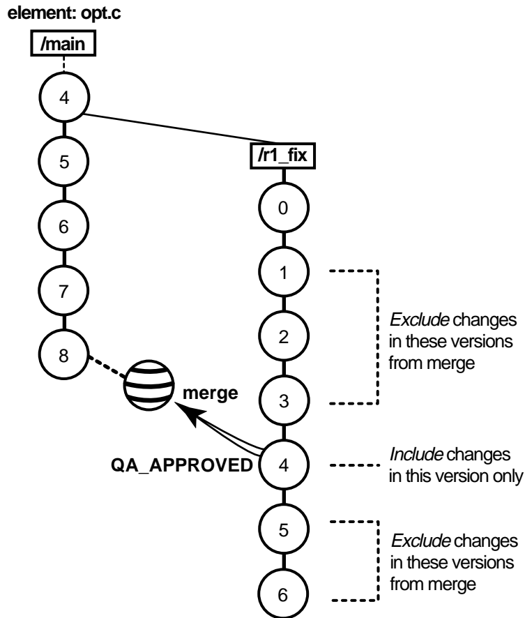
Figure 44 Selective Merge from a Subbranch
