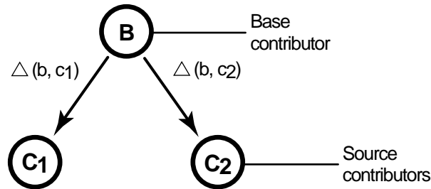
Figure 43 ClearCase Merge Algorithm
