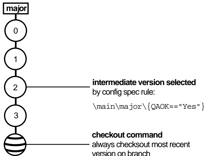
Figure 40 Checking Out a Branch of an Element
