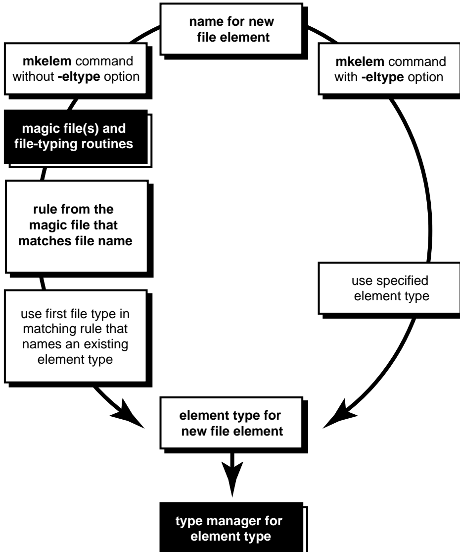
Figure 47 Data Handling: File Type, Element Type, Type Manager
