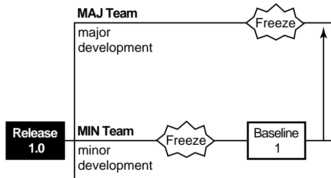
Figure 52 Updating Major Enhancements Development
