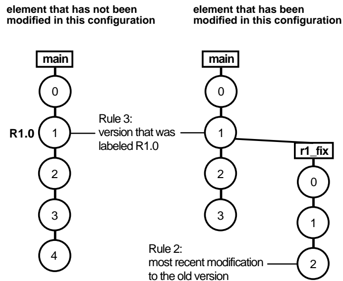
Figure 34 Making a Change to an Old Version
