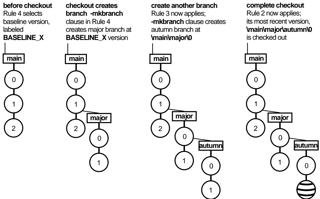
Figure 35 Multiple-Level Auto-Make-Branch
