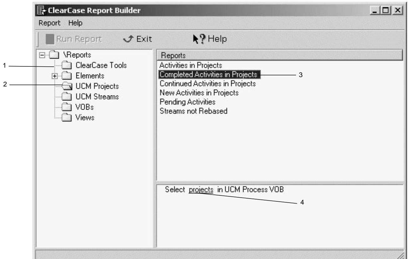
Figure 54 Customizable Areas of Report Builder Interface
