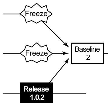
Figure 50 Baseline 2
