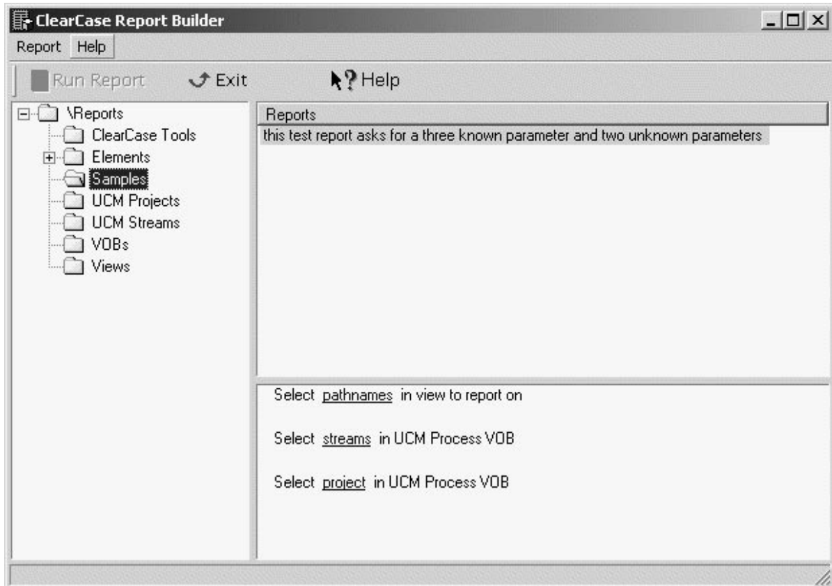
Figure 59 Report Builder Window with Invalid Parameters
