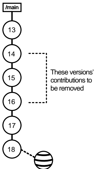
Figure 42 Removing the Contributions of Some Versions
