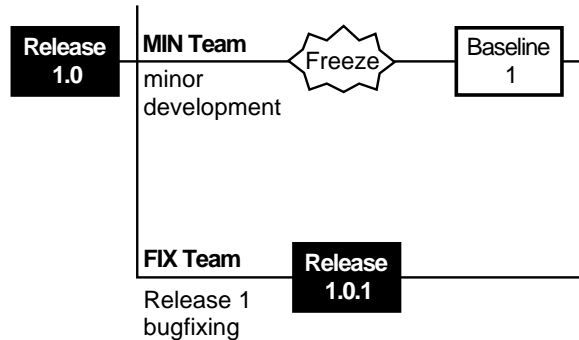
Figure 47 Creating Baseline 1
