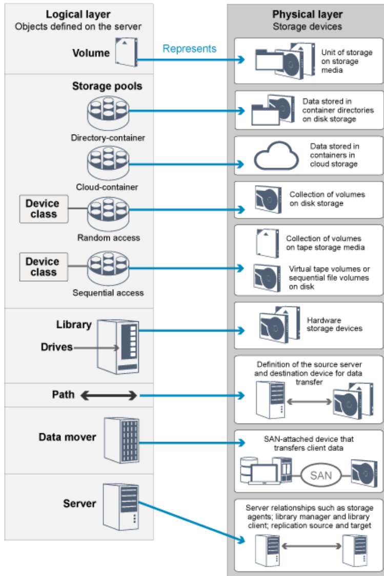
Figure 1. Storage objects
