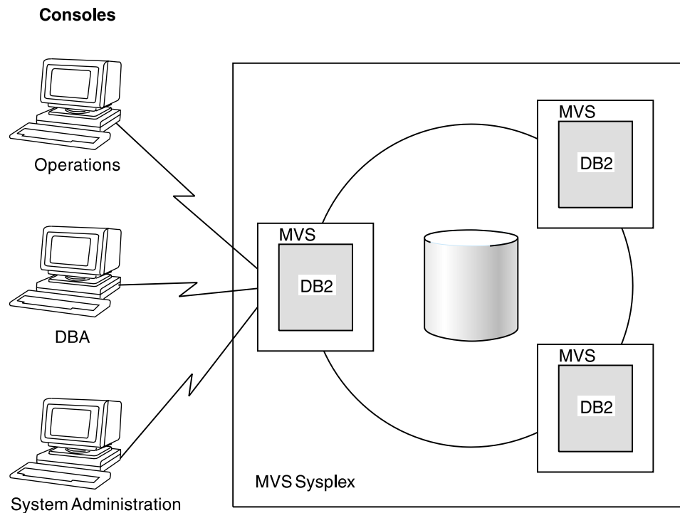
Figure 19. Issuing Commands
