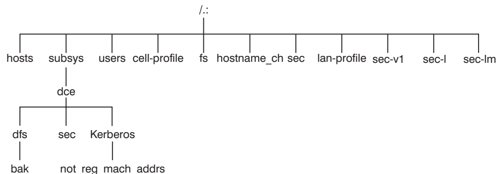
Figure 3. The Top-Level CDS Directory
