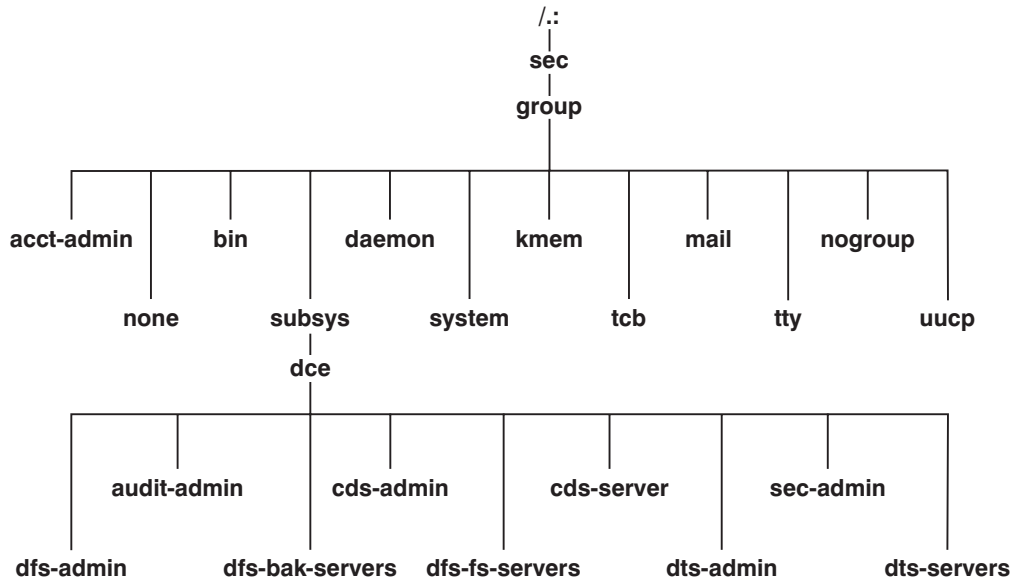
Figure 6. The sec/group Directory
