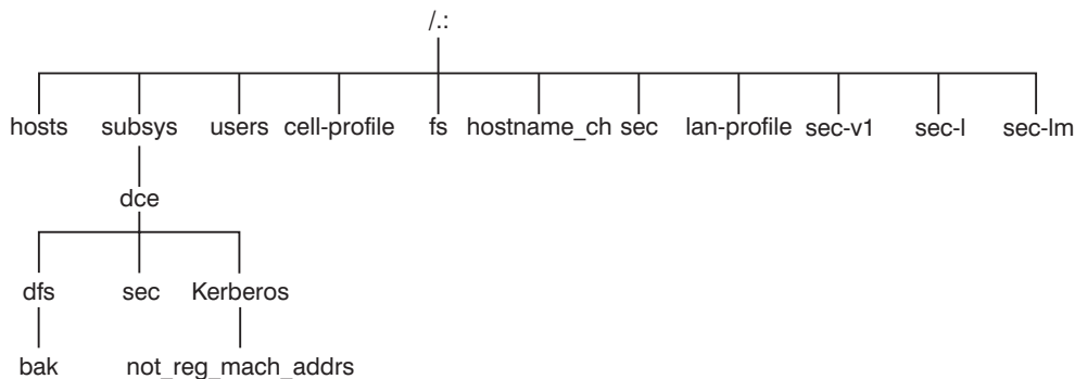
Figure 2. Top Level of the Cell Namespace
