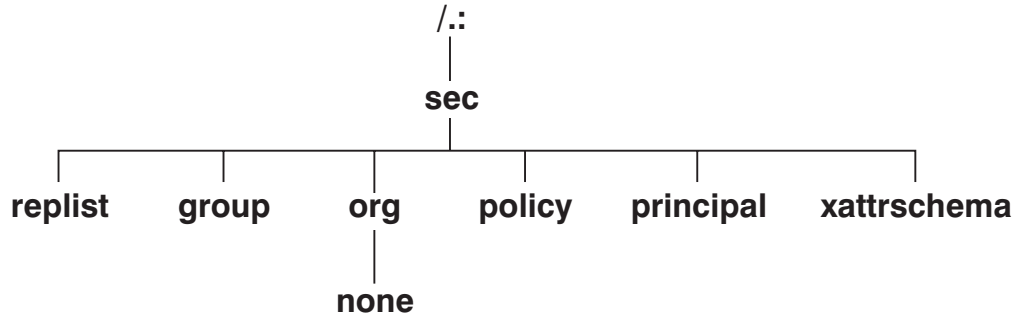
Figure 5. The Top-Level Security Directory
