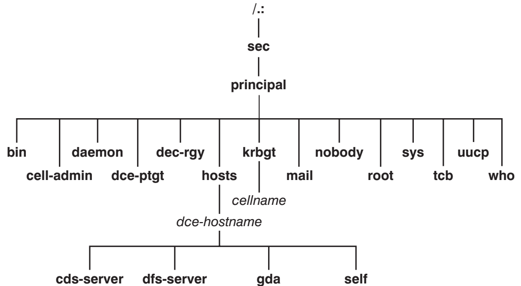
Figure 7. The sec/principal Directory
