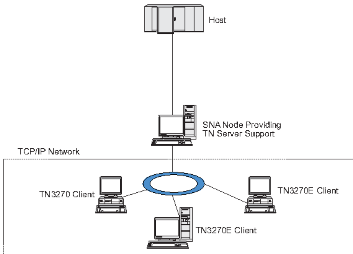
Figure 10. CS/AIX Node Configured for TN Server
