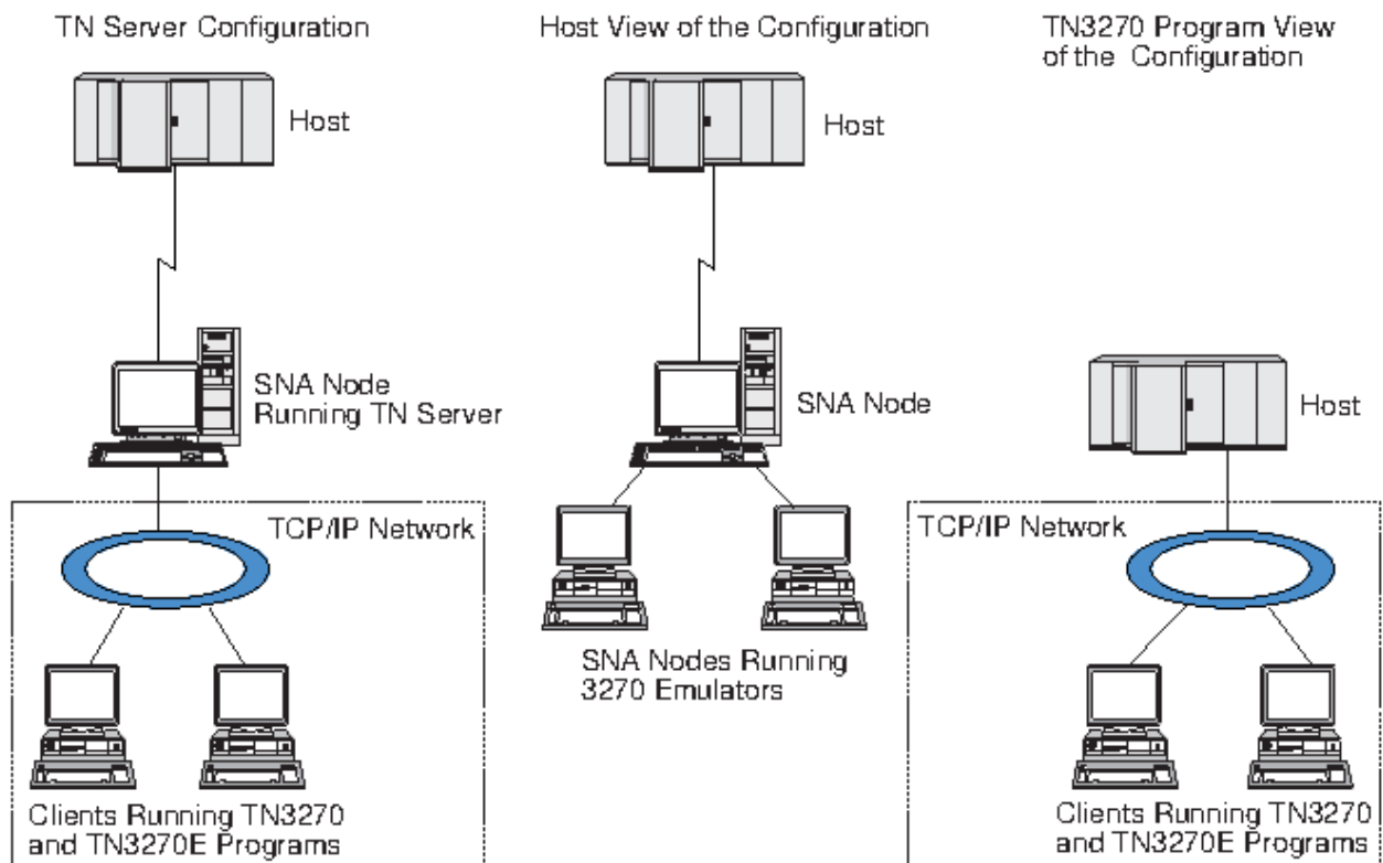
Figure 11. TN Server
