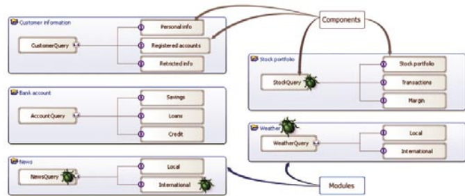
Figure 18. Integration debugger
