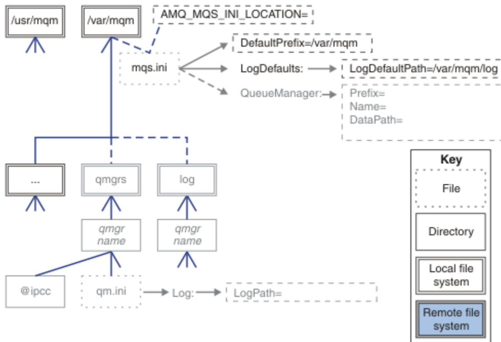
Figure 36. Directory structure pattern template
